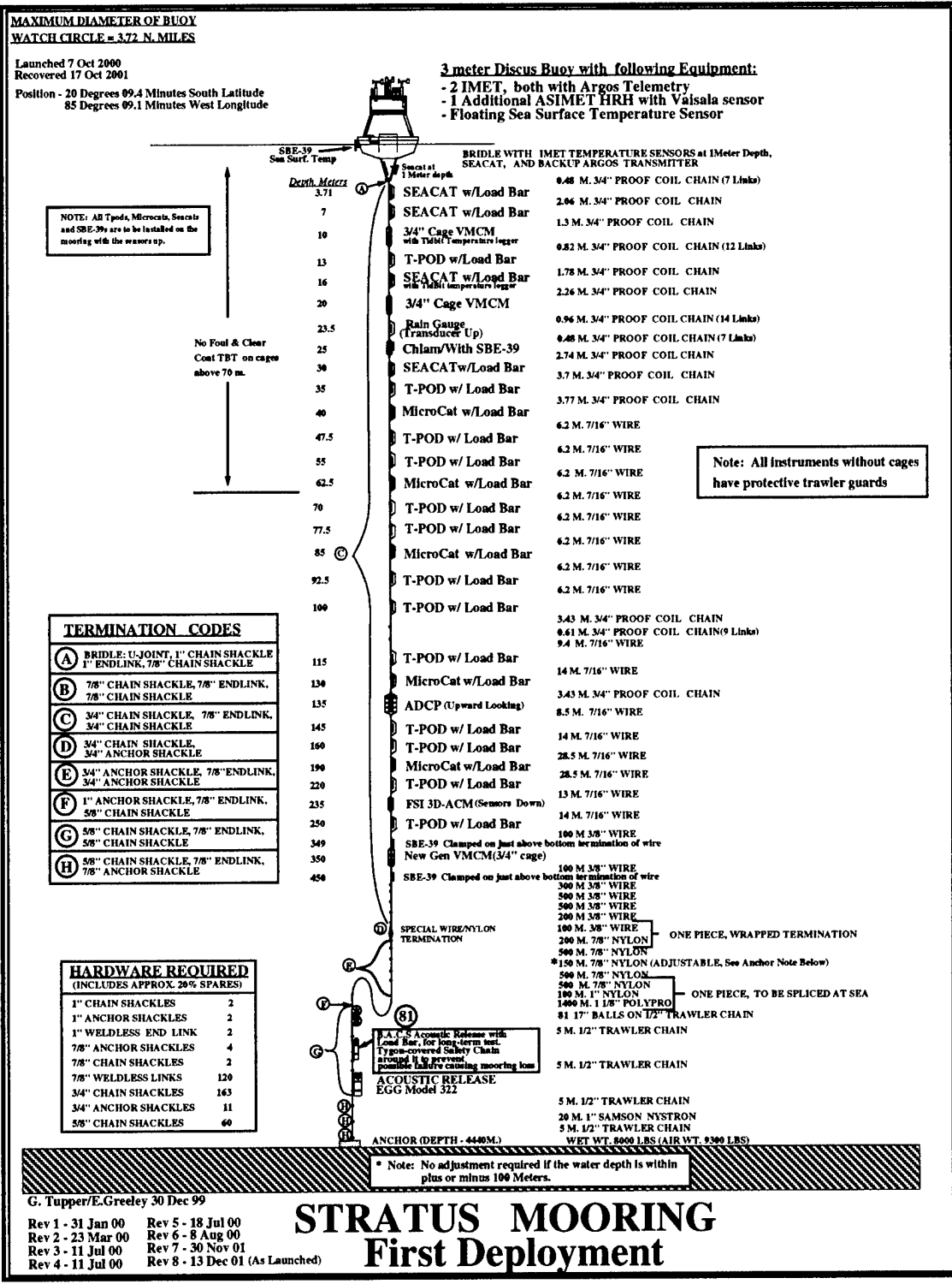
Figure 31 : Stratus 1 mooring diagram – recovery.
