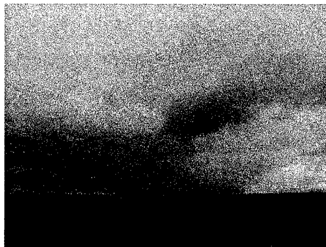
Figure 25: Cloud photo looking eastward at about 11:15 UTC on October 21 (Day 294).
