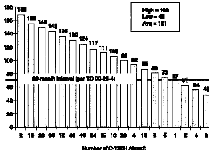
Figure 3. Proposed PDM Intervals (in months) versus Number of C-130H Aircraft
