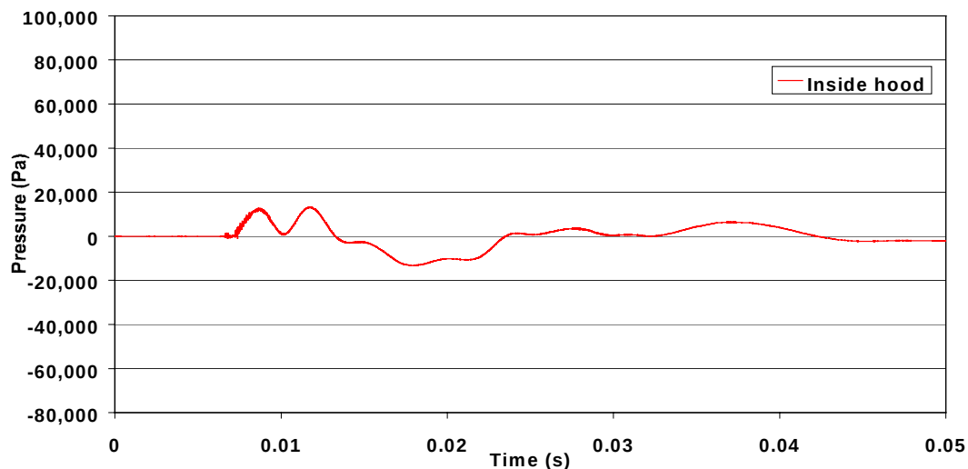
Figure 2-5. The time history of a typical acoustic pressure wave measured inside of a diver's foam neoprene diving hood whilst operating an underwater bolt gun into a concrete block (Parvin, 1999).
