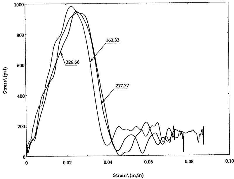
Figure 12.16a. Stress-Strain Curve for Nomex Honeycomb Core With Hybrid Facesheets (With MTG) – Glass/Epoxy Facesheet Facing
