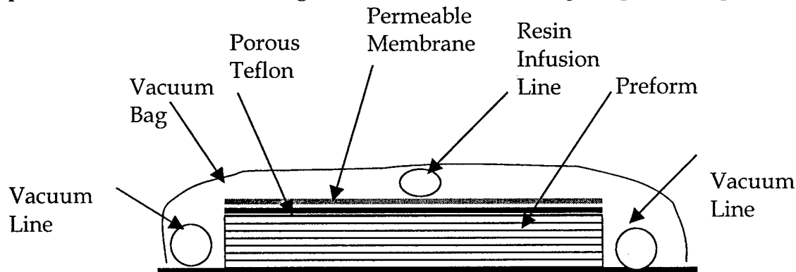
Figure 1.9 Vacuum Assisted Resin Infusion / Transfer Molding (VARIM/VARTM)
