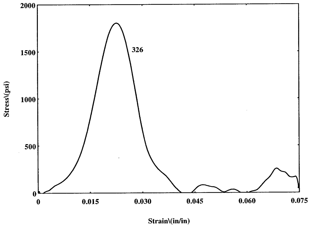
Figure 12.3c. Stress-Strain Curve Obtained from the Above Signal (Honeycomb Core Sandwich Composite)
