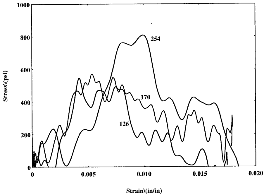
Figure 12.11a. Stress-Strain Curve for Foam+Honeycomb Core Sandwich Composite (1.5" Bar)
