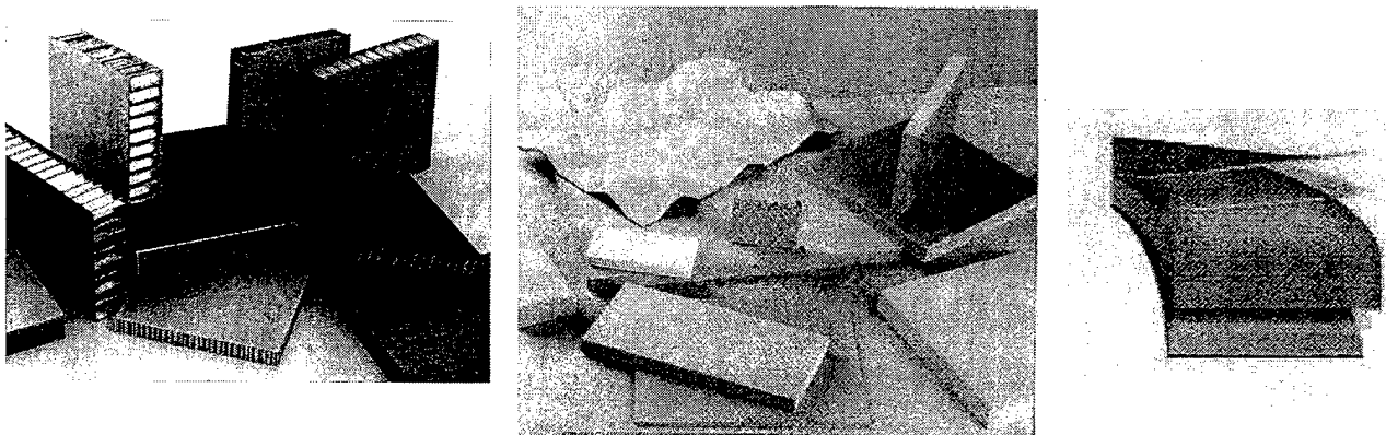
Figure 4.2 Commonly used Honeycomb and Foam Cores and their Sandwich Constructions
