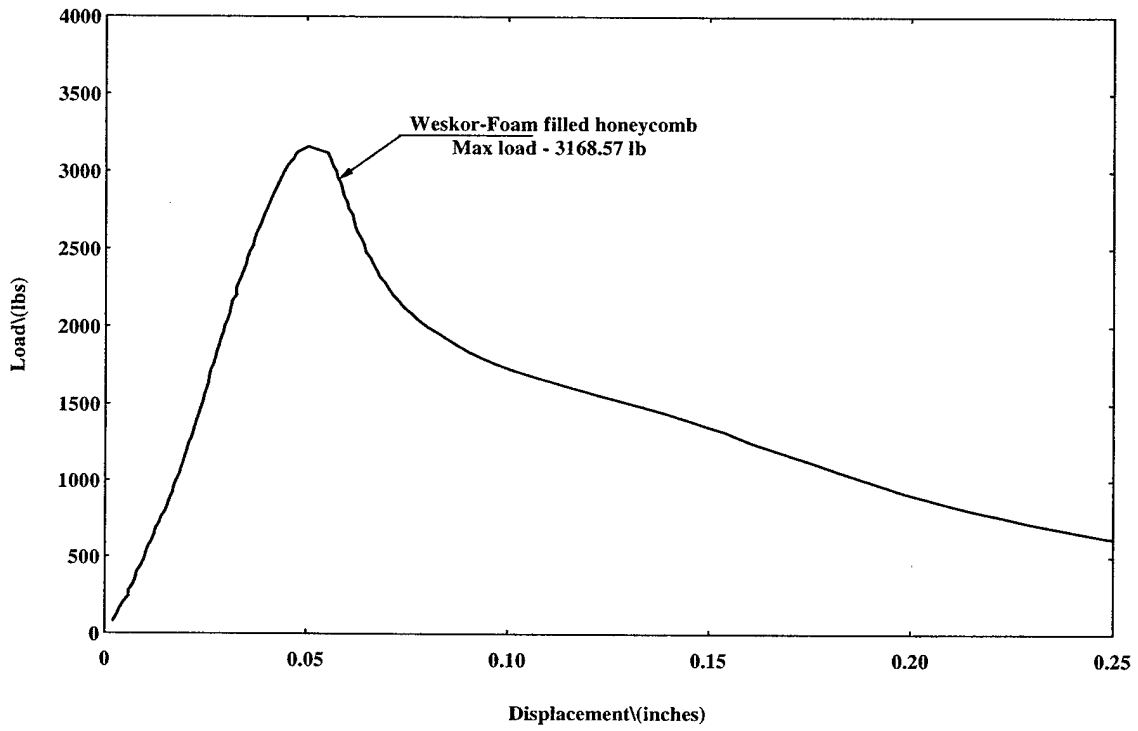
Figure 11.20. In-plane Shear Load-Displacement Curves for WESKOR Foam Filled Honeycomb Core Sandwich Composite
