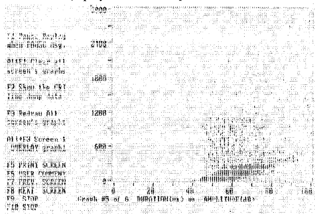
Figure 11.12. AE Response in terms of Duration vs Amplitude for Graphite/Epoxy Truss Core Composite
