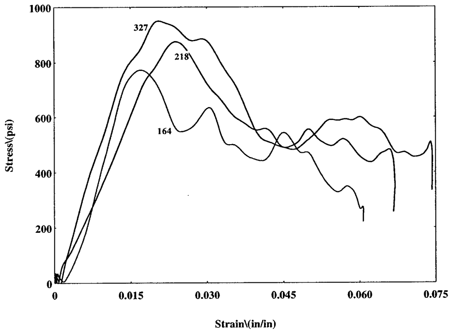
Figure 12.7a. Stress-Strain Curve for Foam + Titanium Pins With MTG
