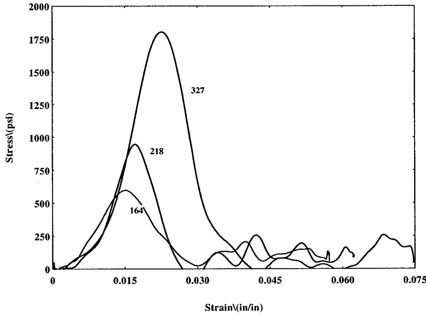
Figure 12.6a. Stress-Strain Curve for Honeycomb Core Sandwich Composite With MTG
