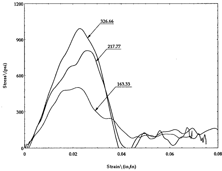
Figure 12.17a. Stress-Strain Curve for Nomex Honeycomb Core With Hybrid Facesheets (With MTG) – Graphite/Epoxy Facesheet Facing
