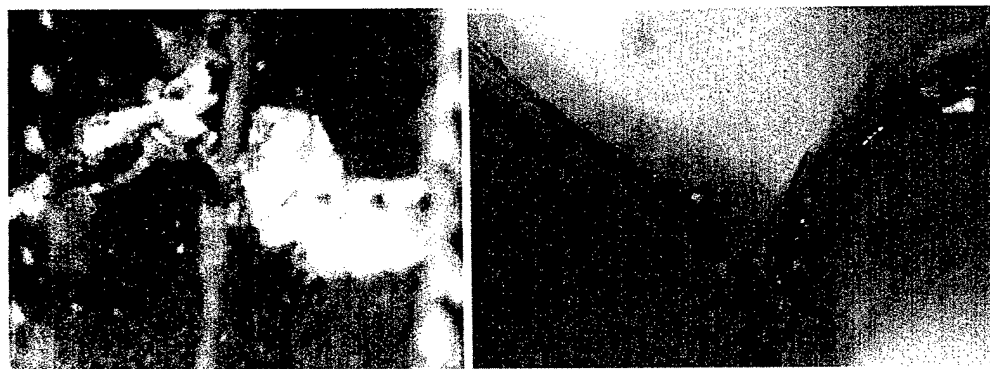
(a) (b) Figure 11.23a-b. Edge View and Top View of Honeycomb Core Cells Failed Under Static Compression
