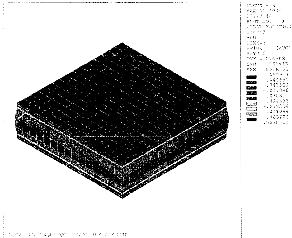
Figure 14.22. Total Strain in the z-Direction for the foam Core Sandwich Panel Under Transverse Compression.
