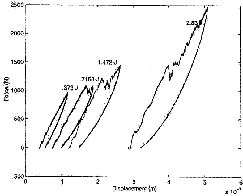
Figure 10.7 Load-Displacement Curves for five 20 Degree orientation Specimens Tested at Different Energy Levels
