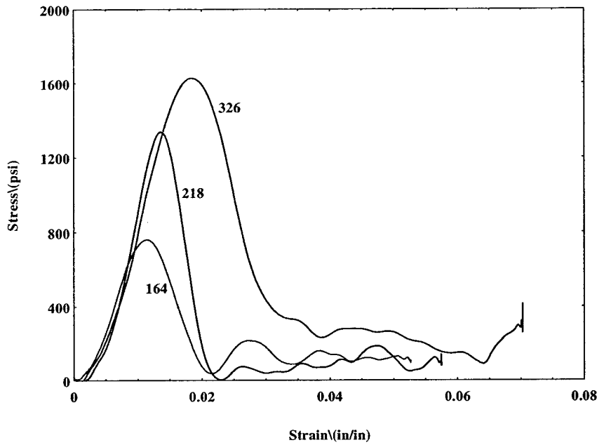
Figure 12.10a. Stress-Strain Curve for Foam+Honeycomb Core Sandwich Composite With MTG
