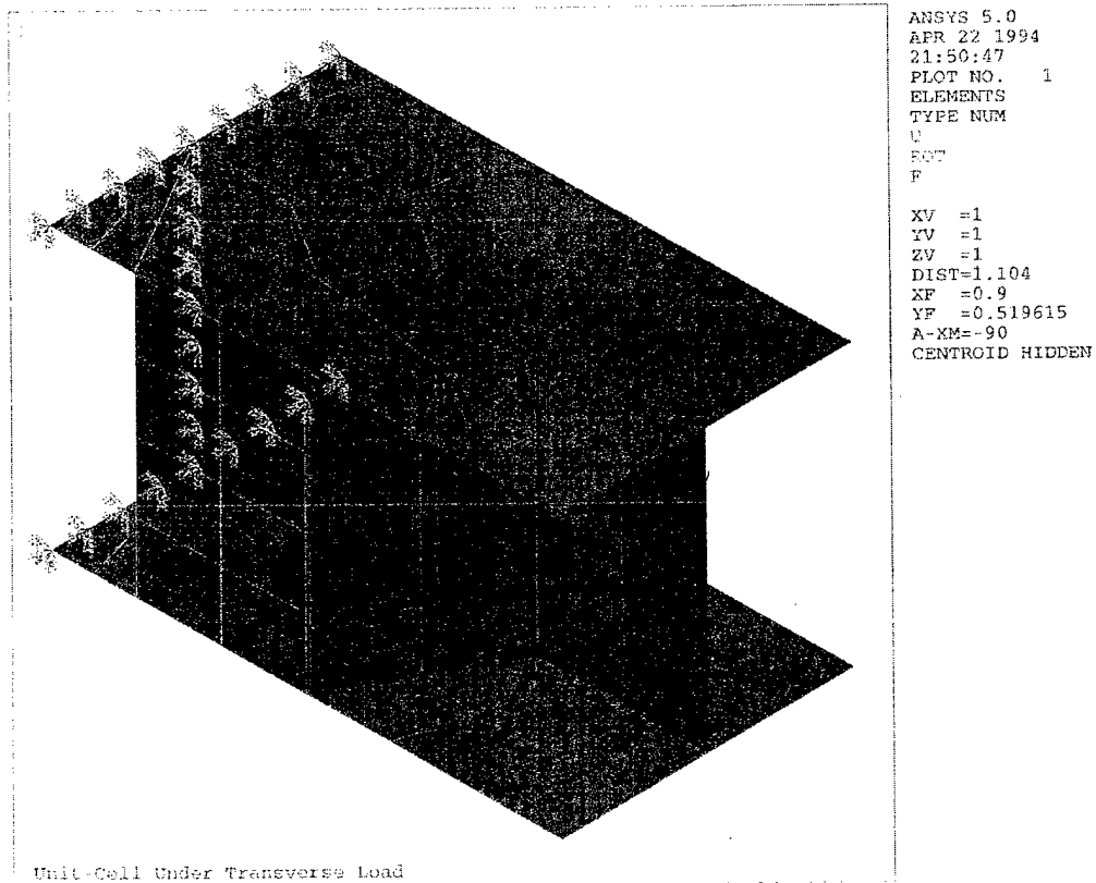
Figure 14.10. Unit Cell Honeycomb with Facesheets Under Constraints for Compression
