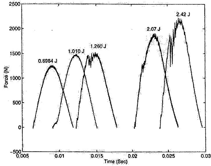
Figure 10.3 Force-Time Curves for five 10 Degree orientation Specimens Tested at Different Energy Levels
