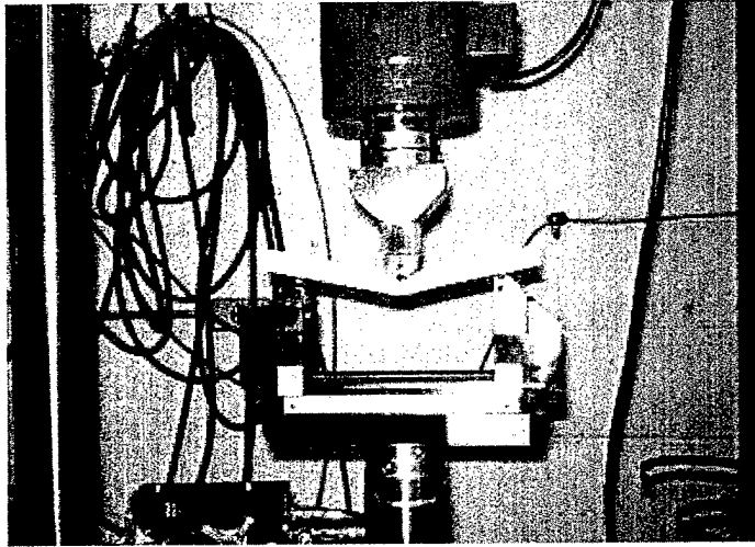
Figure 11.1a Illustration of Static Flexural Testing of Sandwich Composites
