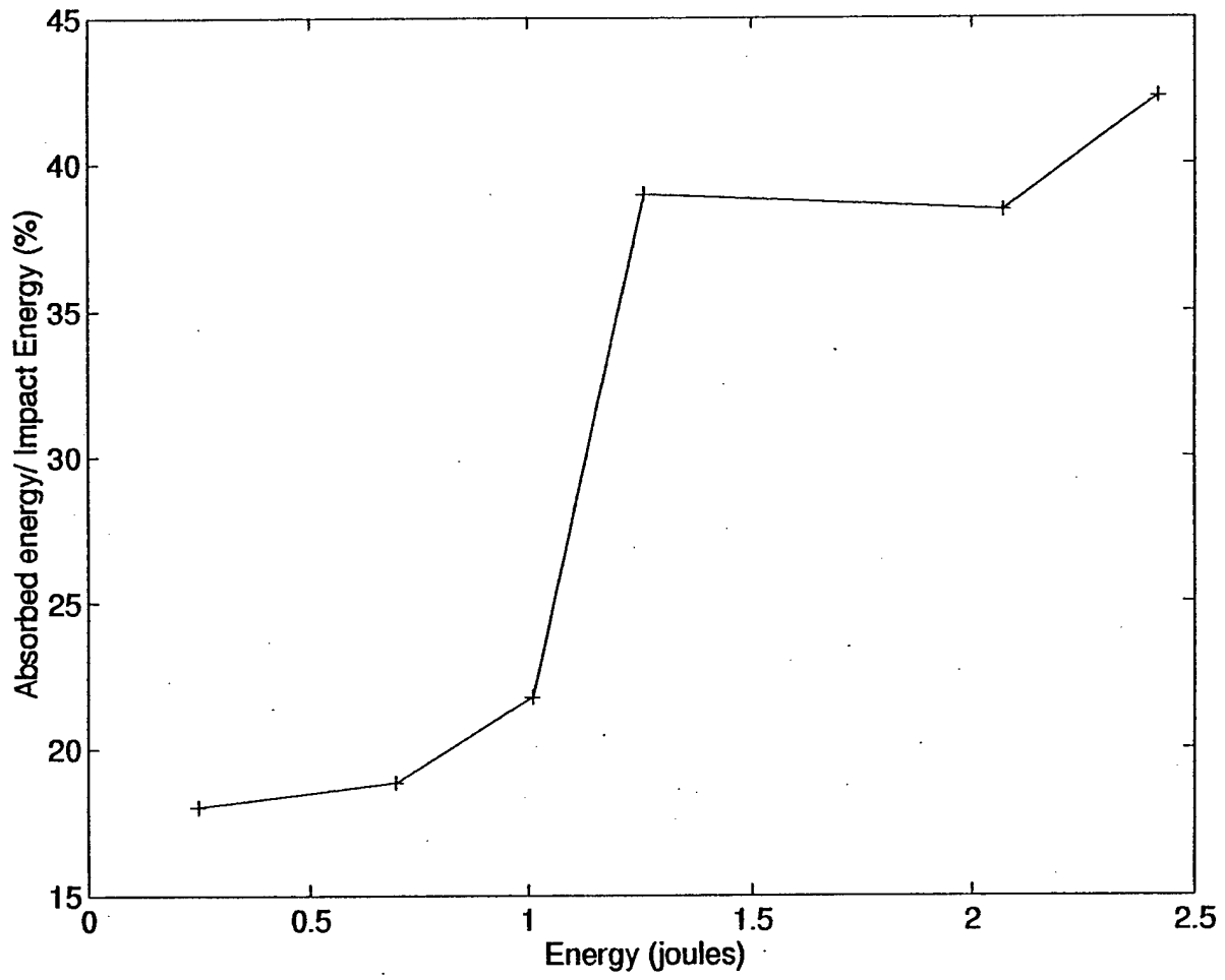
Figure 10.5 Percentage absorbed impact energy vs energy plot
