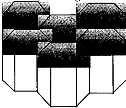
Figure 4.3a Schematic of Honeycomb-Filled-Foam Core
