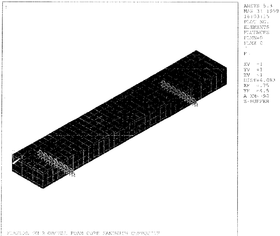
Figure 14.27. Loading and Constrains of Foam Core Sandwich Panel Under Flexure
