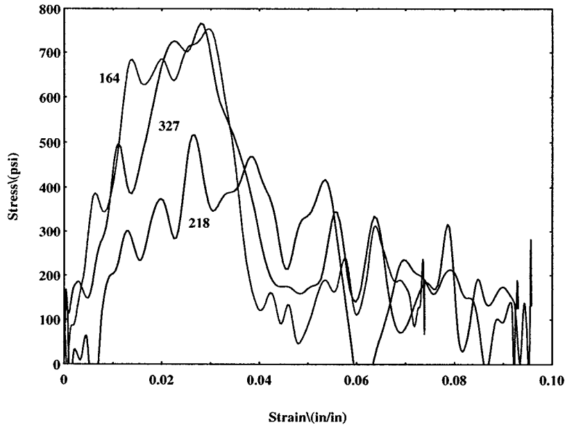
Figure 12.9a. Stress-Strain Curve for Hollow Steel Pin Truss Core Sandwich Composite With MTG
