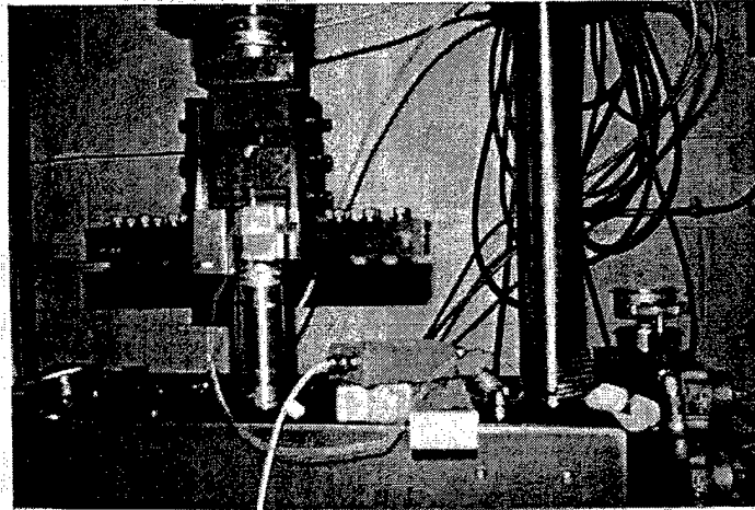
Figure 9.2a,b Photograph of the CAI Testing using MTS
