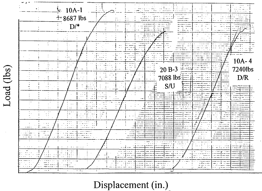
Figure 10.19. CAI Load-Displacement curves (Hollow Z-Pins Steel Core)
