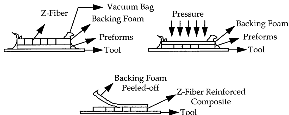
Fig. 3.1 Schematic of Z-Fiber Reinforcement of Composites
