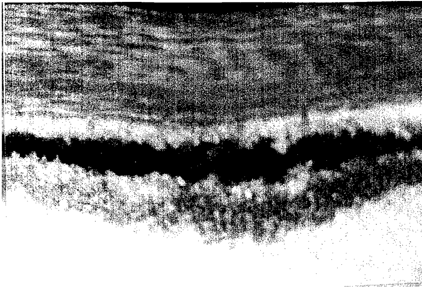
Figure 8.31. Failure of RTM Foam Core Composite. Illustration of Core Crushing Identical to that Observed in the VACM Produced Foam Core Samples
