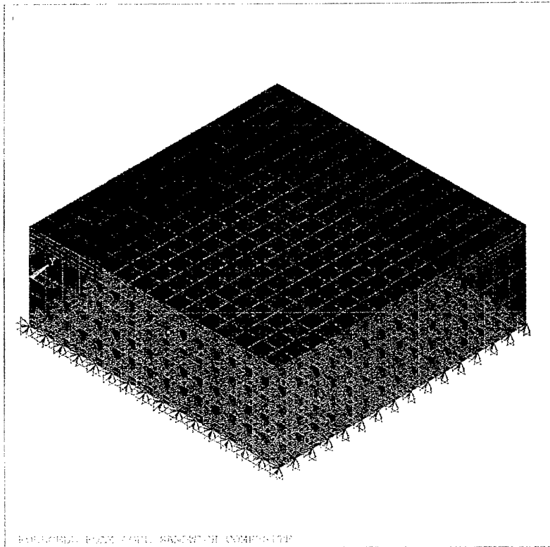
Figure 14.18. Foam Core Sandwich Panel With Constraints.
