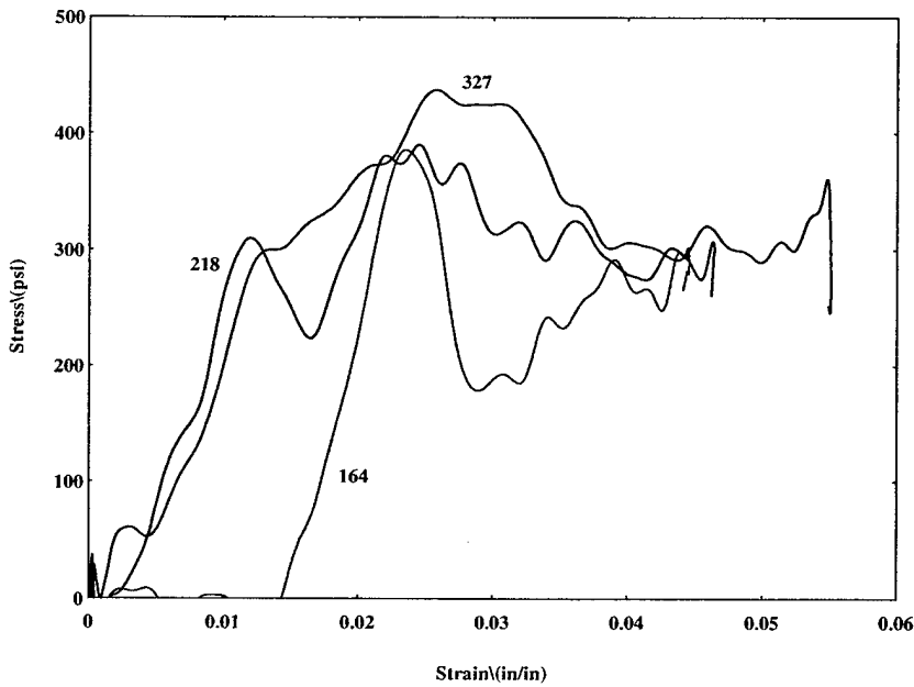
Figure 12.5b. Stress-Strain Curve for Foam Core Sandwich Composite Without MTG
