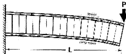
Figure 2.2a. Cantilever Sandwich Beam
