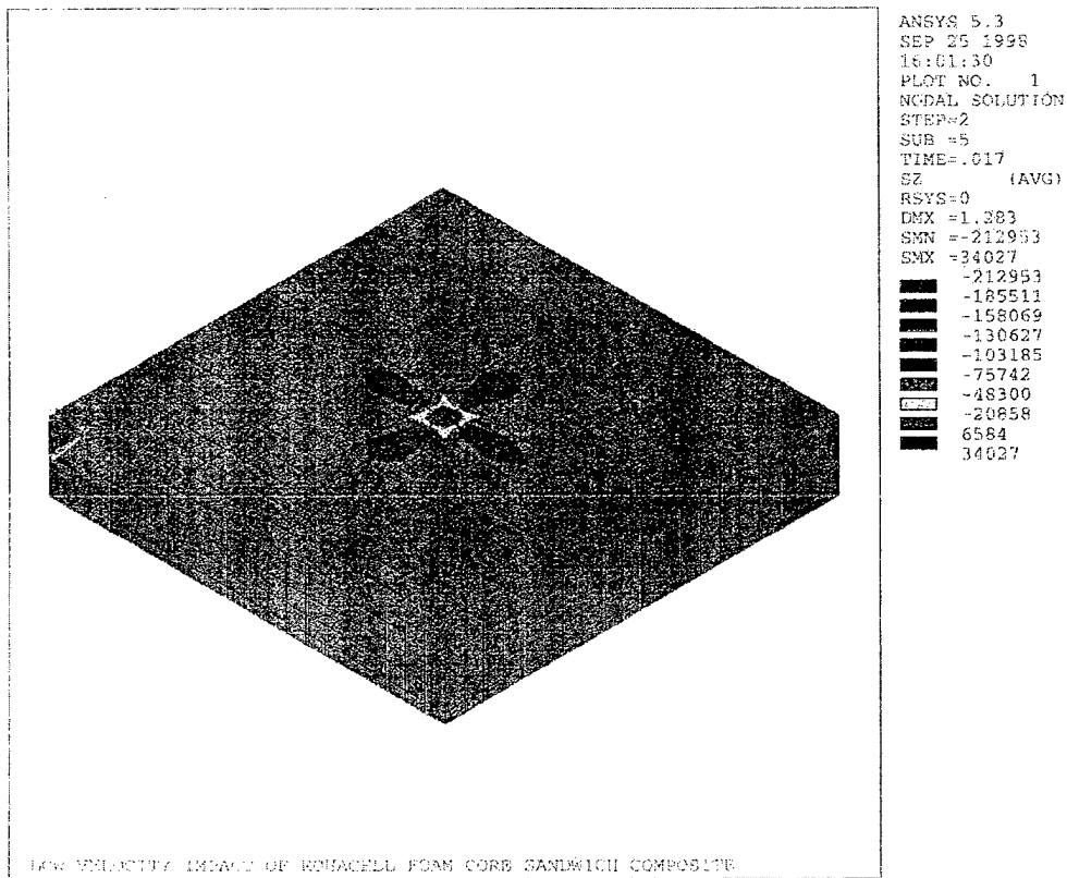
Figure 14.39. \sigma_z Distribution for Foam Core Sandwich Panel Under Low Velocity Impact.
