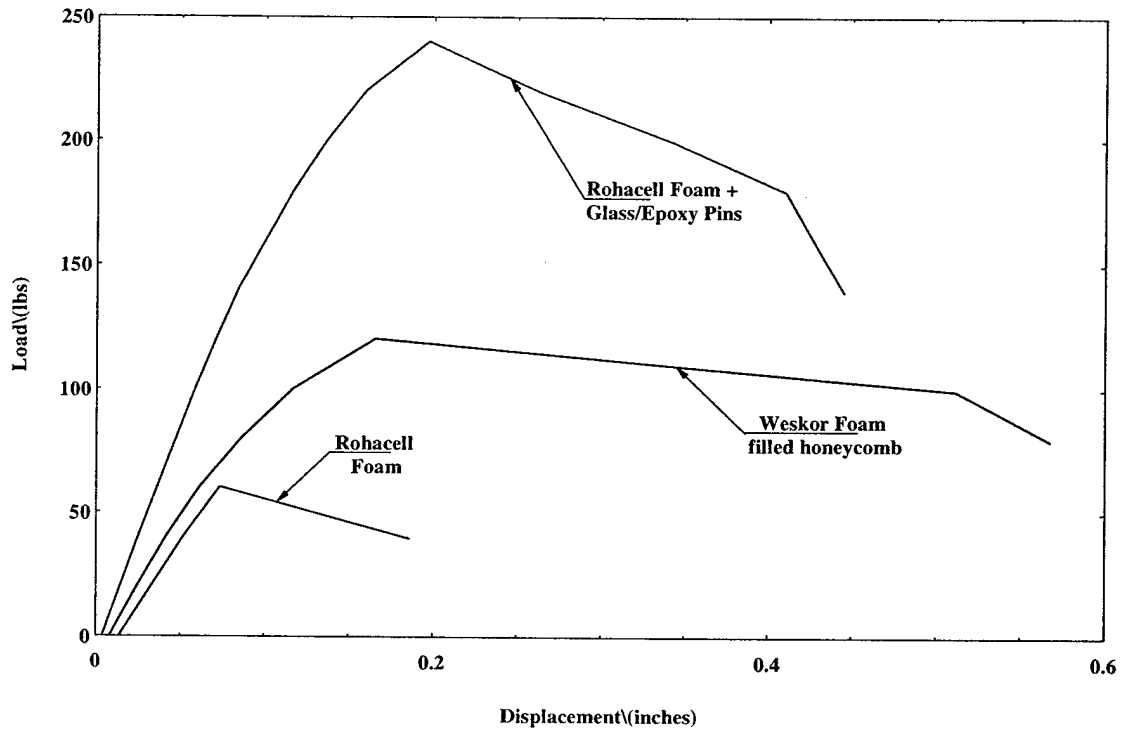
Figure 11.13 Flexural Load-Displacement Curves for Different Sandwich Composites
