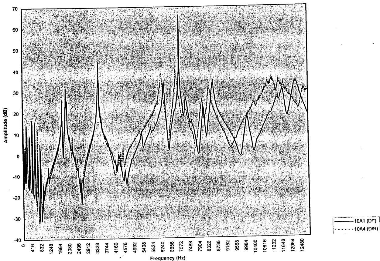
Figure 10.24 Comparison of FRF of 10 degree Pin Orientation Specimens Subjected to a Single Impact vs that Subjected to Repeated Impact
