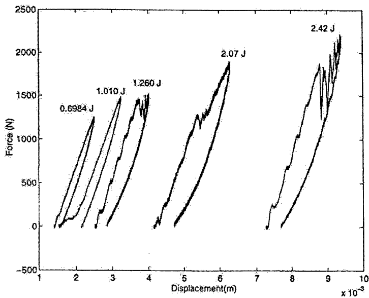
Figure 10.4 Load-Displacement Curves for five 10 Degree orientation Specimens Tested at Different Energy Levels
