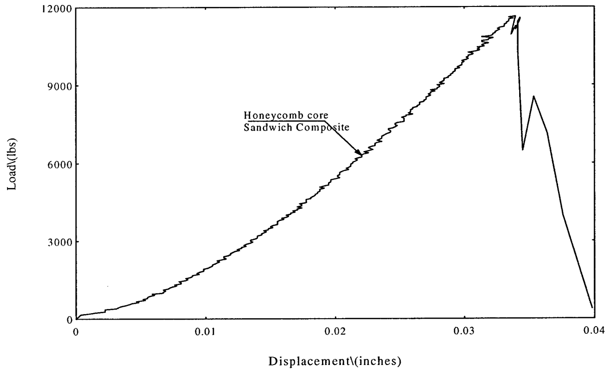
Figure 11.34. In-Plane Compression Load-Displacement Curve for Honeycomb Core Sandwich Composite
