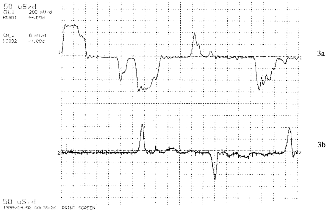
Figure 12.3a. Voltage vs Time Signal for Incident Bar (Strain) Figure 12.3b. Voltage vs Time Signal for Transmission Bar (Stress)
