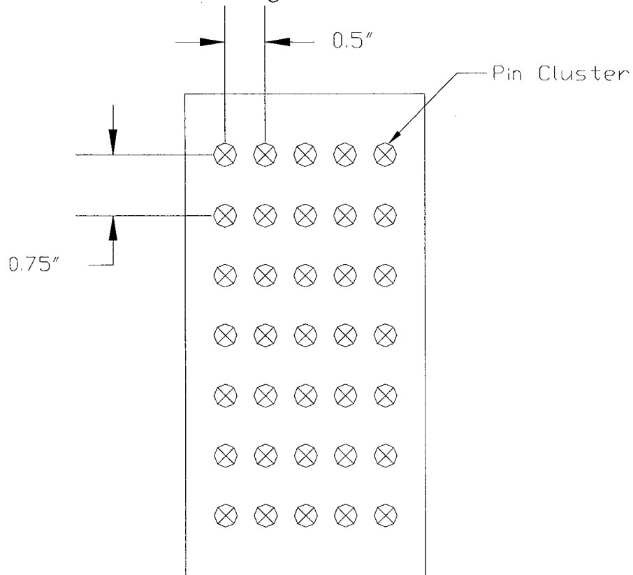
Figure 5.5 Lay-out of Truss Core Pins
