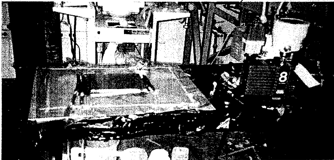
Figure. 5.9 a,b,c . Typical Vacuum Assisted Resin Transfer Molding : Co-Injection of Top and Bottom Facesheets
