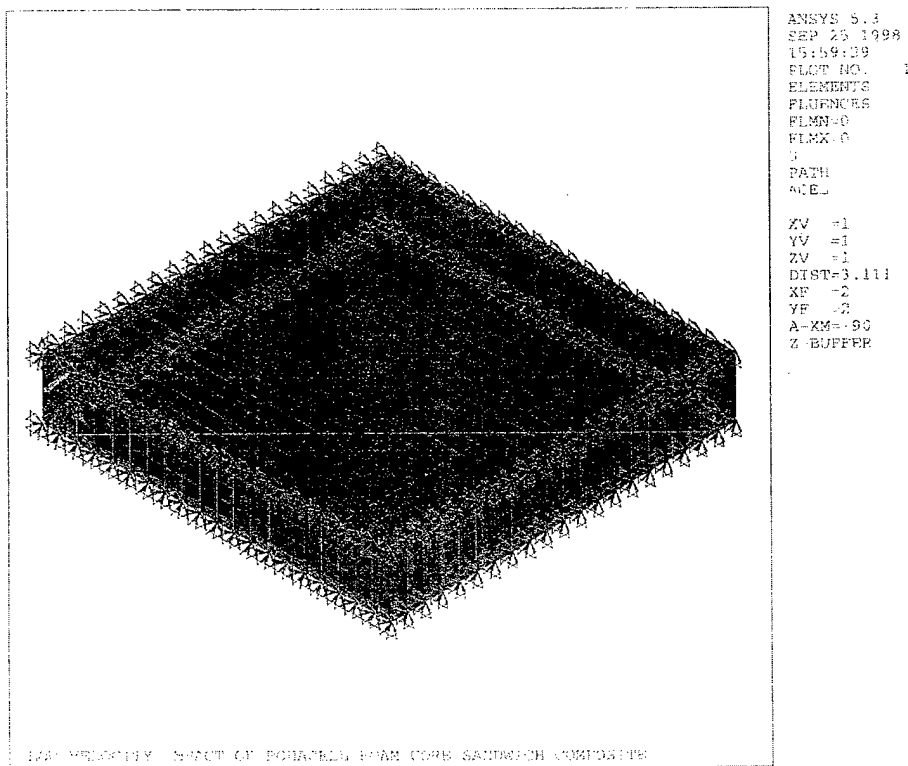
Figure 14.36. Constrains and Loading for Foam Core Sandwich Panel Under Low Velocity Impact
