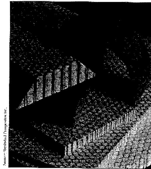
Figure 4.3b. Foam-Filled Honeycomb Core
