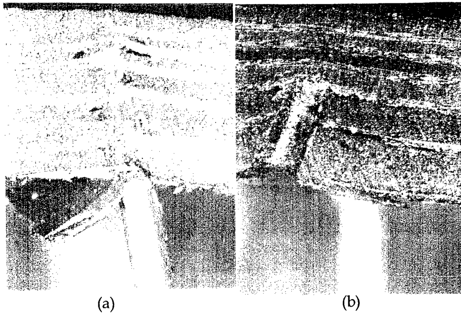
Figure 10.13a,b Pin Push out for the Top and Bottom facesheet
