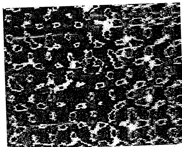
Figure 10.18a,b Ultrasonic C-Scans of a Specimen subjected to Quasi-Static Loading
