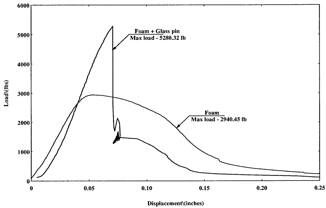
Figure 11.17 In-Plane Shear Load-Displacement Curves for Foam and Foam Reinforced with Glass/Epoxy Pins Core Sandwich Composite
