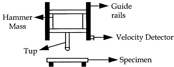
Figure 6.1 Schematic of a Dynatup Drop Weight Test System
