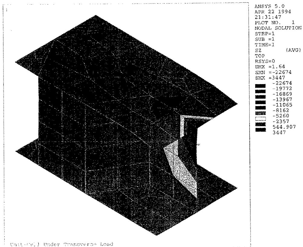
Figure 14.11. \sigma_z Distribution for Unit Cell Honeycomb Core With Facesheets Under Compression
