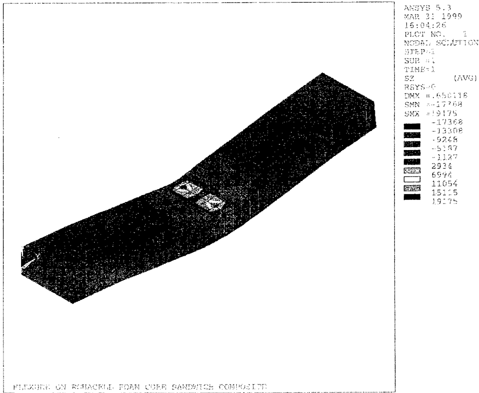
Figure 14.30. \sigma_z Distribution for Foam Core Sandwich Panel Under Flexure
