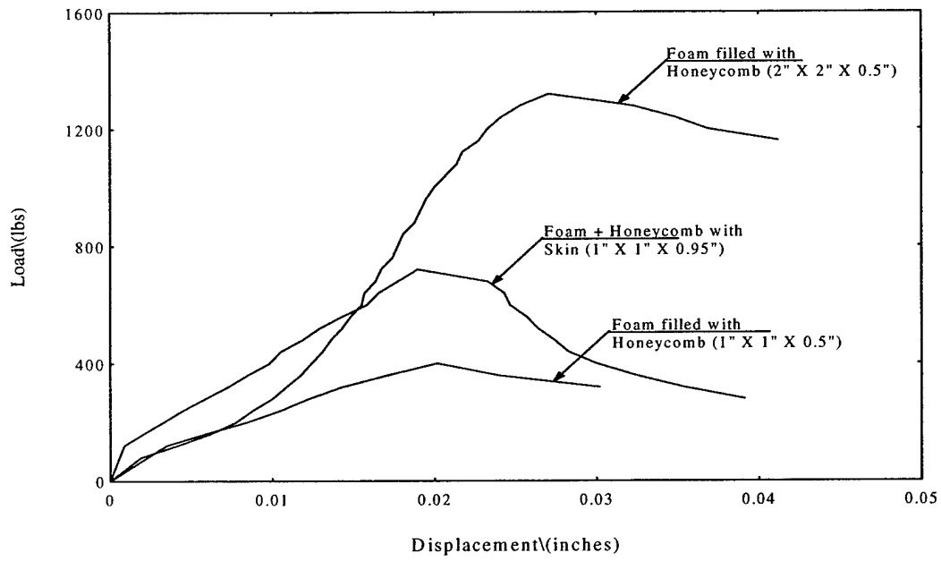
Figure 11.28. Load-Displacement Plot for Through the Thickness Compression Testing of WESKOR Foam Filled Honeycomb Core and its Sandwich Composite
