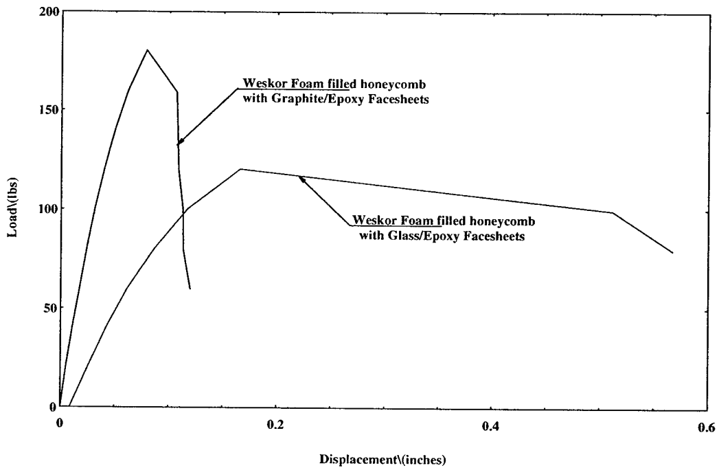
Figure 11.14 Flexural Load-Displacement Curves for WESKOR Foam filled Honeycomb Core with Glass and Graphite Facesheets
