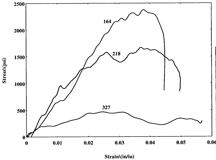
Figure 12.8b. Stress-Strain Curve for Foam + Glass Pins Without MTG
