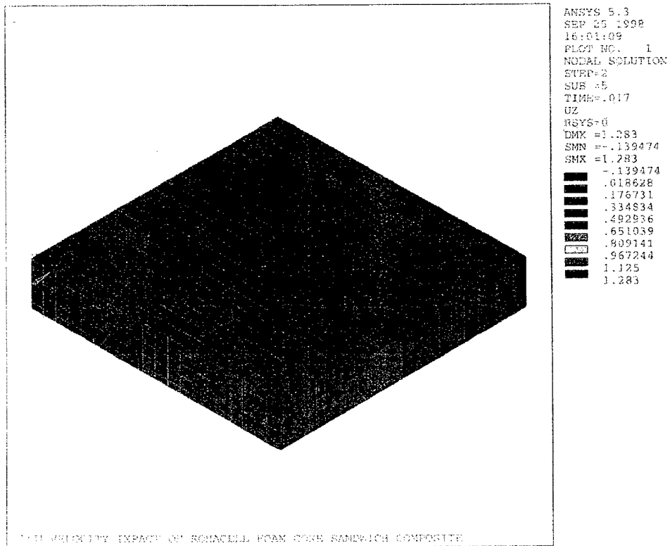
Figure 14.38. Displacement along Z-Direction for Foam Core Sandwich Panel Under Low Velocity Impact
