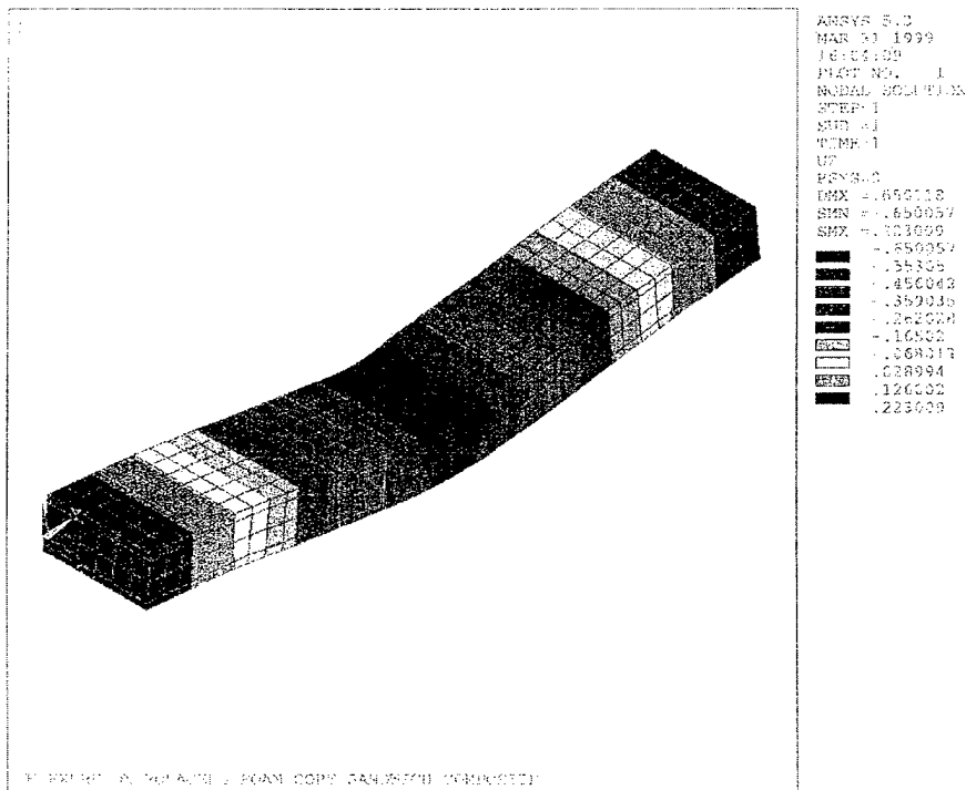
Figure 14.29. Distribution of Z- Direction Stress Under Flexure Loading of Foam Core Sandwich Panel
