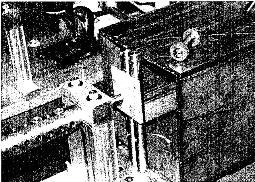
Figure 13.1. Schematic of Intermediate Velocity Impact Test Set-Up The instrument is a modified version of the Split Hopkinson Pressure Bar used in high strain rate testing experiments. a) Details of the Fixture, b) Specimen Mounted on the Fixture
