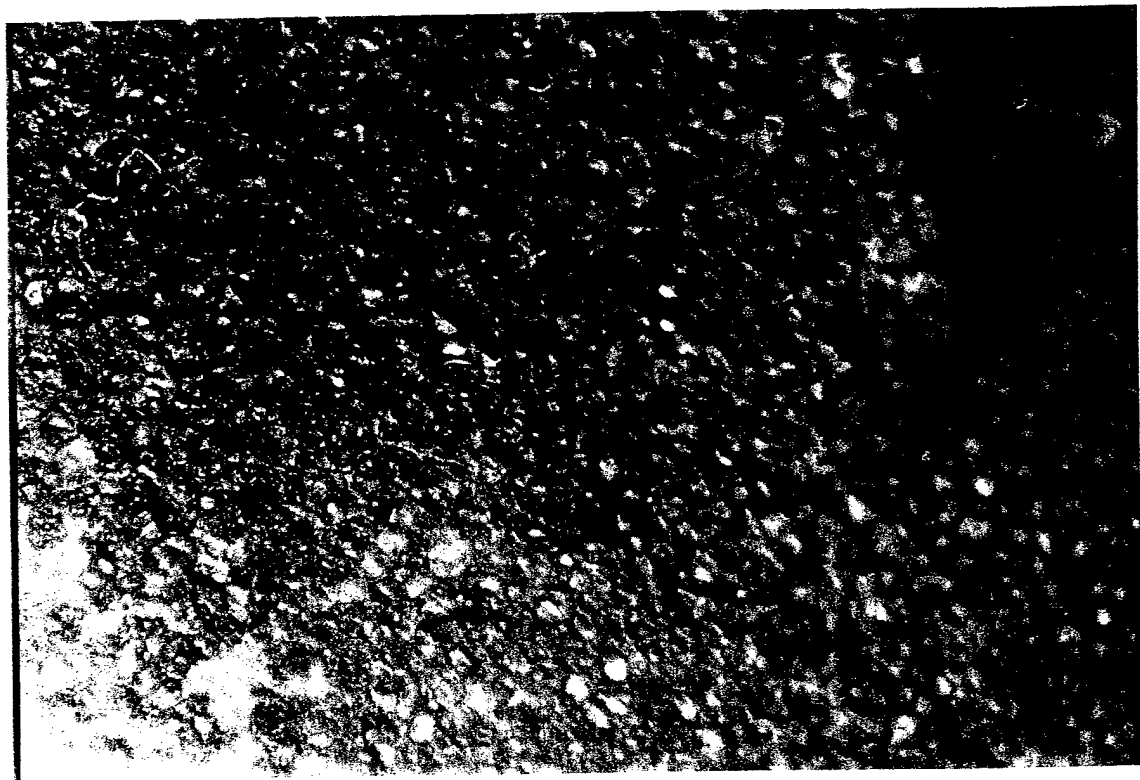
Figure 8.23a and b. Facesheet to core disbond and core crushing for FCo-32 Composite (Energy Level E)
