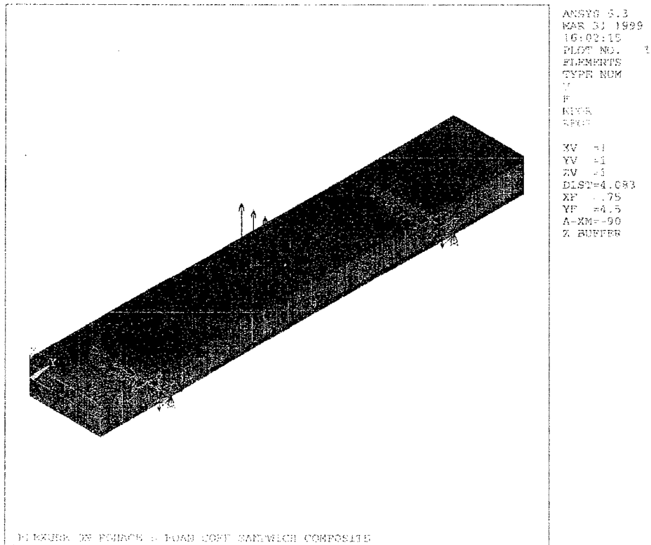
Figure 14.26. Foam Core Sandwich Panel Under Flexural Loading
