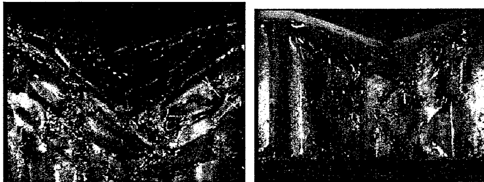
Figure 8.12.5 LVI a) from graphite/epoxy facesheet side, b) from glass/epoxy facesheet side
