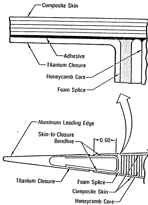
Figure 1.1. a, b and c. Some Application of Composites and Sandwich Constructions in Aircraft Parts
