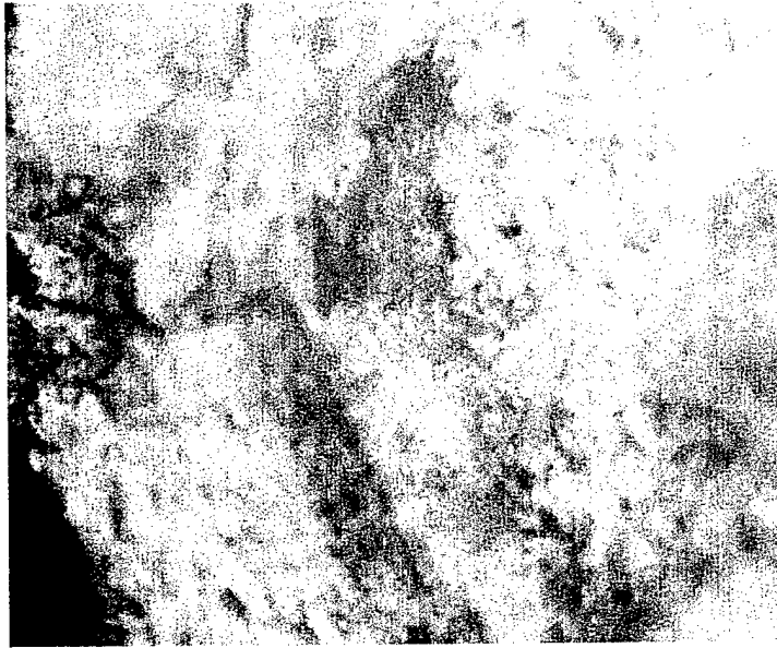
Figure 11.31. Failure Photograph of WESKOR Foam Filled Honeycomb Core under In-Plane Compression Loading
