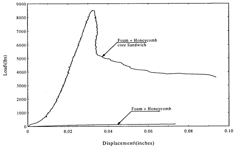
Figure 11.37. In-Plane Compression Load-Displacement Curve for WESKOR Foam Filled Honeycomb Core and its Sandwich Composite
