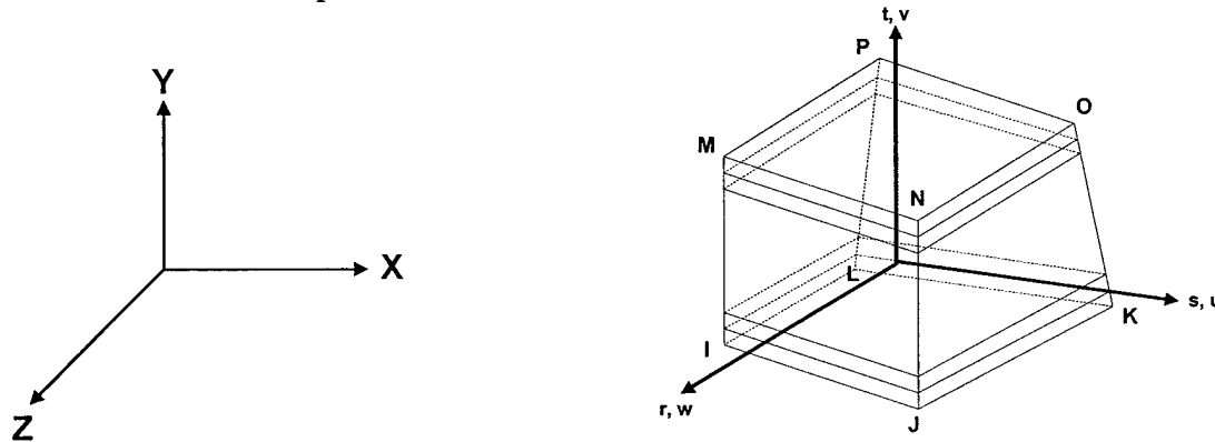
Figure 14.15 SOLID46 element with eight corner nodes (I-J-K-L-M-N-O-P)
