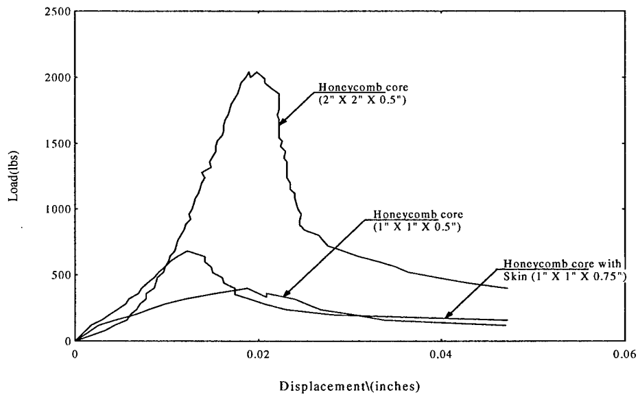
Figure 11.26. Load-Displacement Plot for Through the Thickness Compression Testing of Honeycomb Core and its Sandwich Composite
