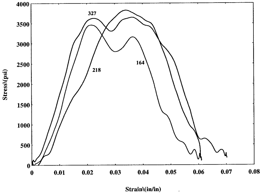
Figure 12.8a. Stress-Strain Curve for Foam + Glass Pins With MTG
