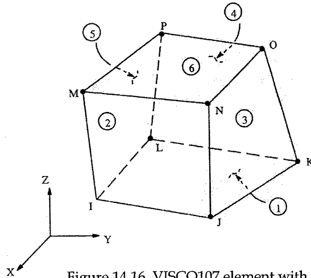
Figure 14.16 VISCO107 element with eight corner nodes (I-J-K-L-M-N-O-P)
