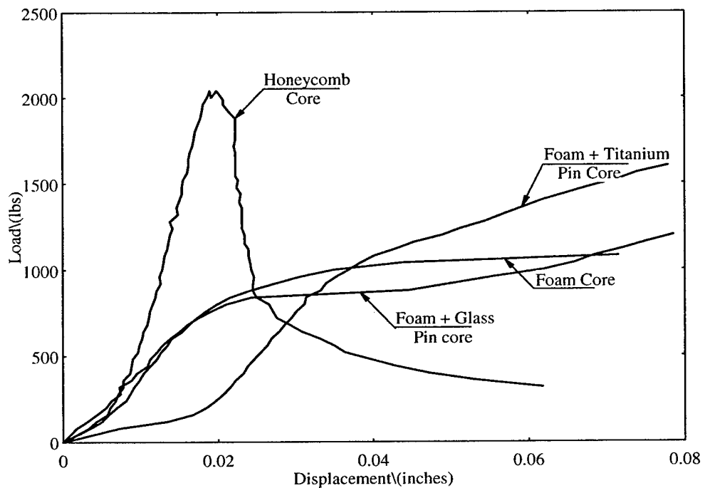
Figure 11.22. Through Thickness Compression Load-Displacement Plot for Different Cores
