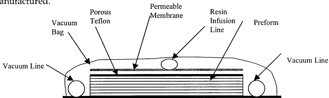
Figure 5.3 Schematic of VARTM process
