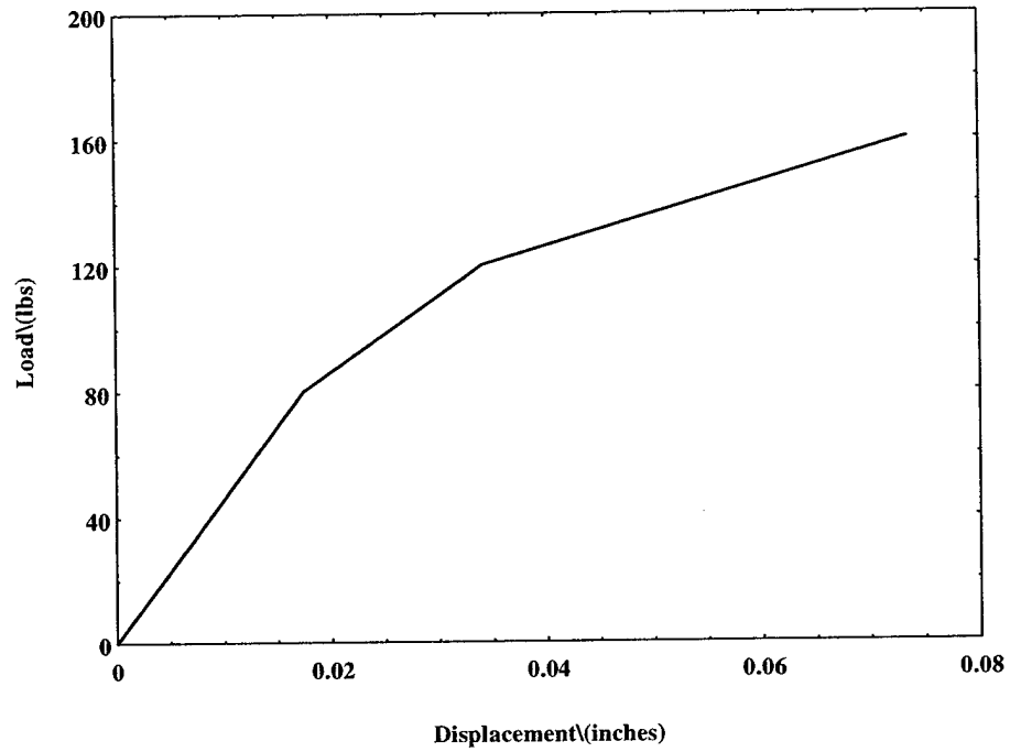
Figure 11.33. Load-Displacement Curve for WESKOR Foam Filled Honeycomb Core Under In-Plane Compression Loading
