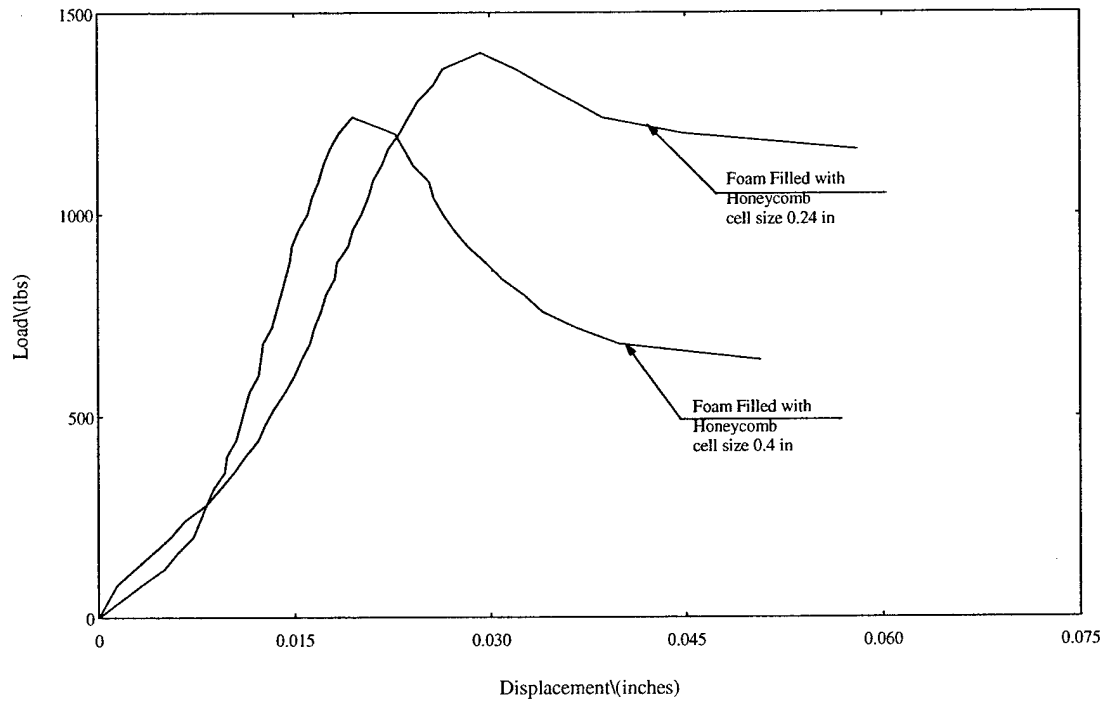
Figure 11.30. Load-Displacement Plot for Through the Thickness Compression Testing of Weskor Foam Filled Honeycomb Core With Different cell Spacing
