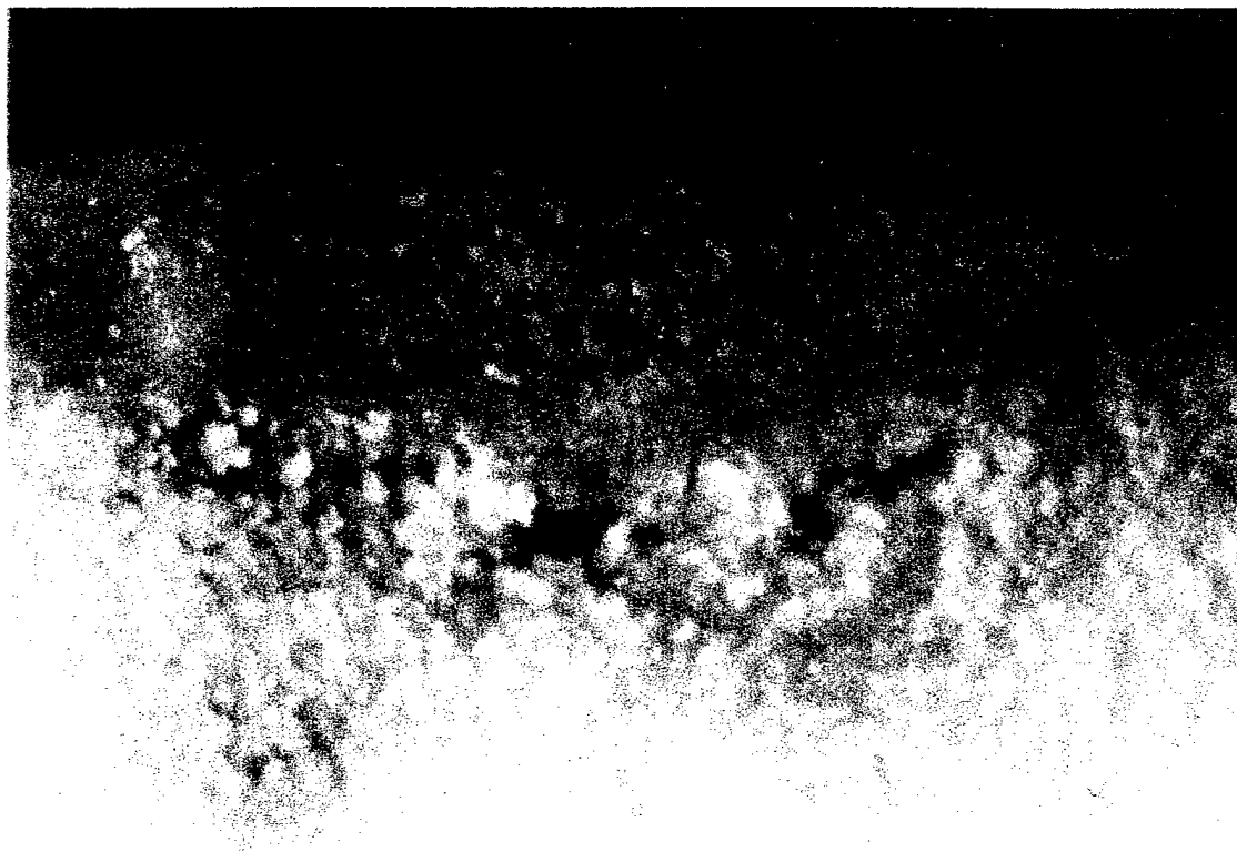
Figure 8.40. Facesheet to Skin Disbond, Core Crushing and Facesheet Flexure for the F+PCo-75 (Glass Pins) Composite (Energy Level E)
