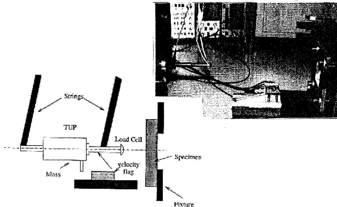
Figure 6.4 Swing Pendulum Setup for LVI of Hollow Steel Pin Core Sandwich Composites
