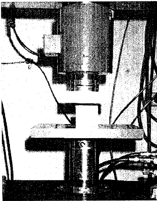
Figure 11.1c Illustration of Static Compression Testing of Sandwich Composites
