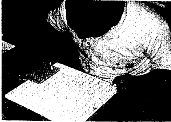
a) Preparation of Titanium Pin Reinforced Rohacell Foam Core. Pins are guided at specific angles through Plexiglass Mold
