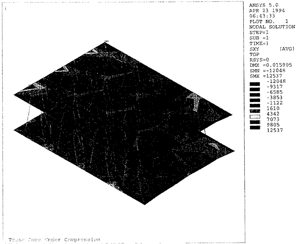
Figure 14.5. \tau_{xy} Distribution for Z-Pin Sandwich Panel Under CAI
