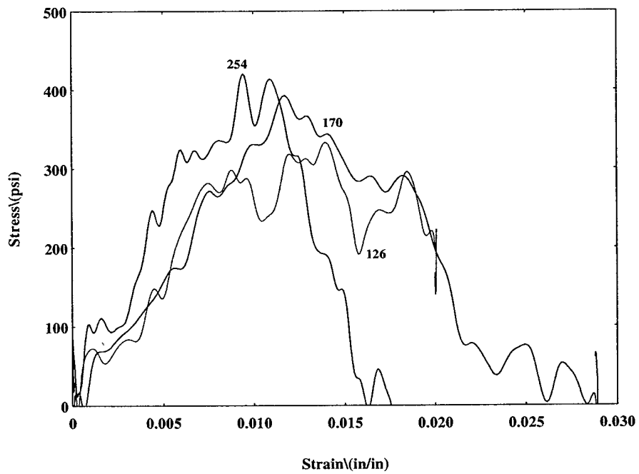
Figure 12.11b. Stress-Strain Curve for Honeycomb Core Sandwich Composite (1.5" Bar)
