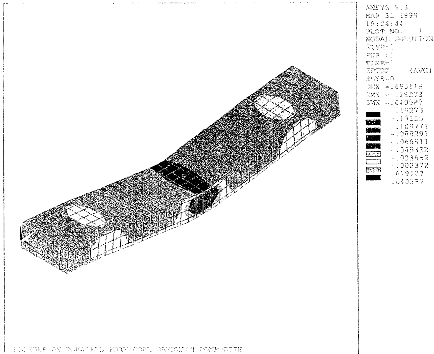
Figure 14.31. Total Strain in Z- Direction for Foam Core Sandwich Panel Under Flexure
