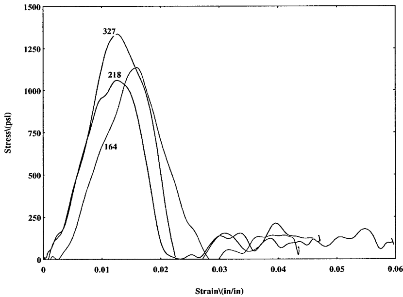
Figure 12.6b. Stress-Strain Curve for Honeycomb Core Sandwich Composite Without MTG
