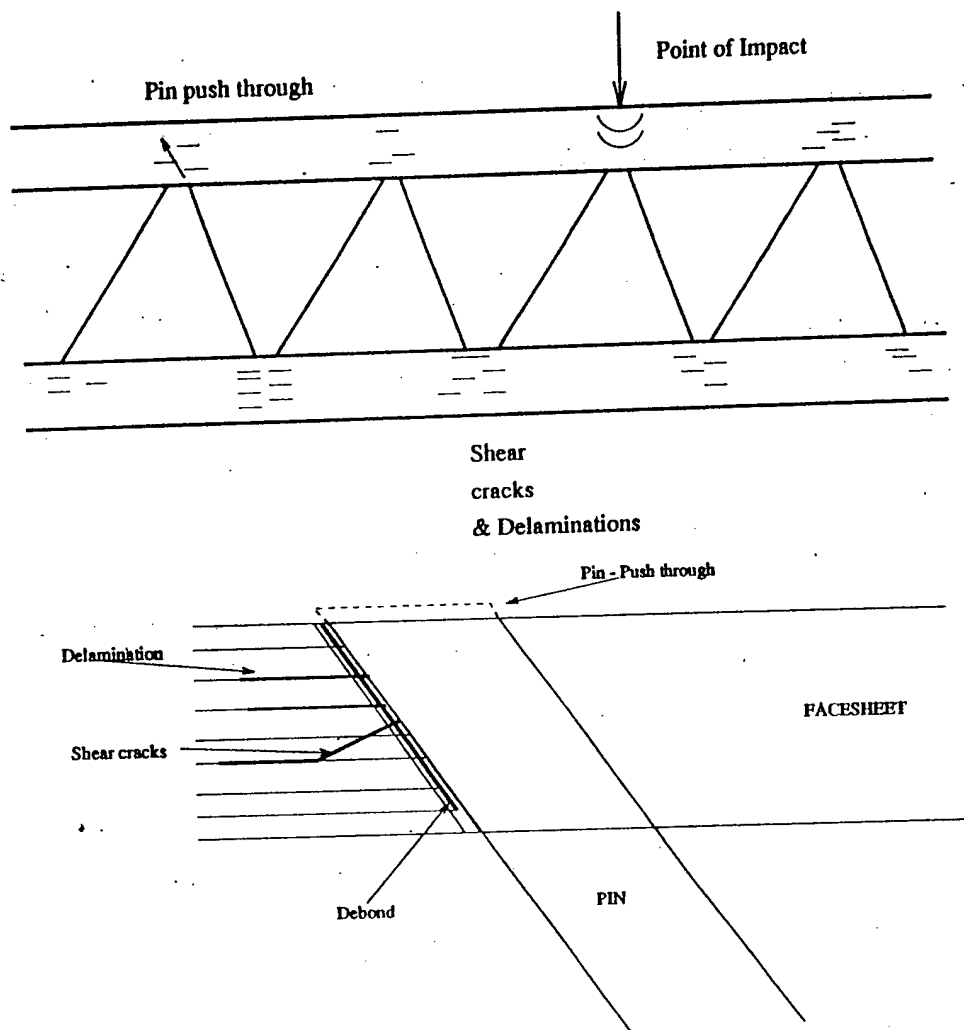
Figure 10.14a&b. Schematic of failure as observed across the top and bottom facesheets
