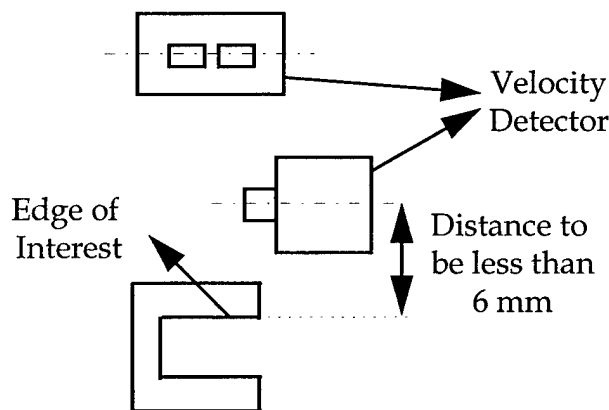
Figure 6.2 Adjustment of Velocity Detector and Flag in the Drop Weight Test System
