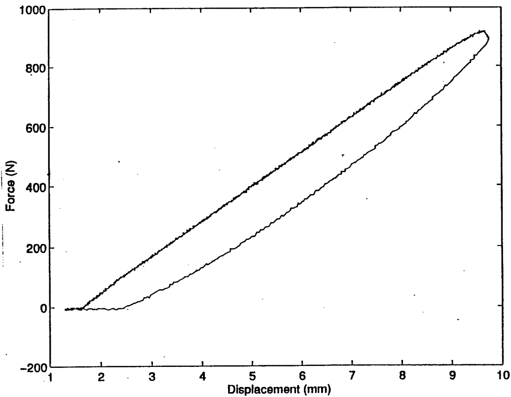
Figure 10.10 Static Load-Displacement curves for 10 degree pin orientation specimen
