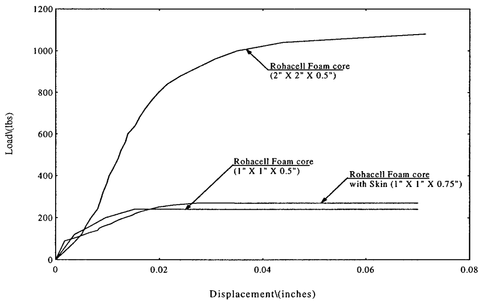
Figure 11.27. Load-Displacement Plot for Through the Thickness Compression Testing of Rohacell Foam Core and its Sandwich Composite
