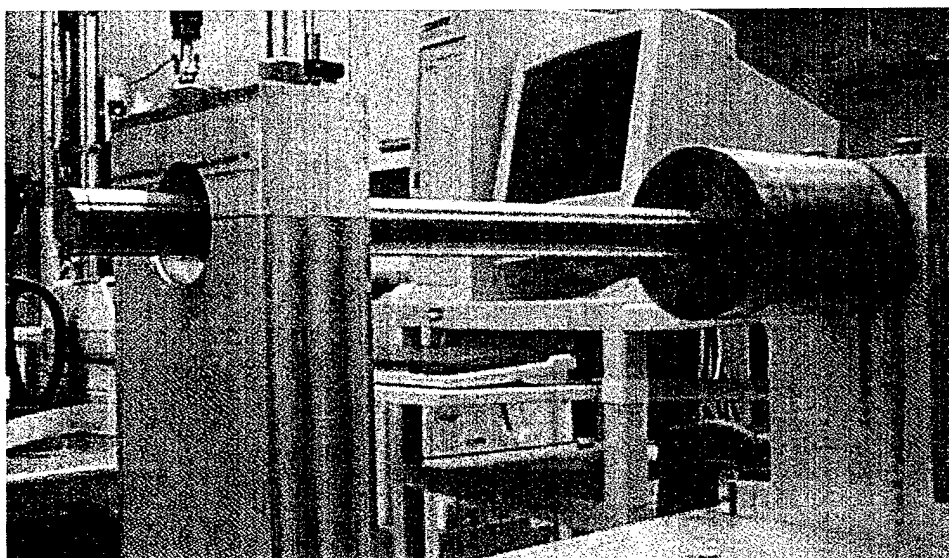
Figure 12.2b. Momentum Trap (Dynamic Recovery Technique)
