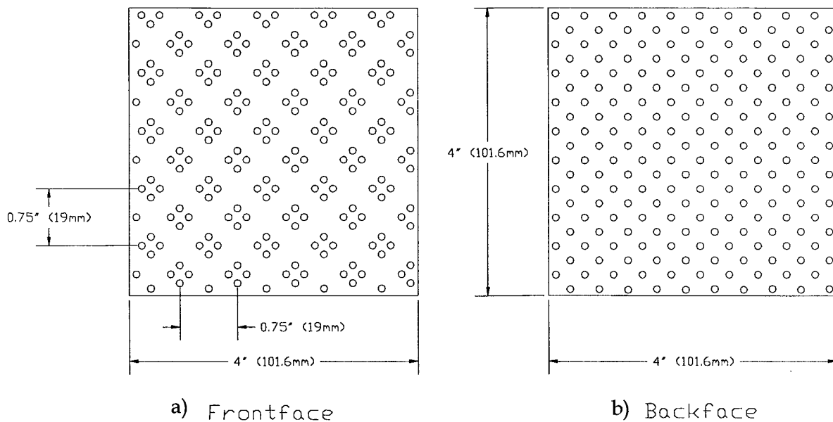
Figure 5.12 a and b. Pin Spacing and Arrangement Within Foam Core
