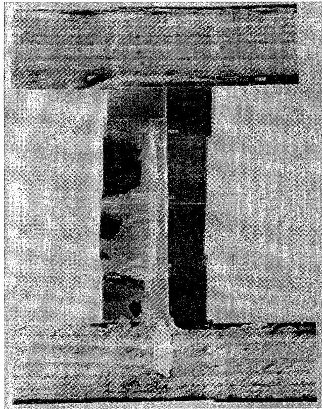
Figure 10.12. Incipient Damage at Pin-Facesheet Interface
