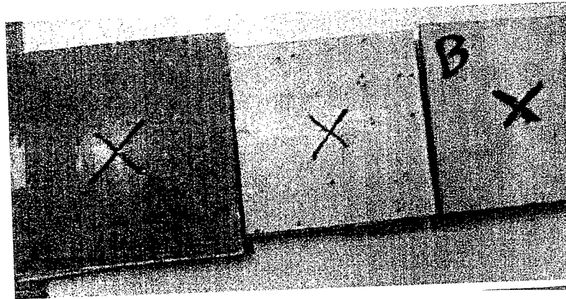
Figure 13.2 . Intermediate Velocity Impact Failure of Foam, Titanium Pins Reinforced Foam and Hollow Titanium Z-Pins Reinforced Core a) and b) represent different details for the same samples. c) Top View of the samples
