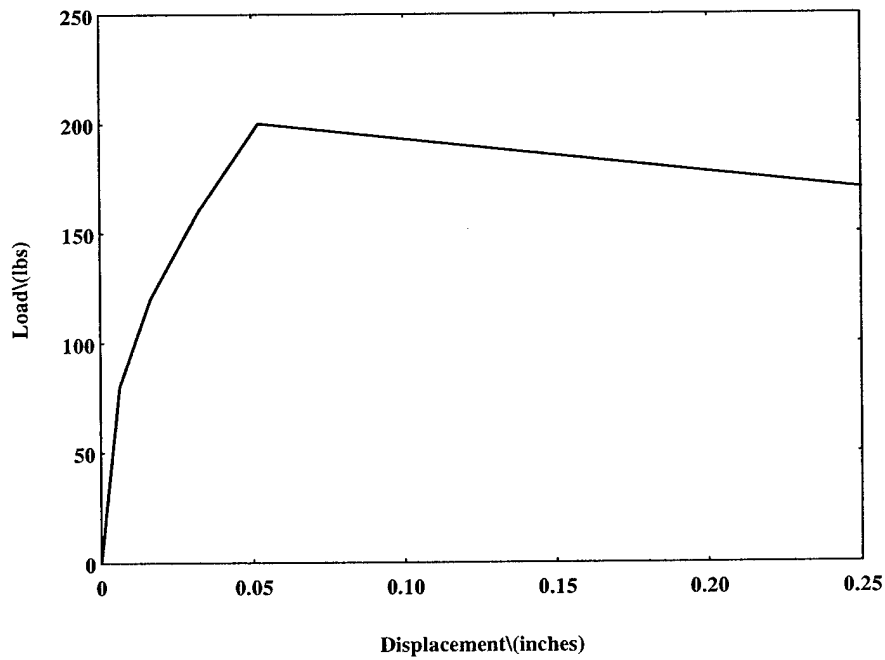
Figure 11.32. Load-Displacement Curve for Rohacell Foam Reinforced with Titanium Pin Core Under In-Plane Compression Loading
