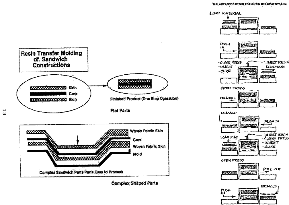
Figure 1.8 Schematic of RTM Processing
