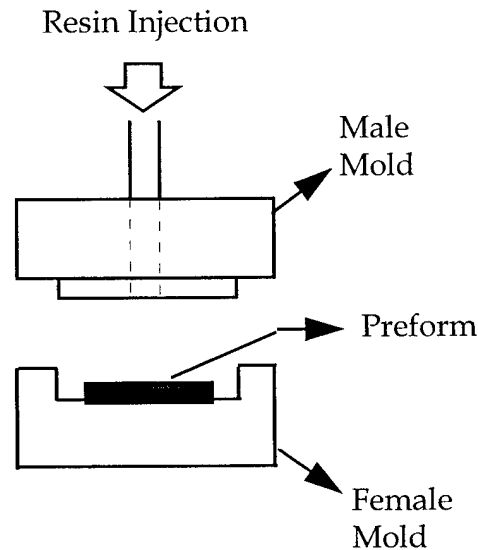
Figure 5.2a Schematic of Resin Transfer Molding
