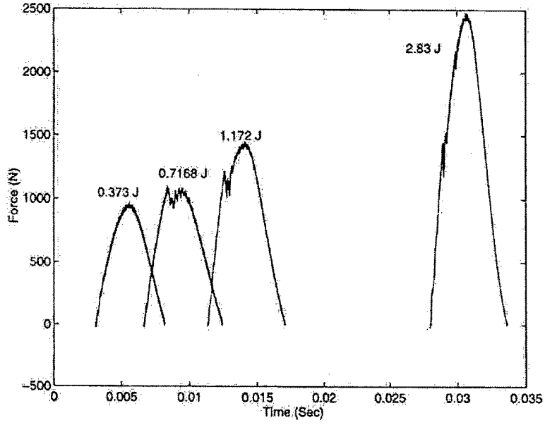
Figure 10.6 Force-Time Curves for five 20 Degree orientation Specimens Tested at Different Energy Levels
