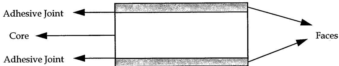
Figure 2.1 Schematic of a Sandwich Construction
