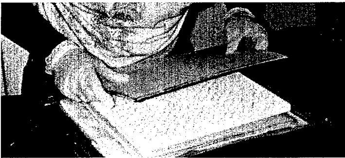
Figure 5.13a-e Photographs of Manufacturing of Pin-Reinforced Foam Core Sandwich Composite Samples
