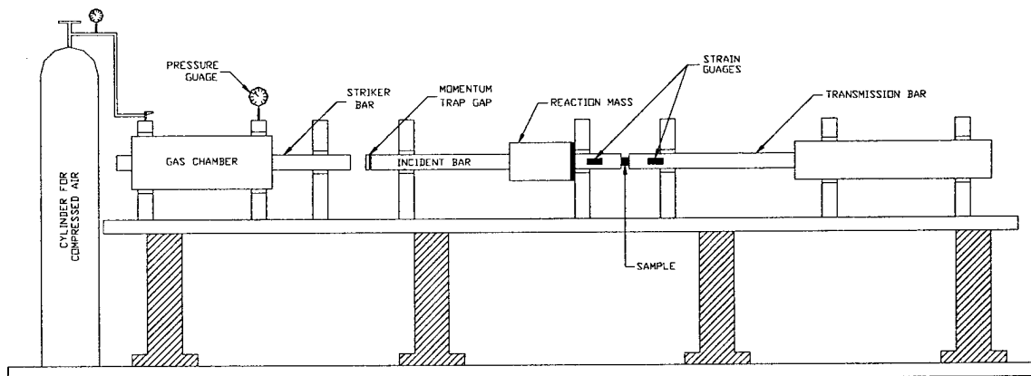
Figure 12.1a. Schematic of Split Hopkinson Pressure Bar
