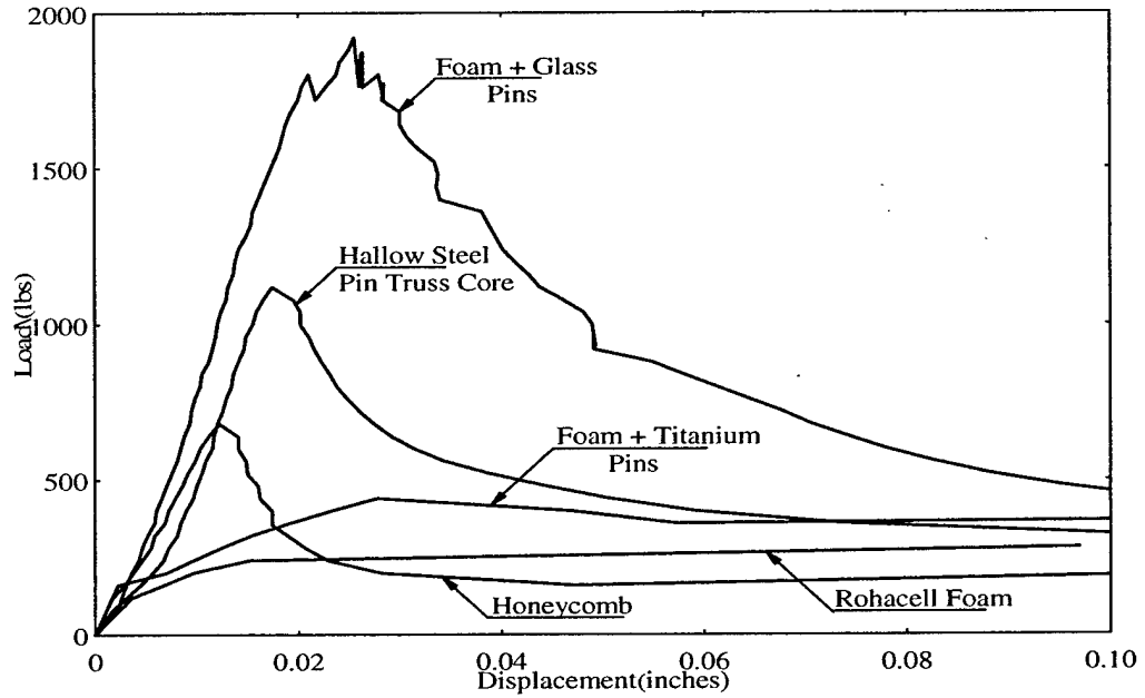
Figure 11.24. Through Thickness Compression Load-Displacement Plot for Different Sandwich Composites
