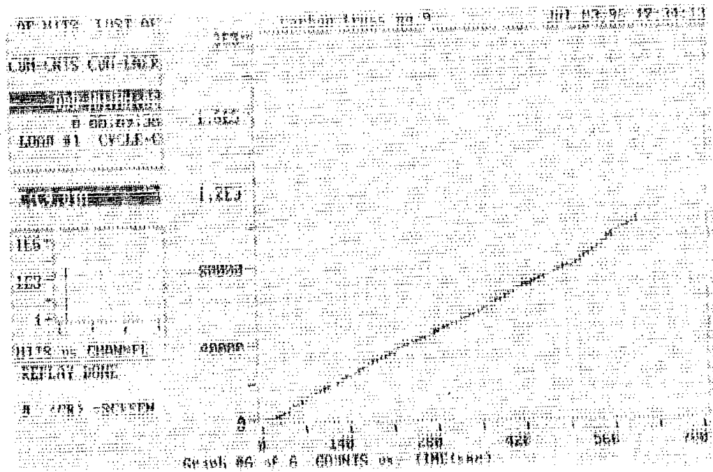
Figure 11.10. AE Response in terms of Cumulative AE Activity for Graphite/Epoxy Truss Core Composite
