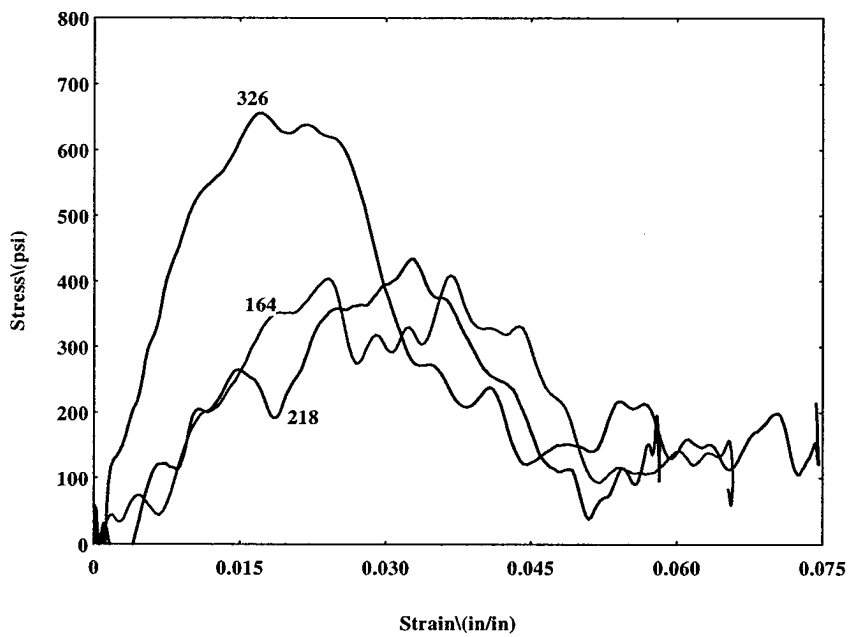
Figure 12.9b. Stress-Strain Curve for Hollow Steel Pin Truss Core Sandwich Composite Without MTG
