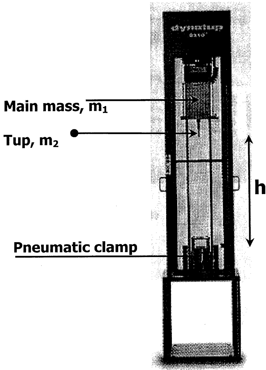
Figure 6.3. Dynatup 8210 Used for Low Velocity Impact Testing
