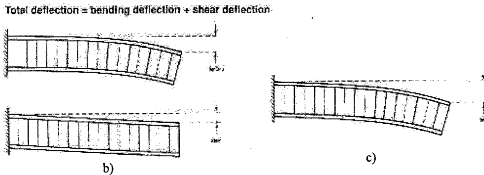
Figure 2.2b & c Illustration of the Working of a Sandwich Beam [1]
