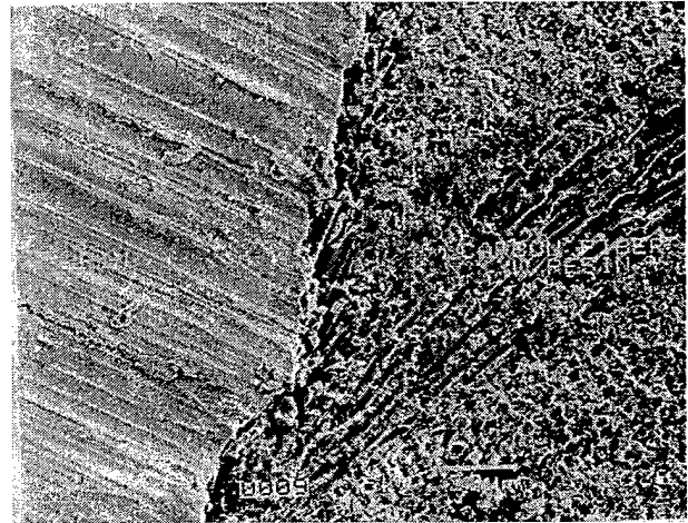
Figure 10.15a,b SEM Photographs showing the Shear Crack and Delamination in the Facesheet around the Pins
