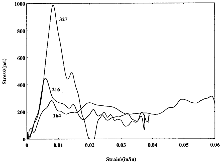
Figure 12.10b. Stress-Strain Curve for Foam+Honeycomb Core Sandwich Composite Without MTG
