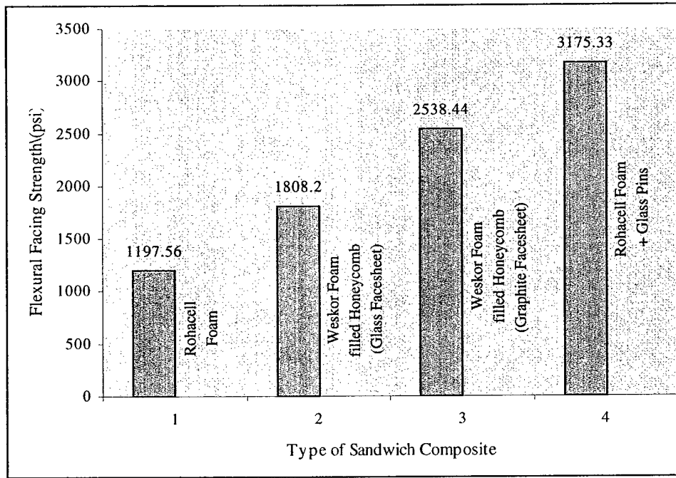
Figure 11.15 Comparison of Flexural Strength for Different Sandwich Composites
