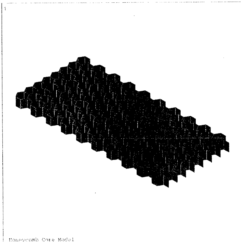
Figure 14.13. Honeycomb Core With Multiple Cell Model
