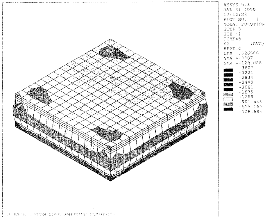
Figure 14.21. \sigma_z Distribution for Foam Core Sandwich Panel Under Transverse Compression.
