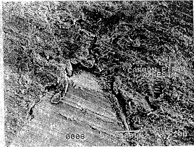
Figure 10.15a,b SEM Photographs showing the Shear Crack and Delamination in the Facesheet around the Pins
