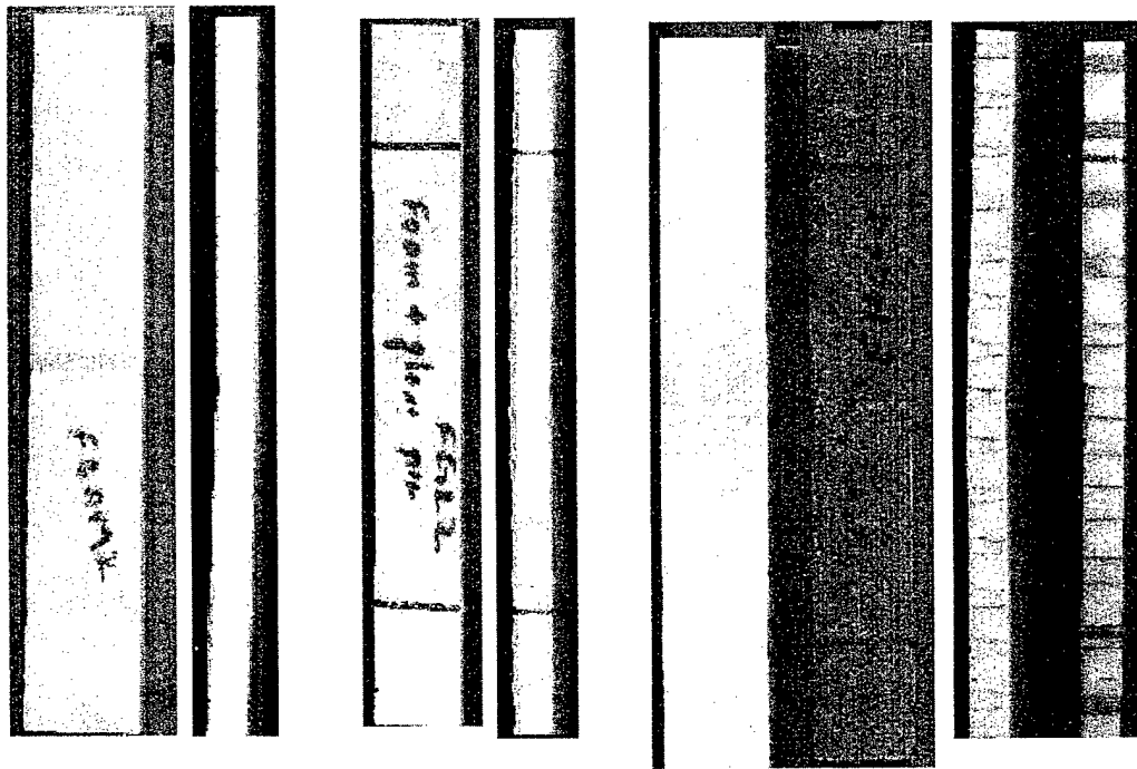
Figure 11.16 Flexural Failure Photographs for Different Sandwich Composites
