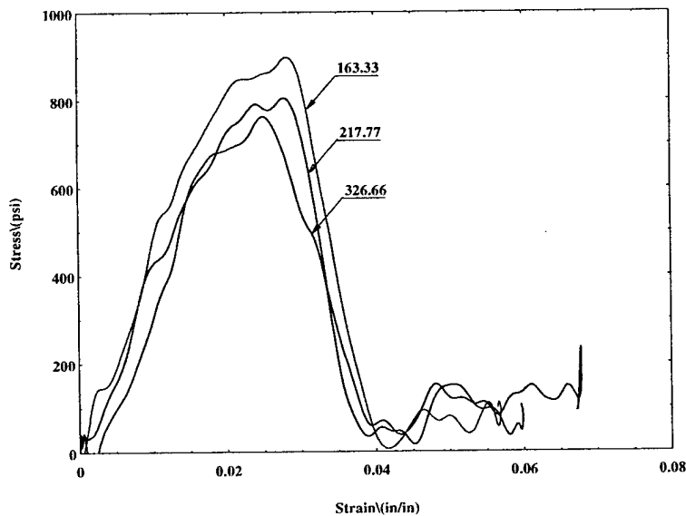
Figure 12.16b. Stress-Strain Curve for Nomex Honeycomb Core With Hybrid Facesheets (Without MTG) – Glass/Epoxy Facesheet Facing
