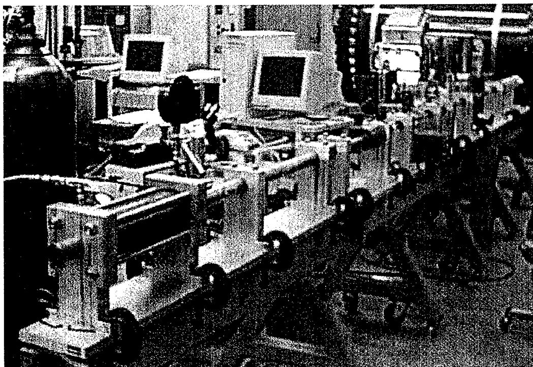
Figure 12.1b. Split Hopkinson Pressure Bar
