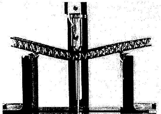
Figure 4.4 Hollow Truss (Z-Pin) Core Sandwich Composite [5]
