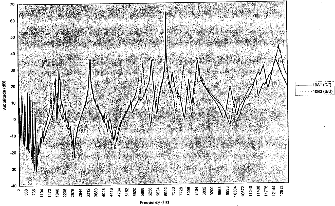
Figure 10.25 Comparison of FFF for an Impact Loaded Specimen and Statically Loaded Specimen
