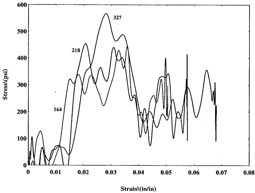
Figure 12.5a. Stress-Strain Curve for Foam Core Sandwich Composite With MTG
