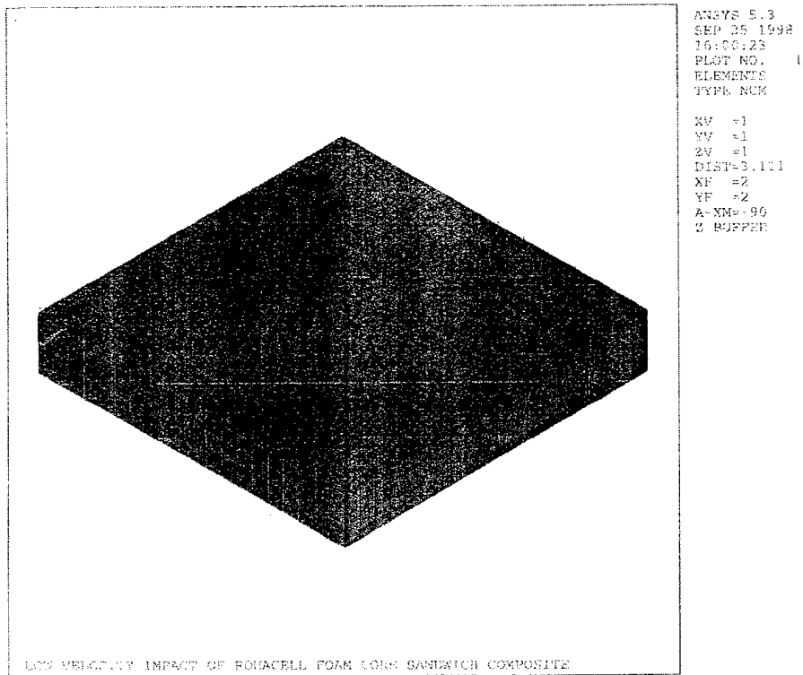
Figure 14.35. Foam Core Sandwich Panel Model for Low Velocity Impact
