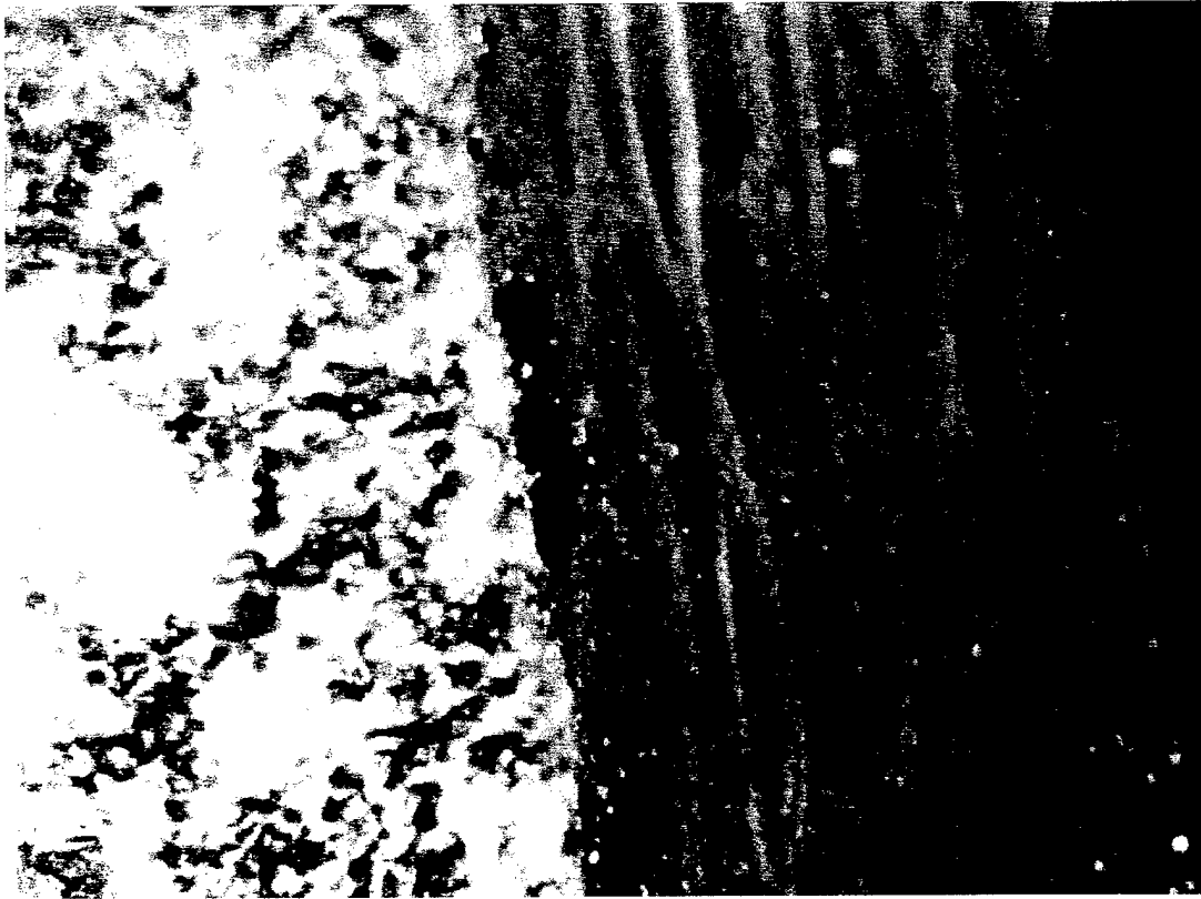
Figure 7.6. Bottom Facesheet Failure for Impact Level D (16-Ply Graphite/Vinyl Ester Facesheets)
