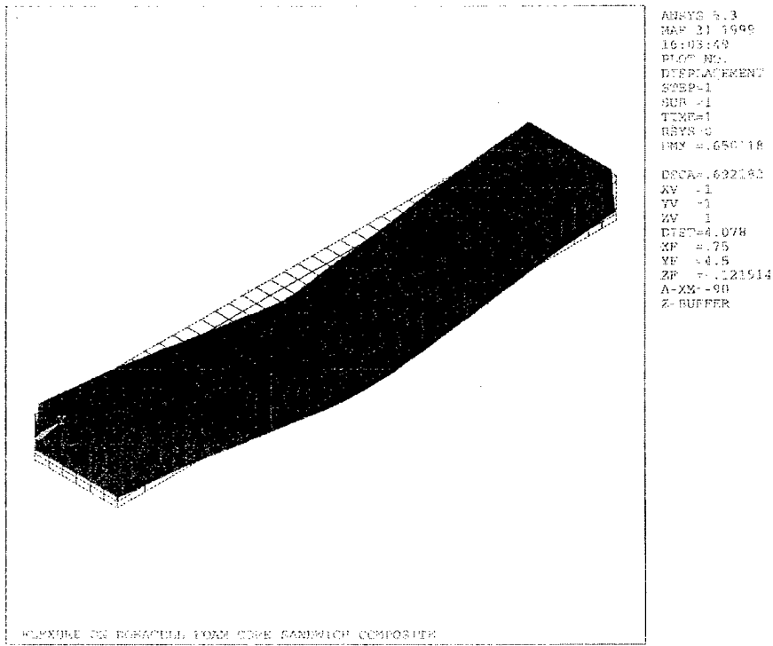
Figure 14.28. Deformed Foam Core Sandwich Panel Under Flexure
