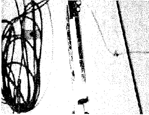
Figure 11.18a Crack Initiation at the Ends
