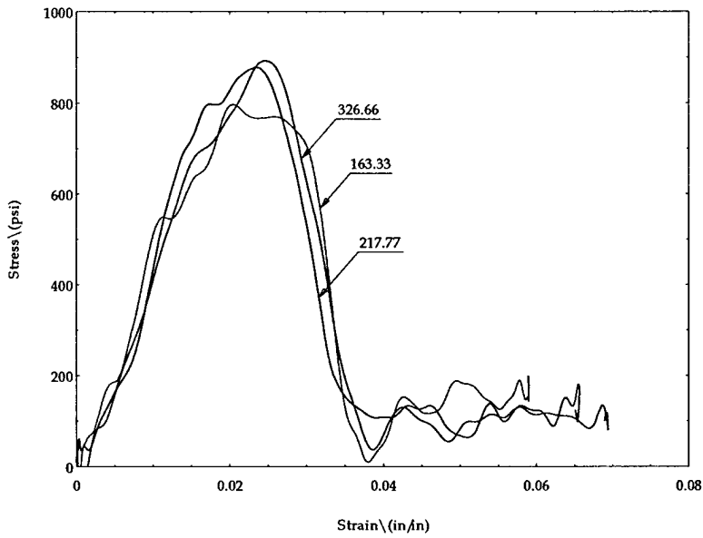
Figure 12.17b. Stress-Strain Curve for Nomex Honeycomb Core With Hybrid Facesheets (Without MTG) – Graphite/Epoxy Facesheet Facing
