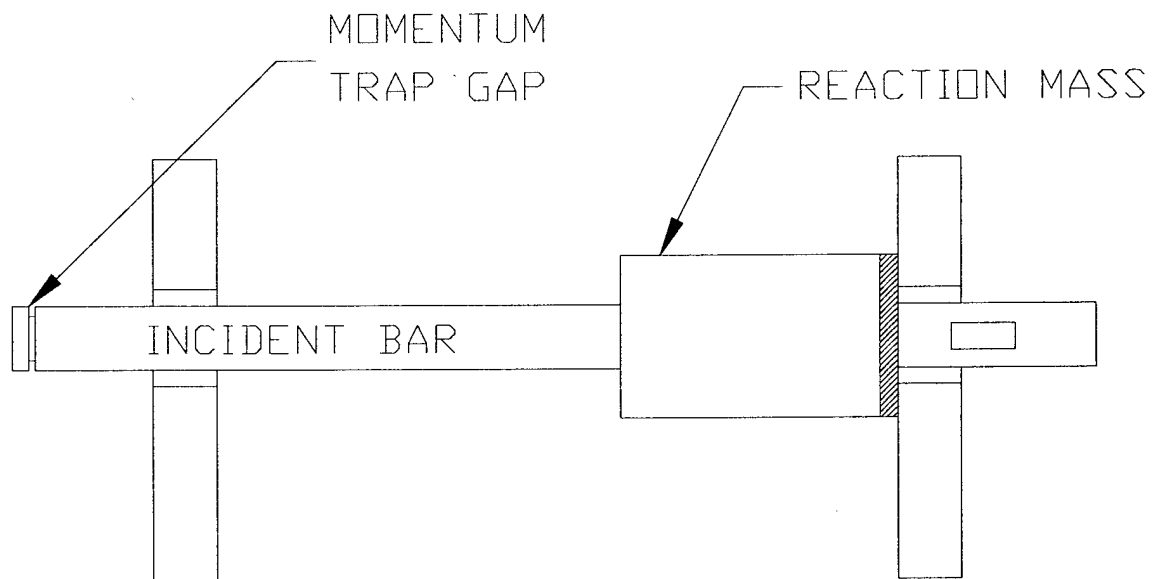
Figure 12.2a. Schematic of Momentum Trap Setup
