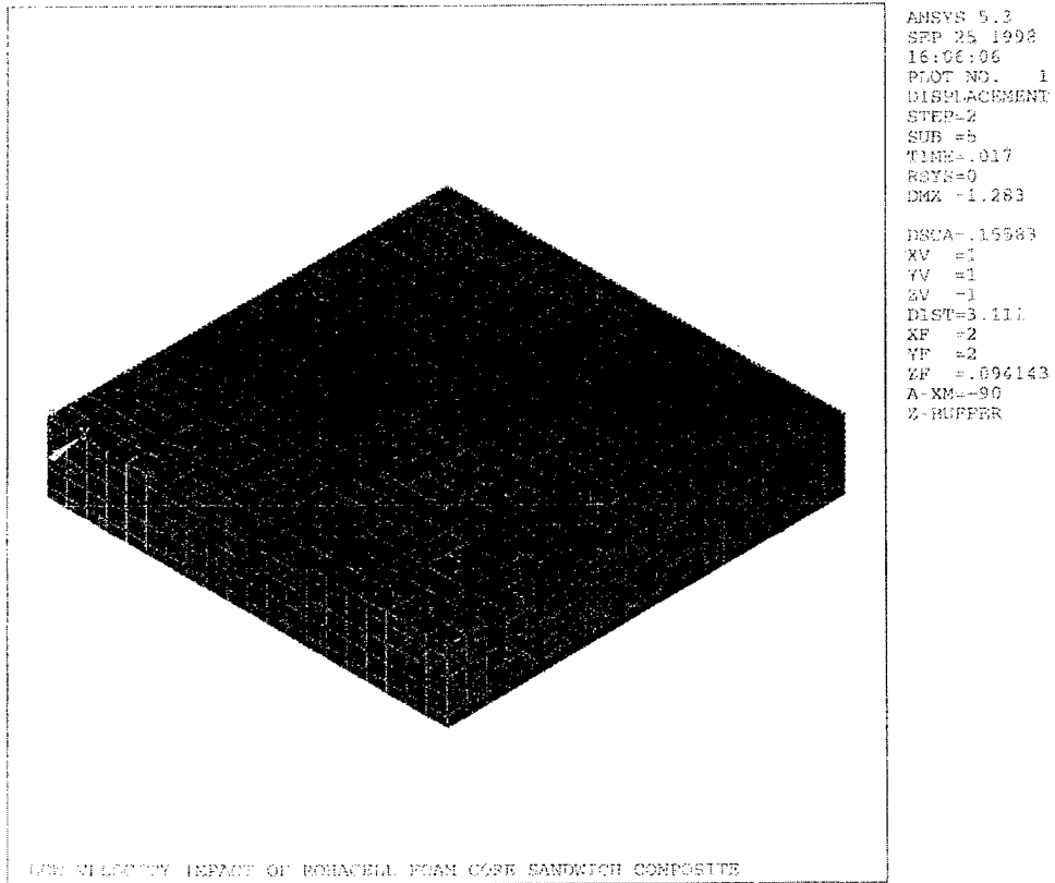
Figure 14.37. Deformed Foam Core Sandwich Panel Under Low Velocity Impact
