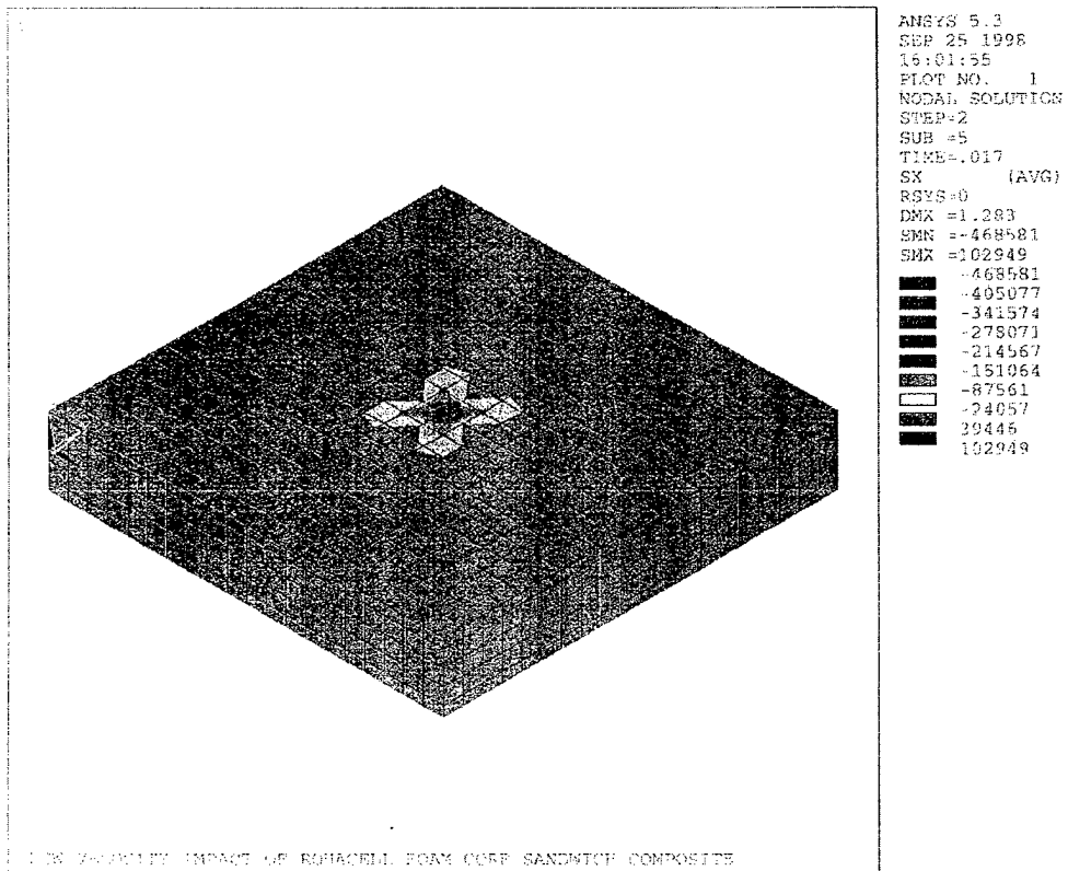
Figure 14.40. \sigma_x Distribution for Foam Core Sandwich Panel Under Low Velocity Impact
