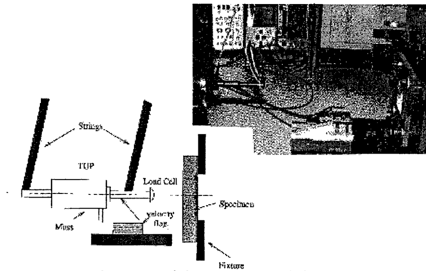
Figure 10.2 Schematic of the Swing Pendulum Test System
