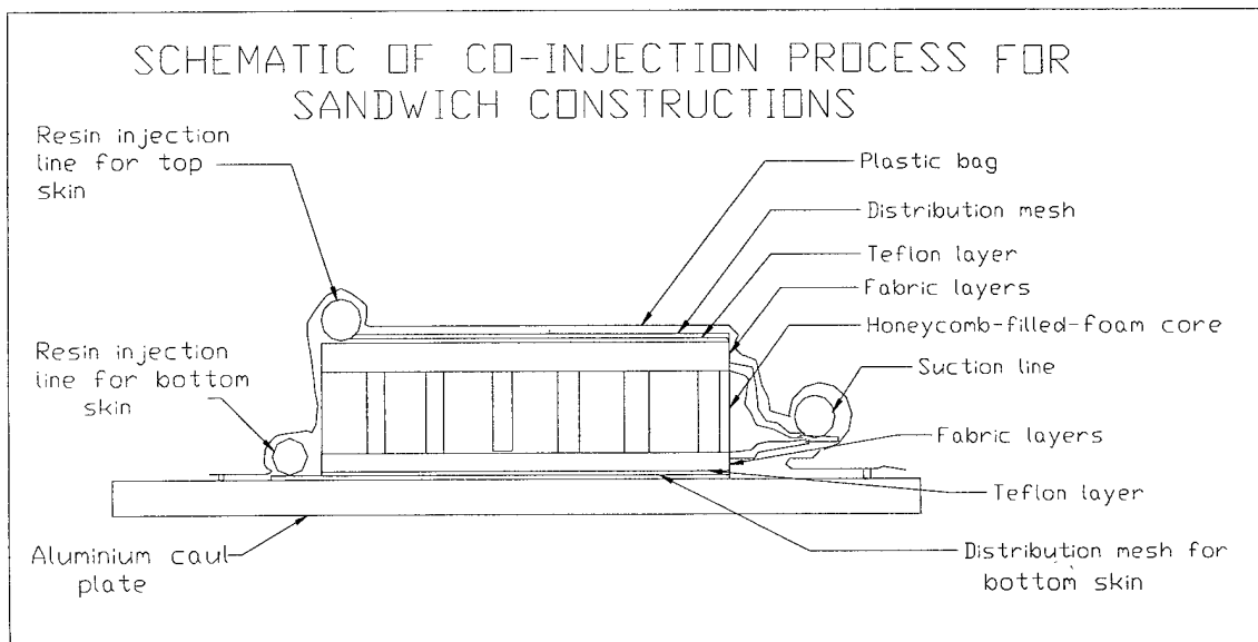
Figure 5.8a. Detailed Schematic of Co-Injection Process
