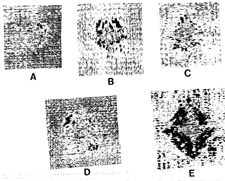
Figure 7.7 Ultrasonic C-scans for Impact Side of Graphite/Epoxy Facesheet and Foam Filled Honeycomb Core Sandwich Composites Impacted at Energy Levels A-E
