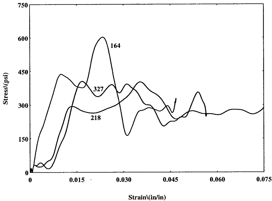
Figure 12.7b. Stress-Strain Curve for Foam + Titanium Pins Without MTG
