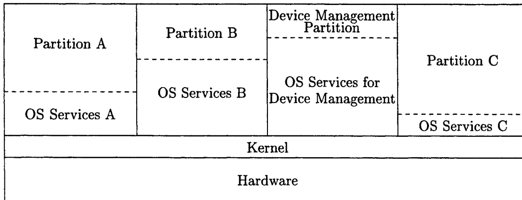
Figure 3.1: Different Operating System Software for Different Partitions
