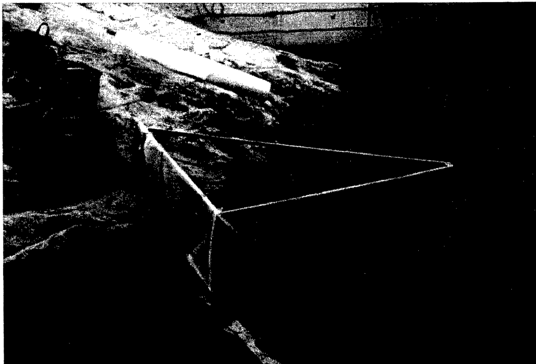
Figure 6-4. Transverse contraction joint construction with plastic-wrapped joint form
