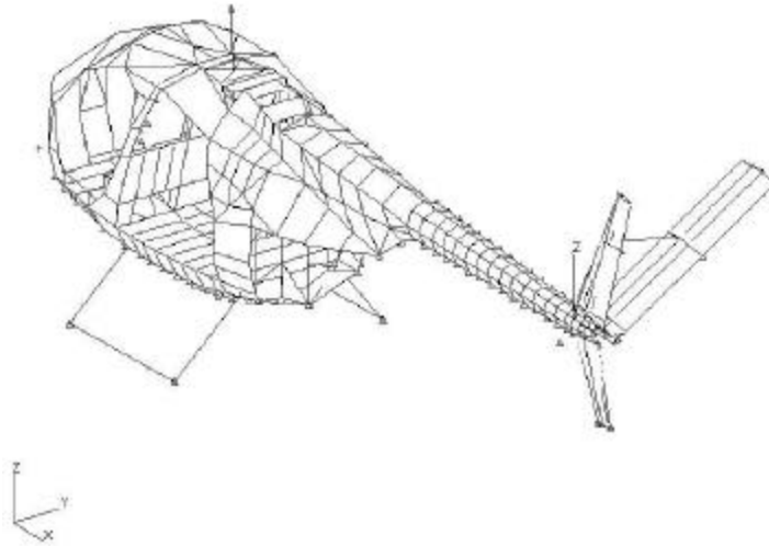
Figure 26: NPS NASTRAN Model
