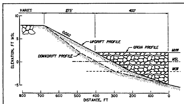
Figure C-6. Groin profile and expected beach profiles after the construction of groins at Ocean City, NJ
