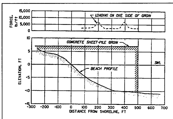
Figure 3-6. Loading diagram, cnoidal waves running along a cantilevered sheet-pile groin (Weggel 1981)
