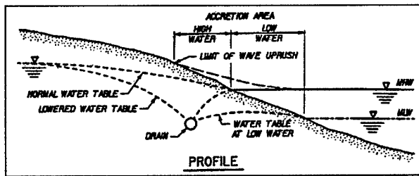
Figure 2-8. Beach dewatering system--lowered beach water table on beachface
