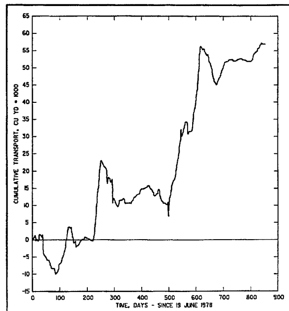
b. Cumulative longshore sand transport
