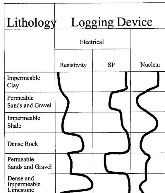
Figure 4-3. Conjunctive use of borehole geophysical logs
