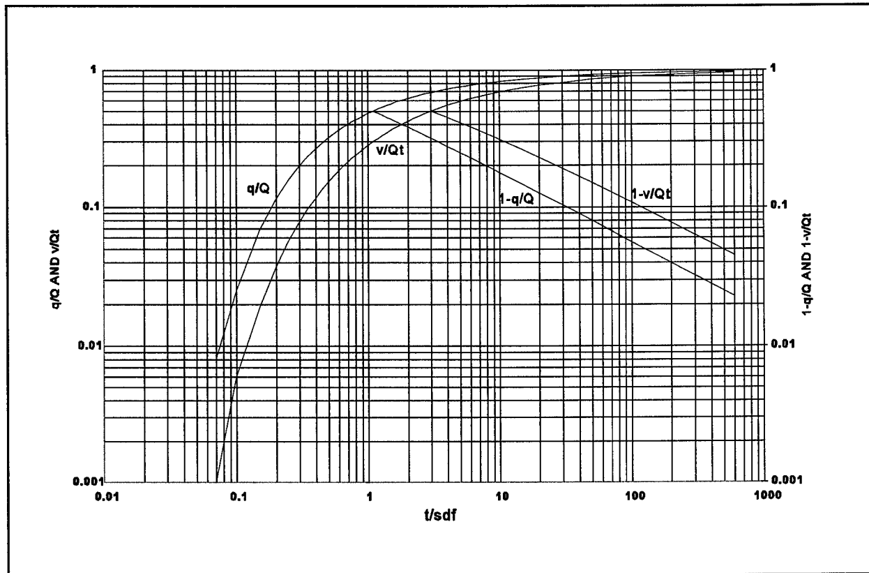
Figure 6-6. Curves to determine rate and volume of stream depletion (Jenkins 1968)
