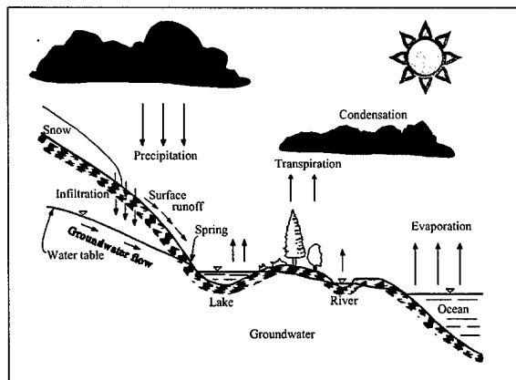
Figure 2-1. Hydrologic cycle
