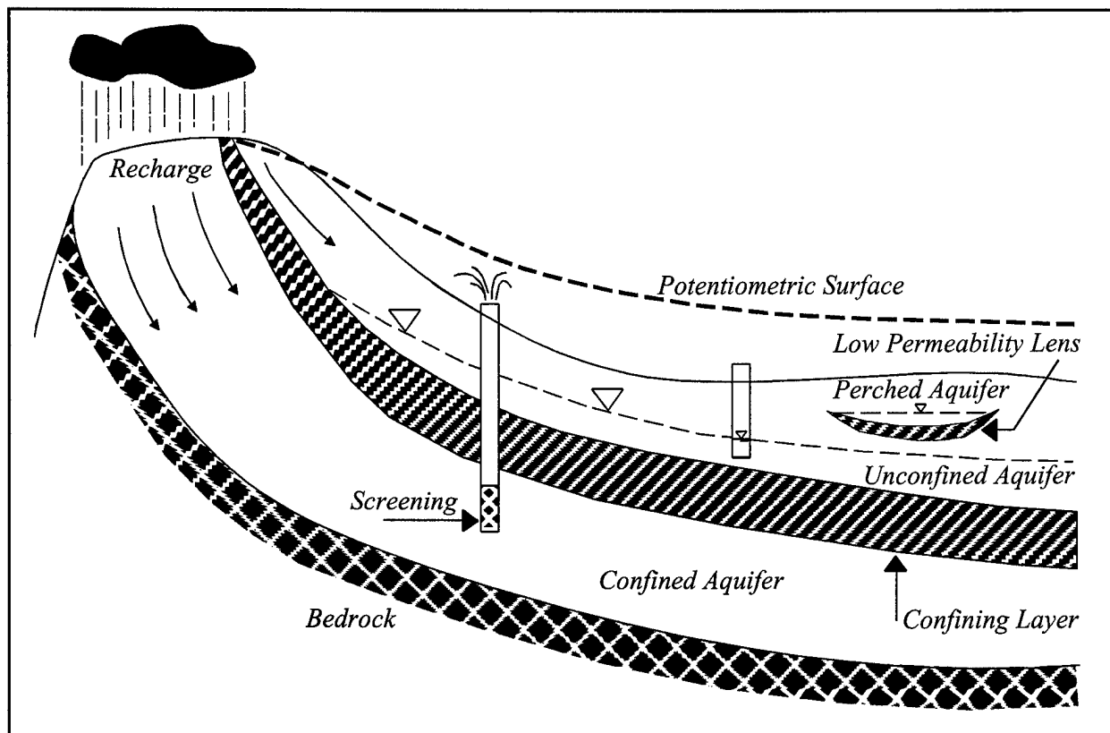
Figure 2-4. Aquifer formations
