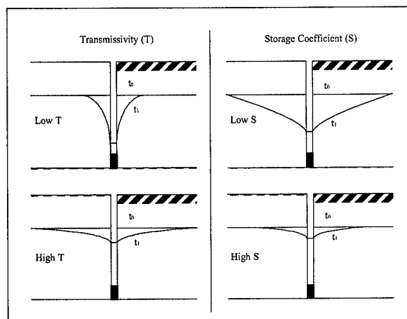
Figure 4-2. Influence of transmissivity and storage coefficients on cone of depression for similar aquifers at a constant pumping rate
