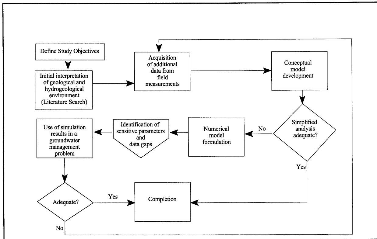
Figure 3-1. General flow diagram for characterizing a groundwater flow system for a management decision-making process
