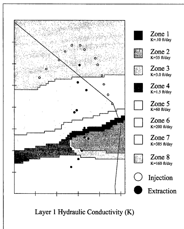
Figure 15. Hydraulic Conductivity Zones, Layer 1
