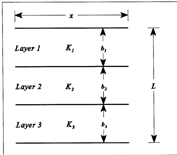
Figure 2-7. Stratified media
