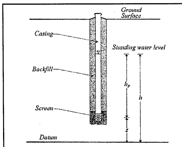
Figure 2-3. Relationship between hydraulic head, pressure head, and elevation head within a well
