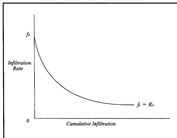
Figure 6-3. Infiltration capacity curve
