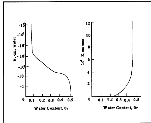
Figure 6-2. Typical relationship between moisture potential ( \psi ), hydraulic conductivity ( K ) and water content ( \theta_v ) for an identical clay sample
