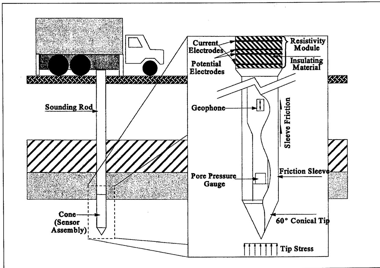
Figure 4-8. Components of cone penetrometer testing system
