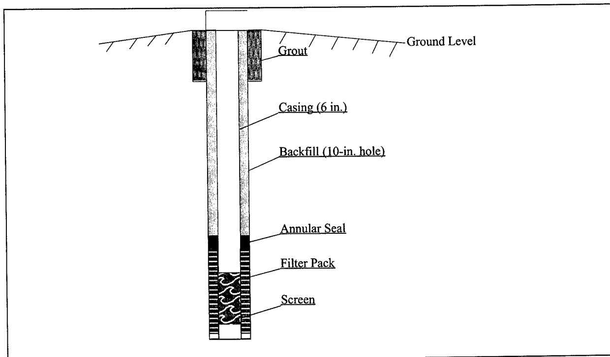
Figure 4-1. Basic well components
