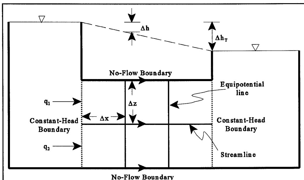
Figure 2-9. Basic flow net
