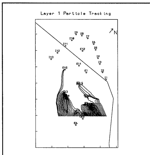
Figure 26. Particle tracking for optimization of plume removal, Layer 1
