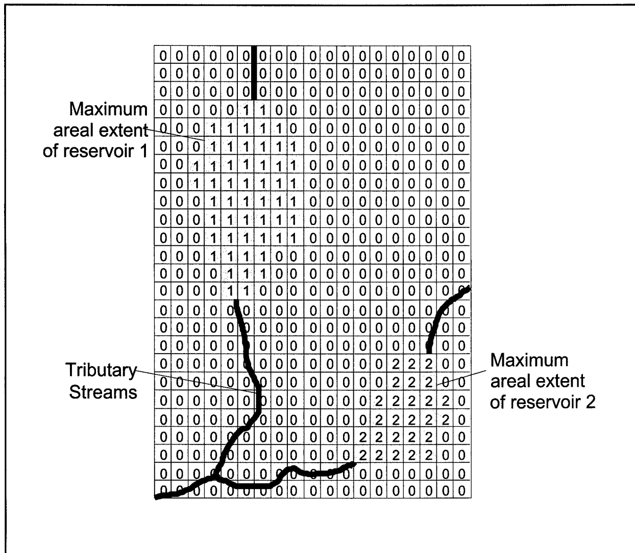
Figure 6-9. Definition of maximum areal extent of reservoir(s)
