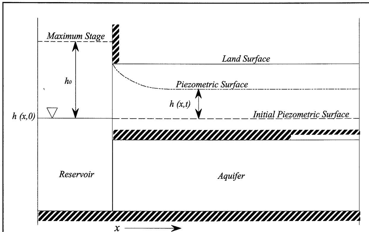
Figure 6-4. Representation of simplified one-dimensional flow as a function of surface-water stage
