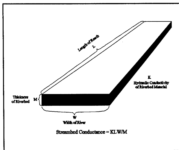
Figure 6-8. Determination of streambed conductance
