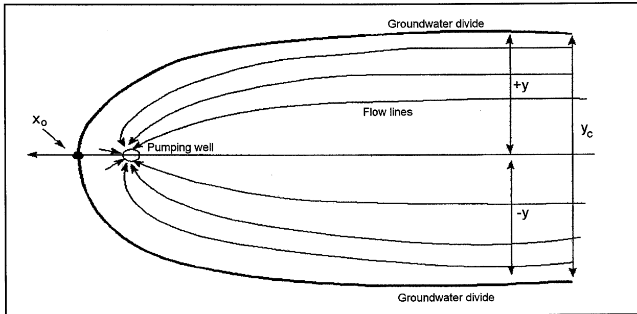
Figure 2-10. Capture zone of a pumping well in plan view. The well is located at the origin (0,0) of the x,y plane
