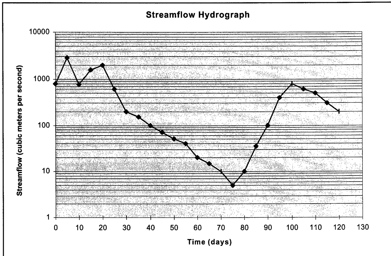
Figure 6-5. Hypothetical streamflow hydrograph
