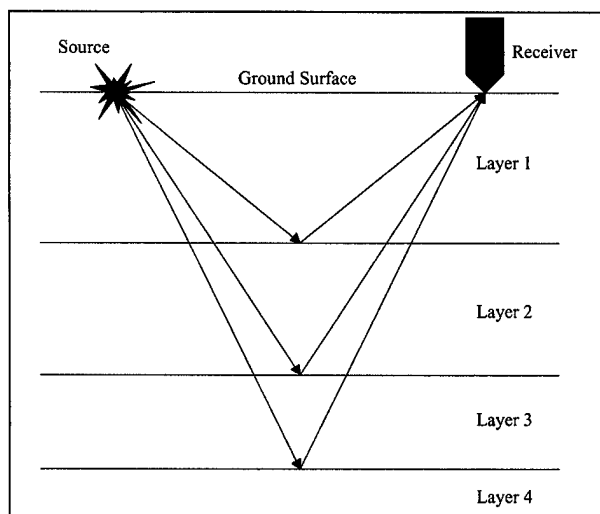
Figure 4-4. Reflected energy from three layers
