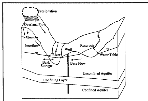
Figure 6-1. Flow components of the surface-groundwater system
