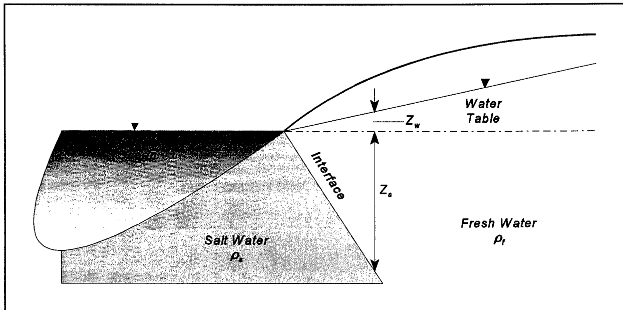
Figure 2-12. Saltwater-freshwater interface in an unconfined coastal aquifer
