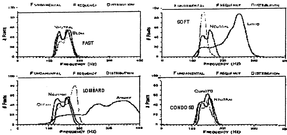
Figure 1: Distribution of fundamental frequency based on fundamental frequency estimates from neutral, angry, fast, slow, loud, soft, clear, Lombard effect, moderate (50%), and high (70%) (workload condition speaking styles.
