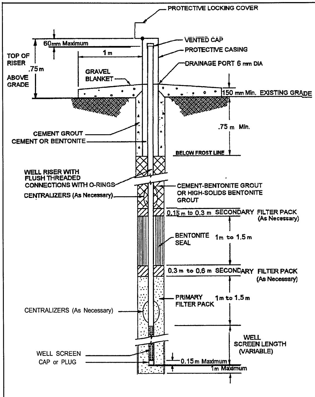
Figure 5-1. Schematic construction of single-cased well with gravel blanket
