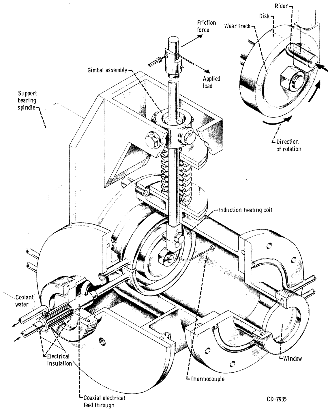
Figure 1. - High-temperature friction apparatus.
