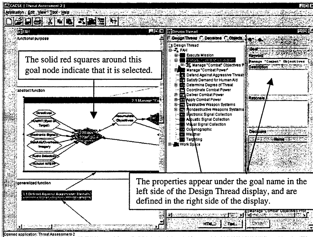
Properties of a Goal Node Shown in the Design Thread Window
