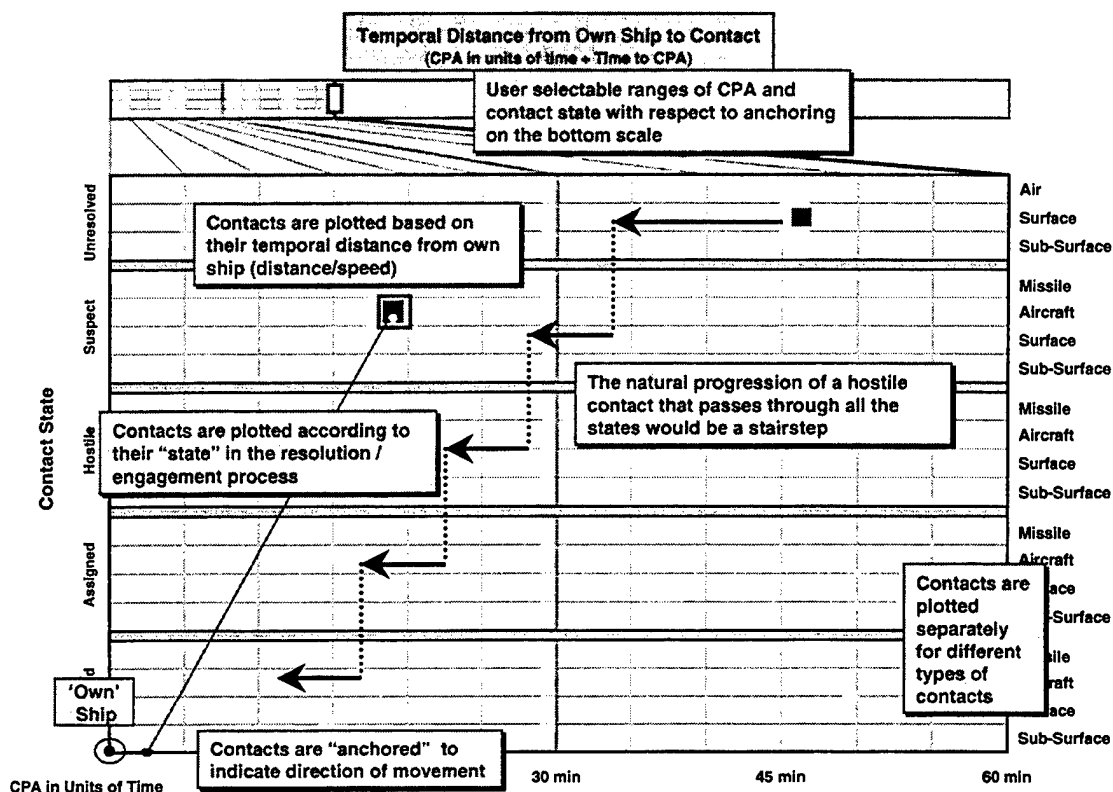
Figure 13. Annotations describing behavior of threat assessment visualization.
