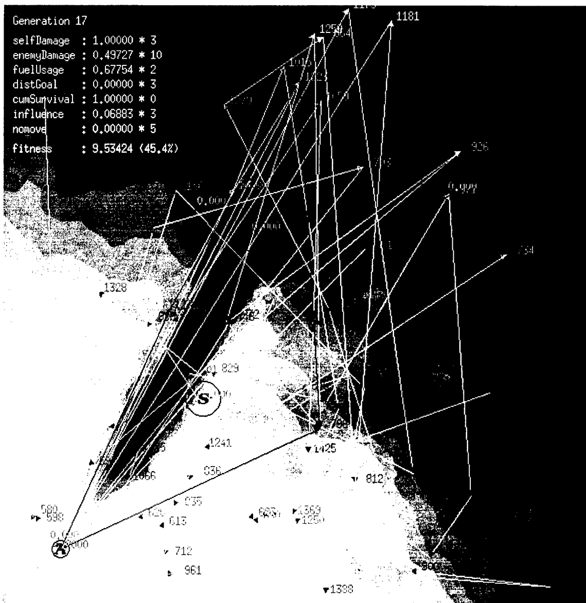
Figure 5. Evolved plans for basic scenario after 17 generations.
