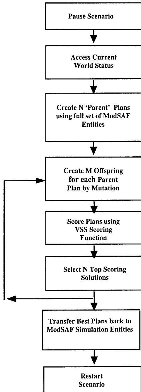
Figure 1. Flow diagram of EP / ModSAF processing.
