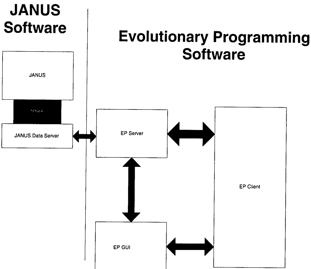
Figure 2. Processing diagram of EP / JANUS software system.
