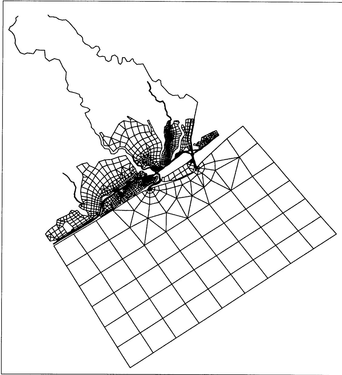
Figure 44. Numerical mesh
