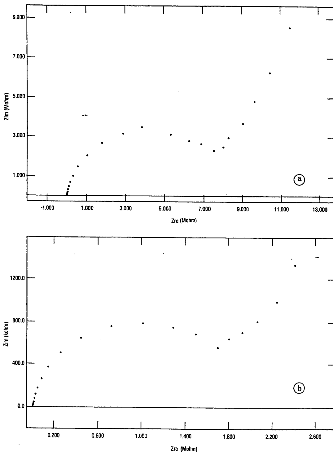
Figure 25. AC Impedance Spectra of PEO:LiCF 3 SO 3 (8:1)-MgO (10 wt%) Films (a) As-Prepared and (b) After Stretching. The Specimen was Not Subjected to Any Prior Heat Treatment
