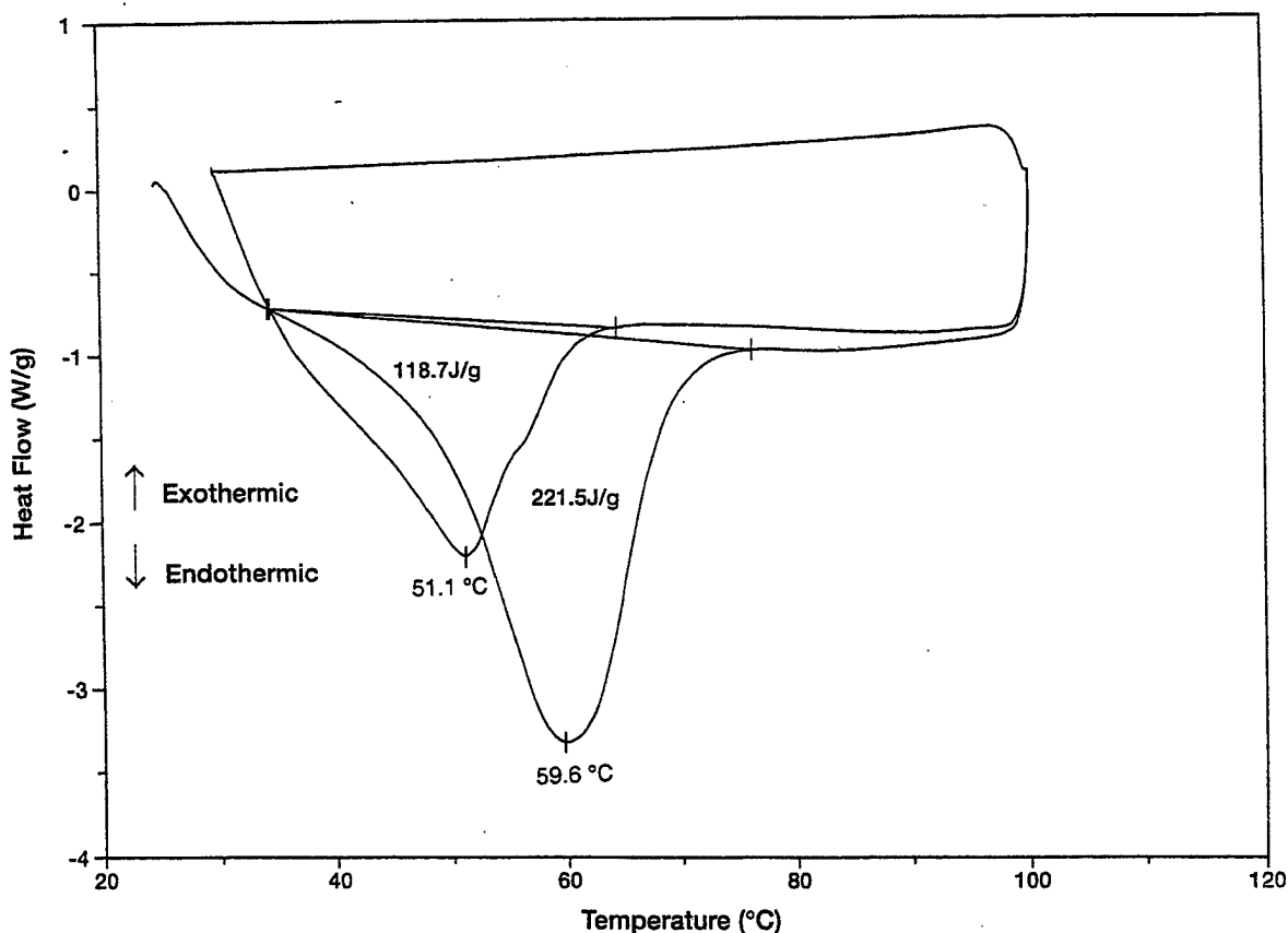
Figure 21. DSC Scans of \text{PEO}:\text{LiBF}_4 (8:1)- \text{Al}_2\text{O}_3 (20 wt%, 24 nm) Specimen
