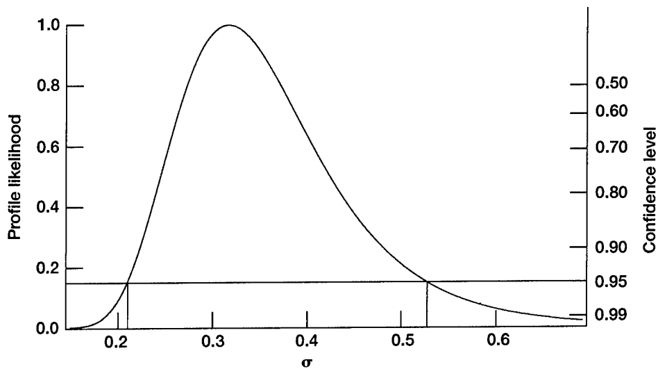
Figure 12.—Profile-likelihood method to determine confidence interval for shape parameter. Weibull shape parameter \beta = 1/\sigma . In the manner of figure 8.6 from Meeker and Escobar (1998).
