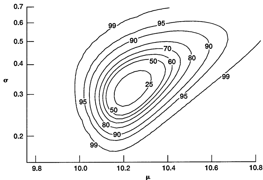
Figure 10.—Contours of equal joint confidence levels. Weibull shape parameter \beta = 1/\sigma and Weibull scale parameter \eta = \exp(\mu) . In the manner of figure 8.4 from Meeker and Escobar (1998).
