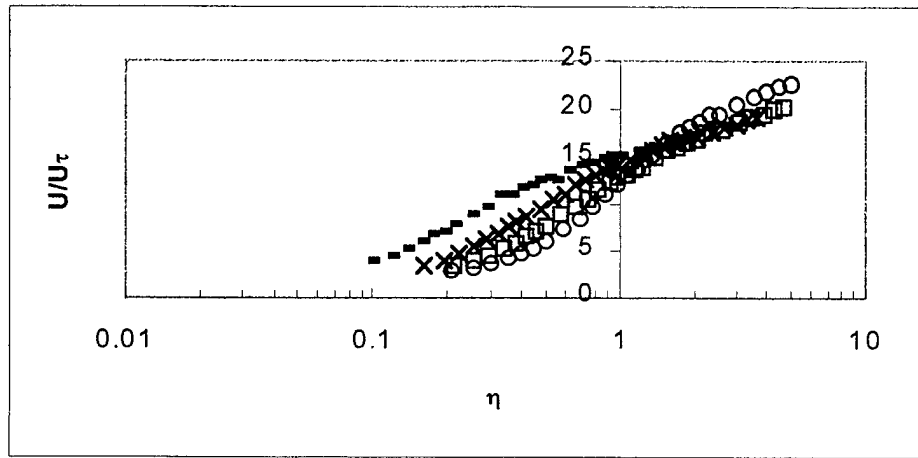
Figure 5. Stokes' Phase Variation of the Total Axial Velocity (Symbols: \bullet - 1 Hz; \times - 3 Hz; \square - 5 Hz; \circ - 7 Hz. Measurements are proposed by Choi et al. (reference 4).)
