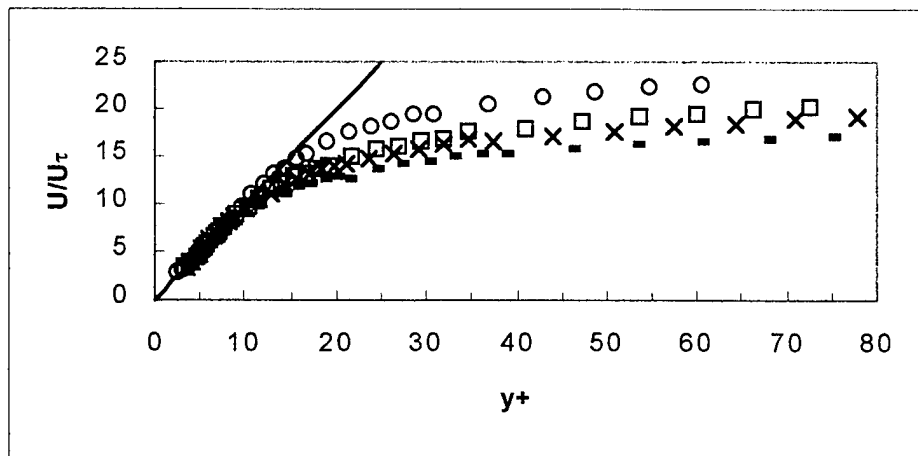
Figure 6. Total Axial Velocity in Normal Wall-Layer Velocity and Length Scales (Solid line is U^+ = y^+ . Symbols \bullet - 1 Hz; \times - 3 Hz; \square - 5 Hz; \circ - 7 Hz. Measurements are proposed by Choi et al. (reference 4).)
