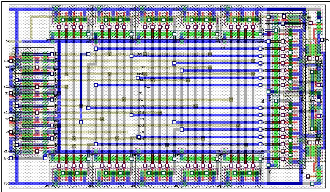
Figure 35. 4-Bit ALU Overflow.
