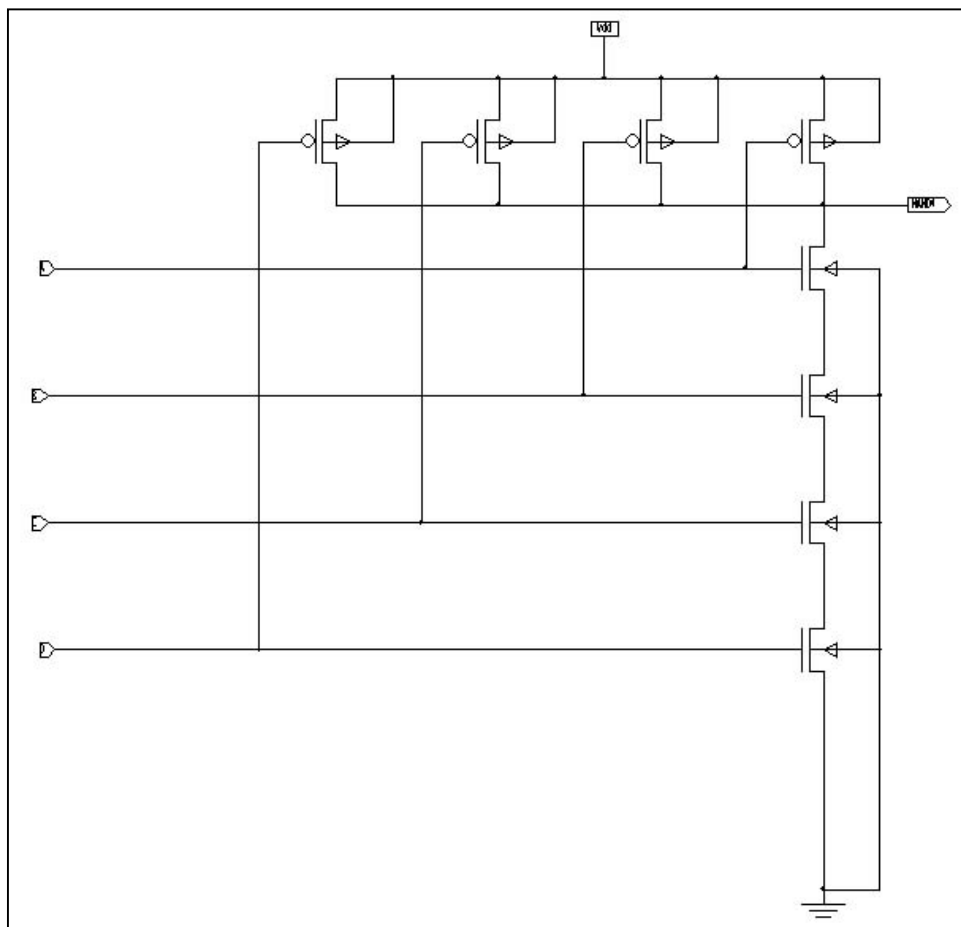
Figure 49. 4-Input NAND.
