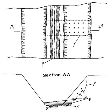
Figure 58. Formation of an earth-filled dam by means of nuclear explosions:
