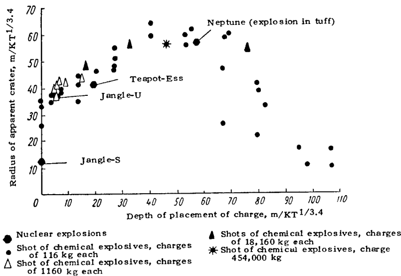
Figure 9. Dependence of the radius of the apparent crater upon the depth of placement of the charge, in alluvium, for nuclear and chemical explosives (reduced to a charge with a power of 1 KT).
