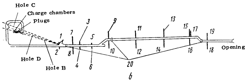
Figure 3. Placement of charge and plan of approach galleries in the Rainier shot.
