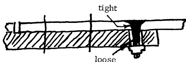
Figure 6.6 Interference Bolt Installation
