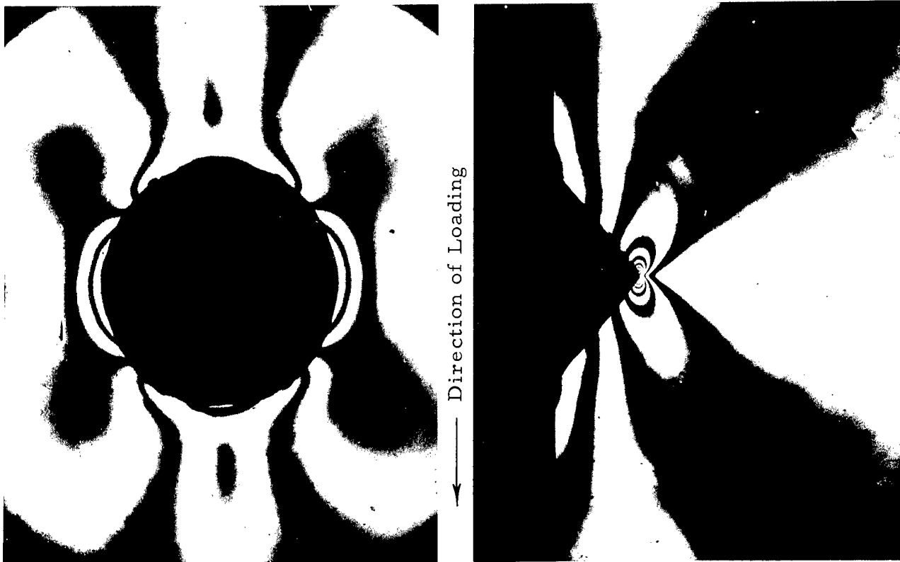
Figure 2.4 Photoelastic Models, Showing Stress at Edge of Hole and at V Notch
