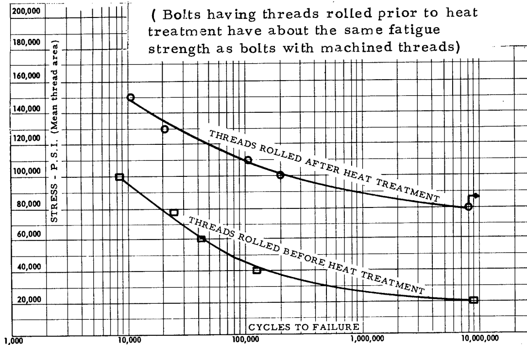
Figure 6.1 Thread Rolling
