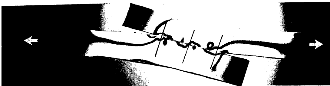
Figure 2.8. Simple Lap Joint -- Note Bending
