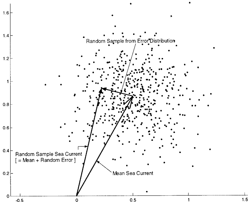
Figure 6-6. Obtaining a Sample Sea Current Vector.
