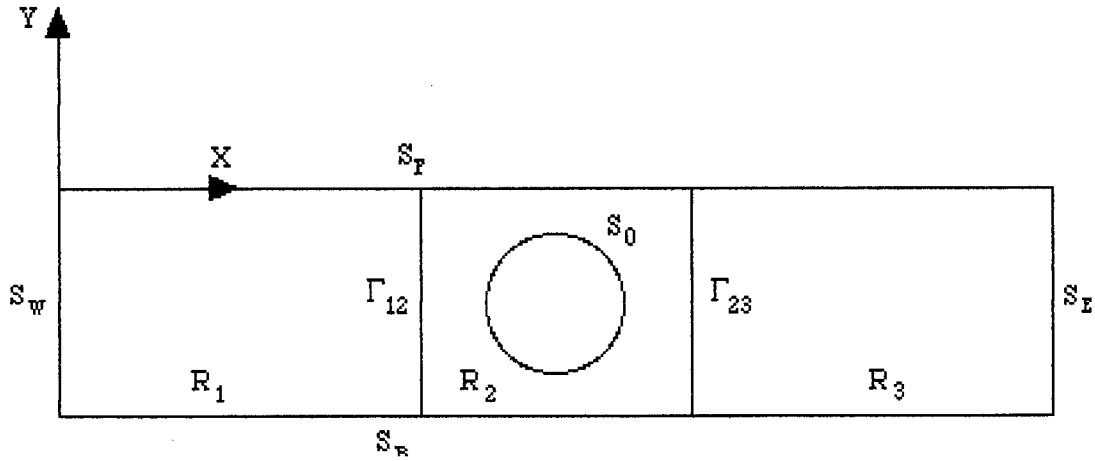
Figure 1 The coupled FEM and BEM computational domain
