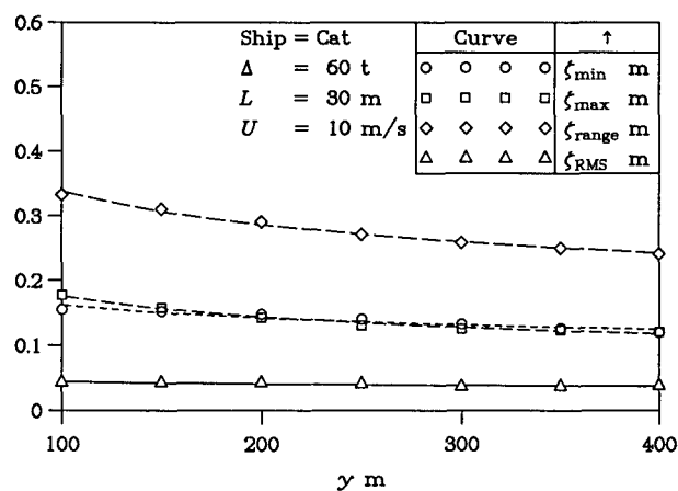
Figure 4: Curves of Wave Decay (b) Catamaran with a Length of 30 m
