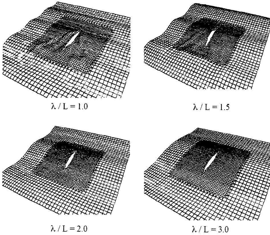
Fig.5 Wave Field around running ship hull
