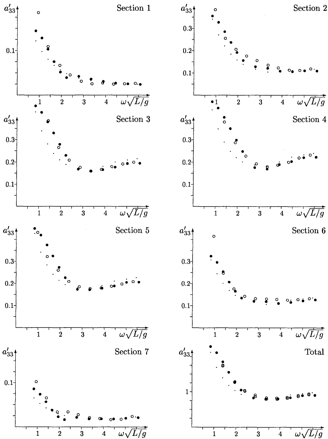
Fig.1: Series-60, C_B = 0.7 , F_n = 0 ; added mass; m = \nabla \cdot \rho a'_{33} = a_{33}/m for vertical force due to heave motion for strips and total ship; ○ Exp., ● GFM, · strip method
