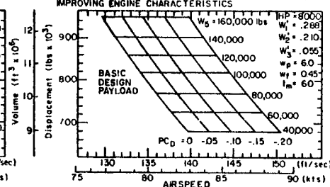
FIG. 4(d) ALL MAJOR TECHNOLOGY IMPROVEMENTS
