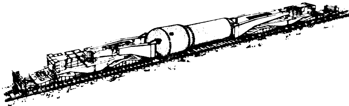
Figure 7: Nuclear component - Schnabel rail car of 800-ton capacity
