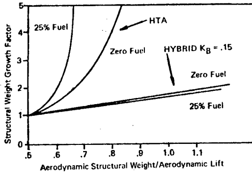
Figure 1 Structural Weight Growth for a Constant Payload
