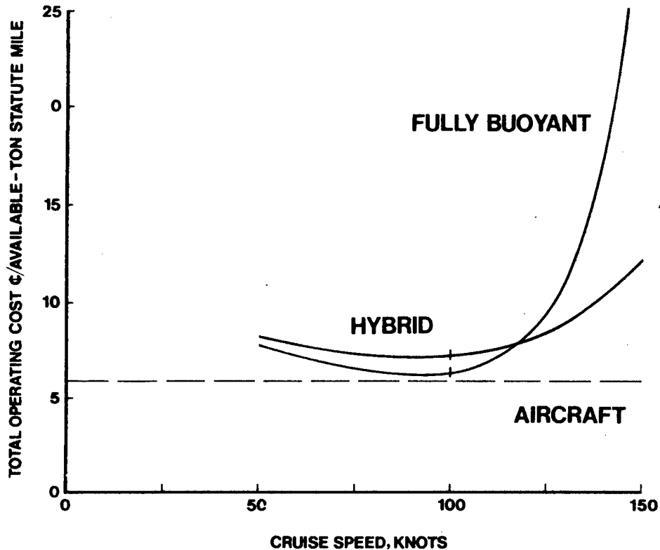
Figure 4 Effect of Cruise Speed
