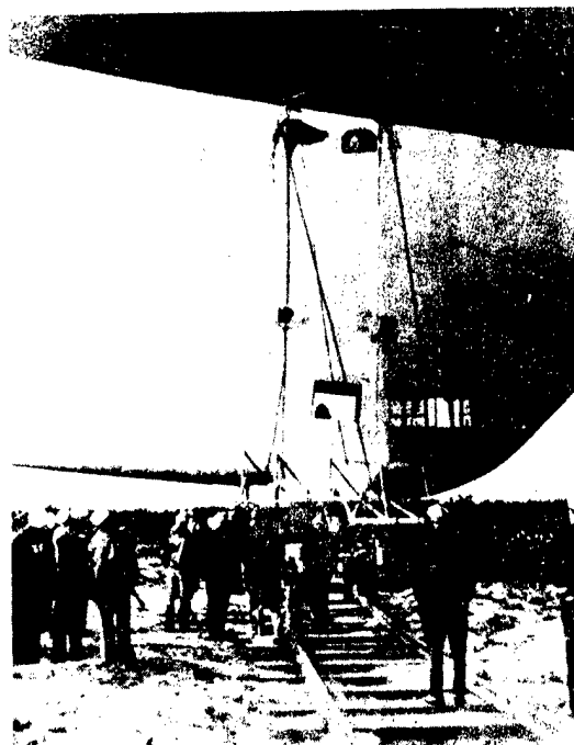
3. USS Akron lower fin moored at circle with rideout RR carriage and taxi-wheel. Lakehurst (~1932)
