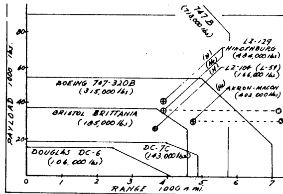
Figure 10. Range-Payload Comparisons
