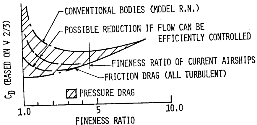
Figure 1 Pressure Drag Versus Fineness Ratio
