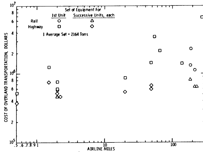
Figure 12: Cost of overland transportation of nuclear components
