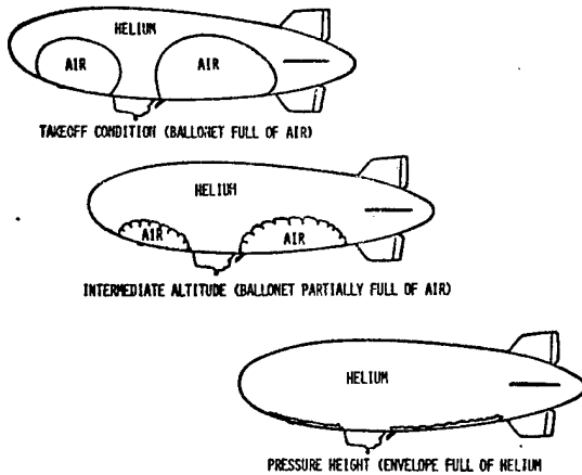
Figure 3 Airship Ballonet Operation During Flight
