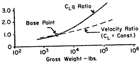
Figure 21 Size Effect on Hybrid Aircraft
