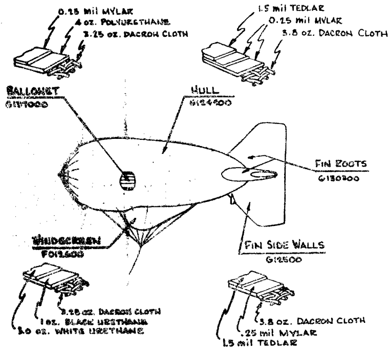
Figure D AEROSTAT MATERIALS
