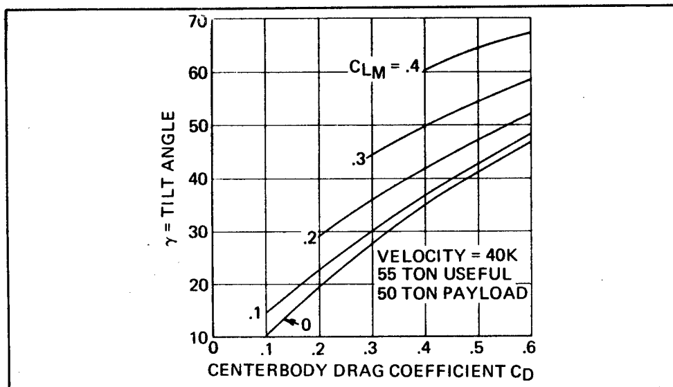
FIGURE 11. Aerocrane Skew Angle
