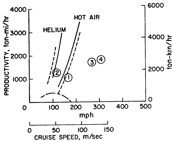
Figure 8 Productivity
