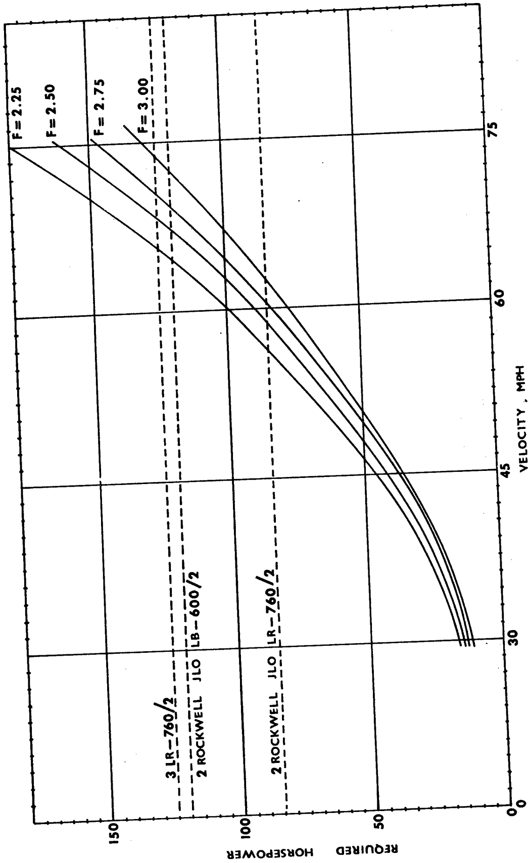
FIG. 2 REQUIRED ENGINE HP V. MAXIMUM VELOCITY VOLUME = 70,000 CUBIC FEET N=0.2 M=0.6
