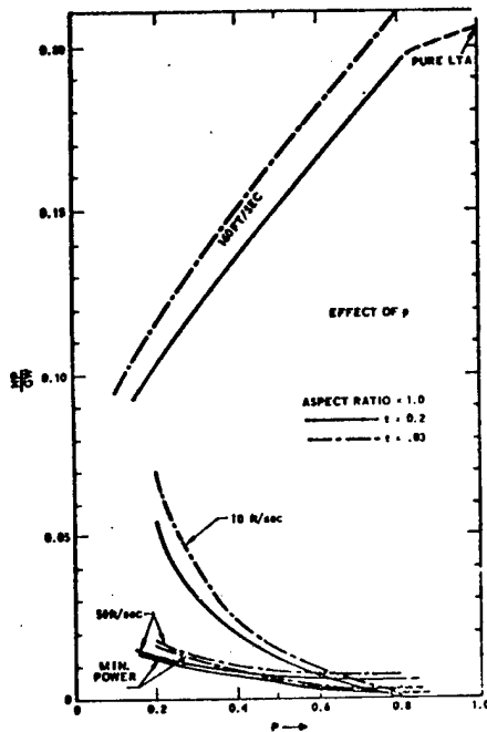
Figure 15 Effect of p
