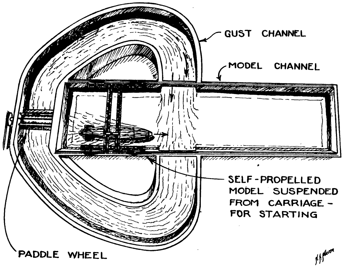
Sketch of Water Channel
