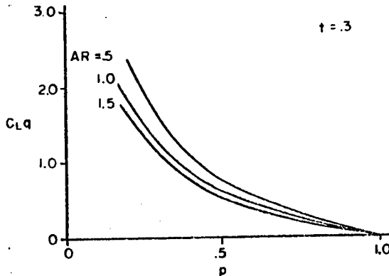
Figure 11 Hybrid Aircraft Dynamic Wing Loading
