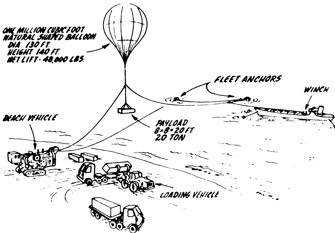
Ship-to-Shore TELTA Cargo Transfer System
