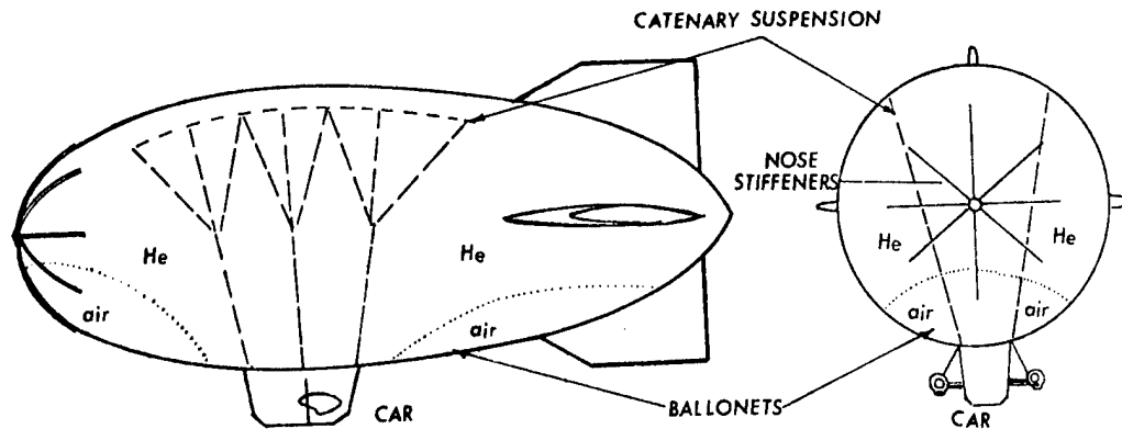
Fig 1 General arrangement of a non rigid pressure airship
