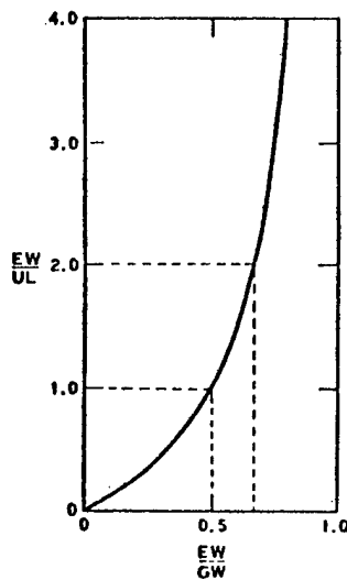
Figure 17 Empty wt/Useful Load Ratio
