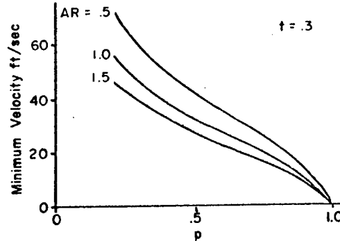
Figure 12 Hybrid Aircraft Minimum Flying Speed
