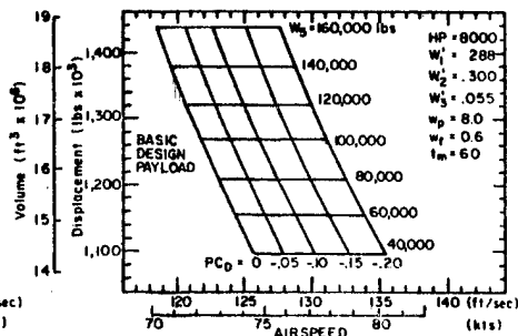
FIG. 4(b) REDUCING HULL DRAG, STRUCTURAL WEIGHT FRACTION, IMPROVING ENGINE CHARACTERISTICS
