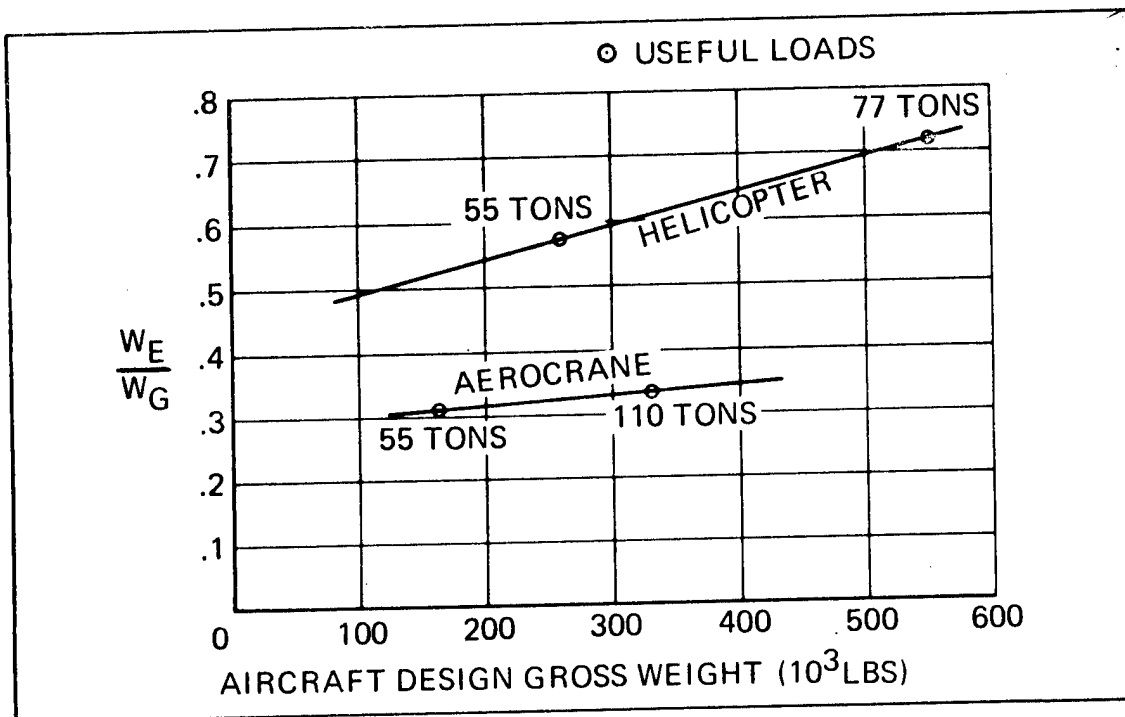
FIGURE 8. Aircraft Empty Weight Fraction
