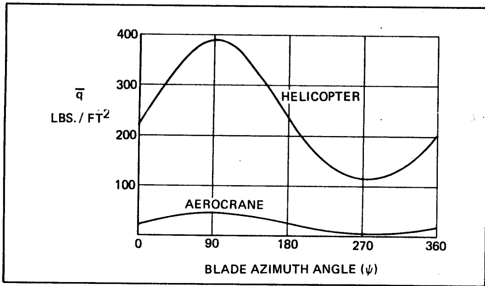
FIGURE 7. Blade Mean Dynamic Pressures
