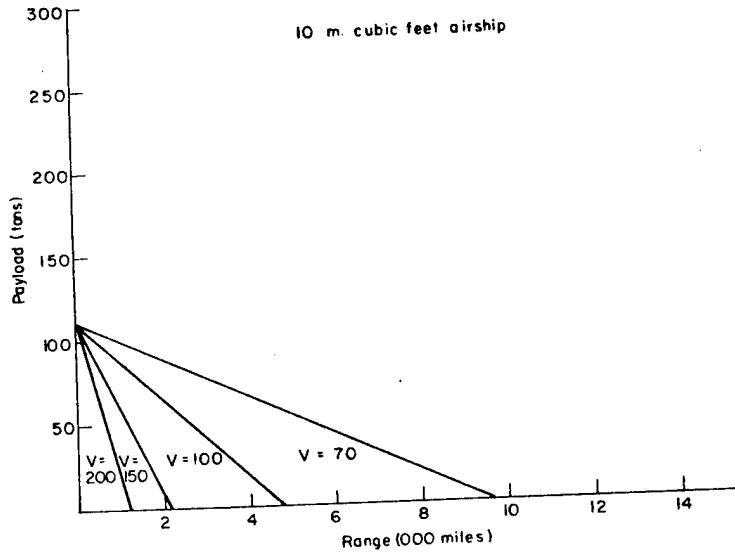
FIGURE 4 Payload vs. Range (10 m. cubic feet airship)
