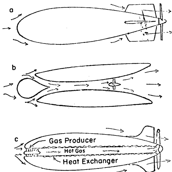
Figure 25 Aero/Propulsion Integration Systems for Dirigibles
