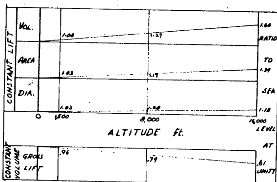
Figure 2. Static Effect of Altitude
