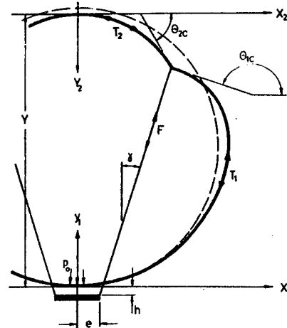
Fig 4 Twin Suspension Case
