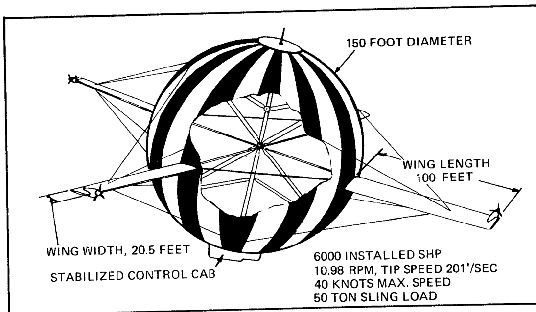
Figure 2. Aerocrane
