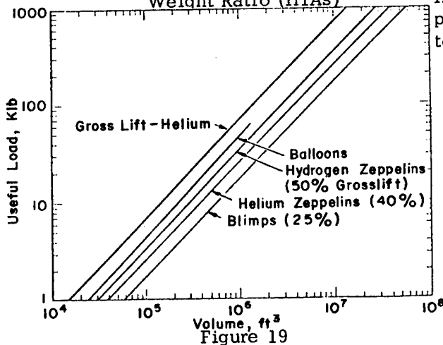
Useful Load Capabilities of LTA Craft
