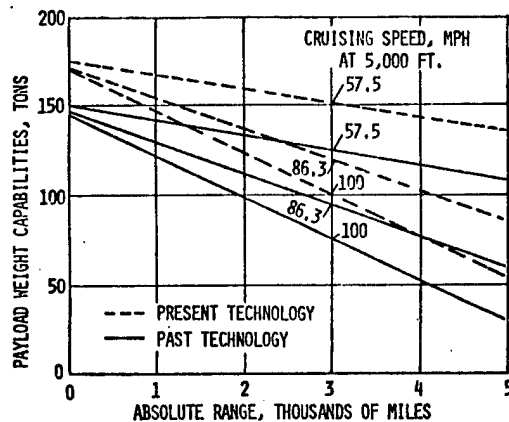
Figure 8 Payload Weight Capabilities Versus Range For 10 Million Cu. Ft. Airships At Different Cruising Speeds
