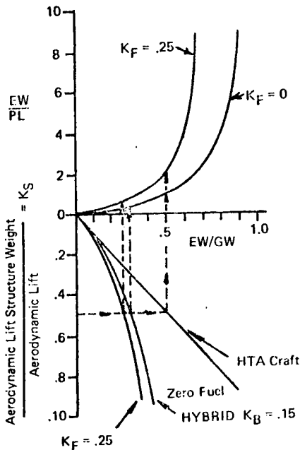
Figure 2. Structural Weight Comparisons HTAs vs HYBRIDS
