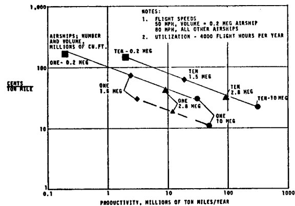
Figure 11 Effect Of Airship Size On Ton-Mile Costs
