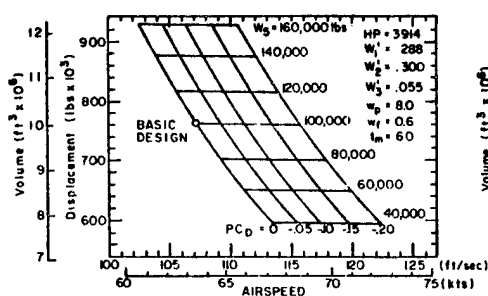
FIG. 4(a) REDUCING HULL DRAG ONLY
