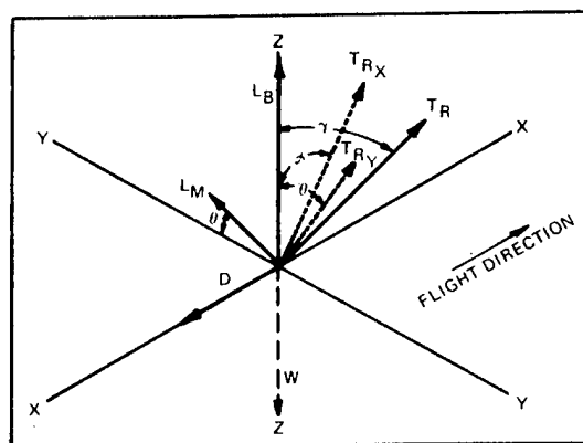
FIGURE 10. Free Body Diagram
