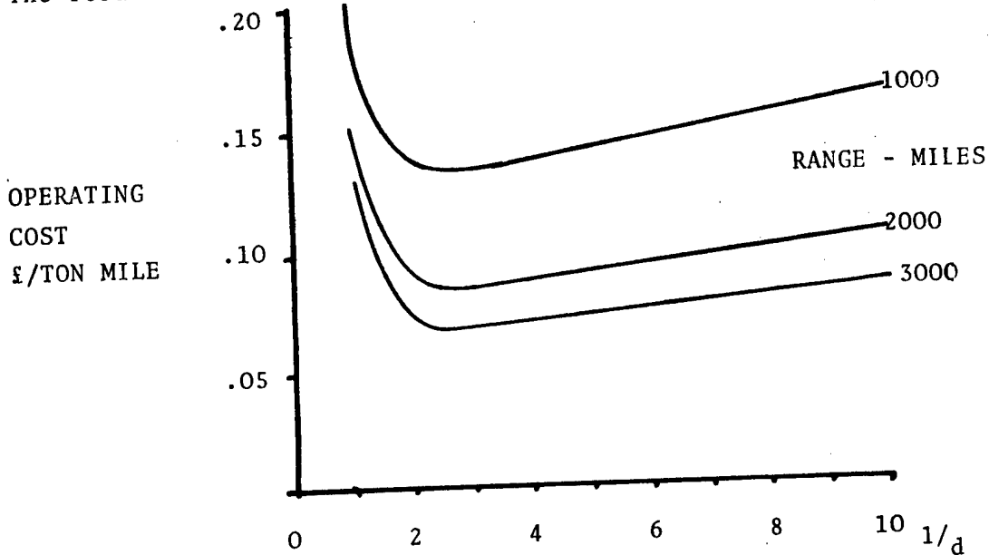
FIGURE 5 VARIATION OF LENGTH/DIAMETER
