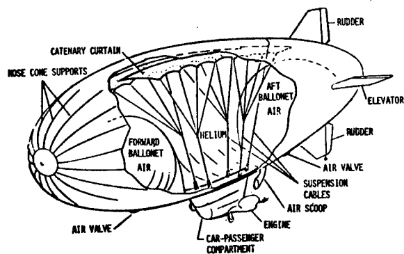
Figure 2 Typical Airship Design
