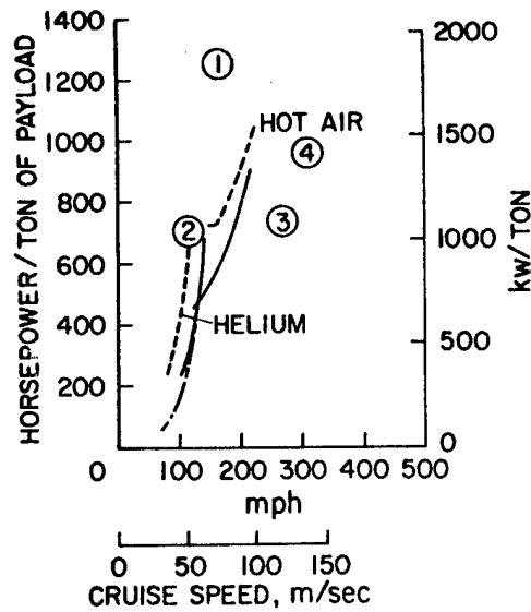
Figure 7 Power Requirements
