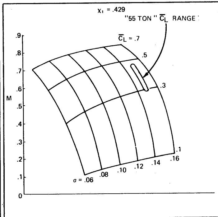
FIGURE 4. M vs Solidity and \bar{C}_L
