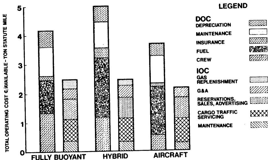
Figure 2 Operating Cost Comparison
