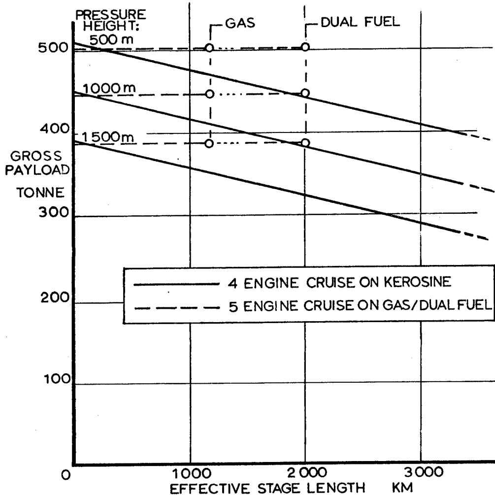
Fig. 2. PERFORMANCE OF AIRFLOAT HL AIRSHIP (ISA)
