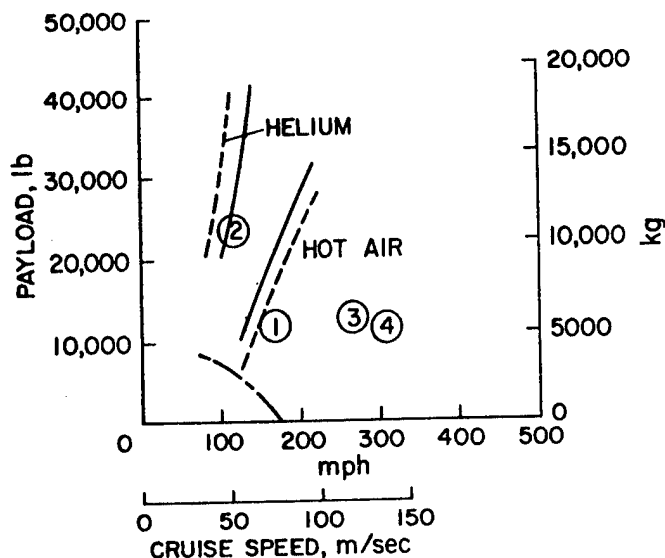
Figure 6 Payload Capability
