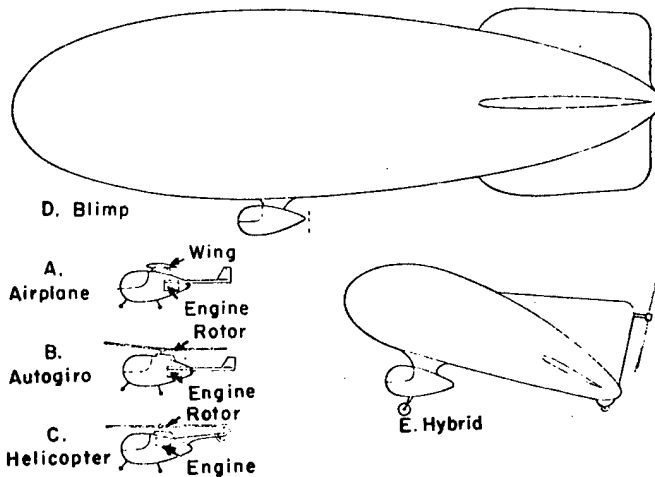
Figure 4 Generalized Aircraft
