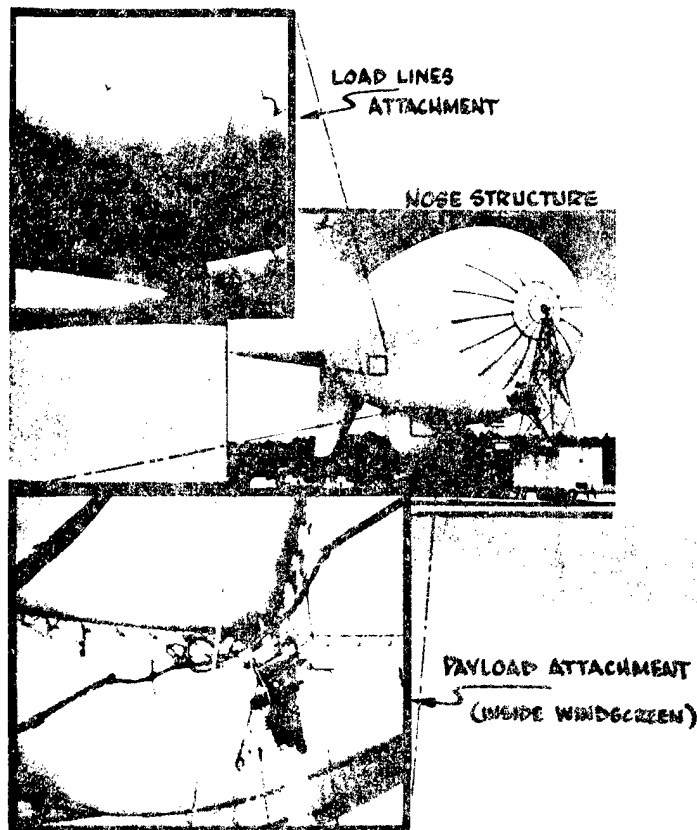
Figure G LOAD ATTACHMENT HARDWARE
