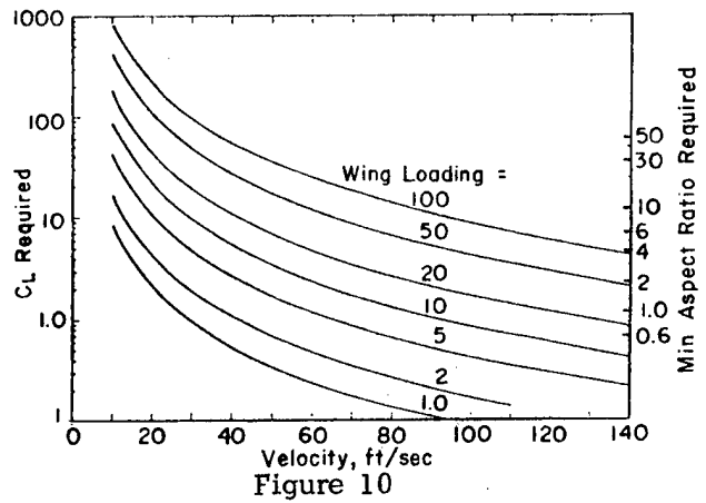
Figure 10 Wing Requirements for Low Speed Flight
