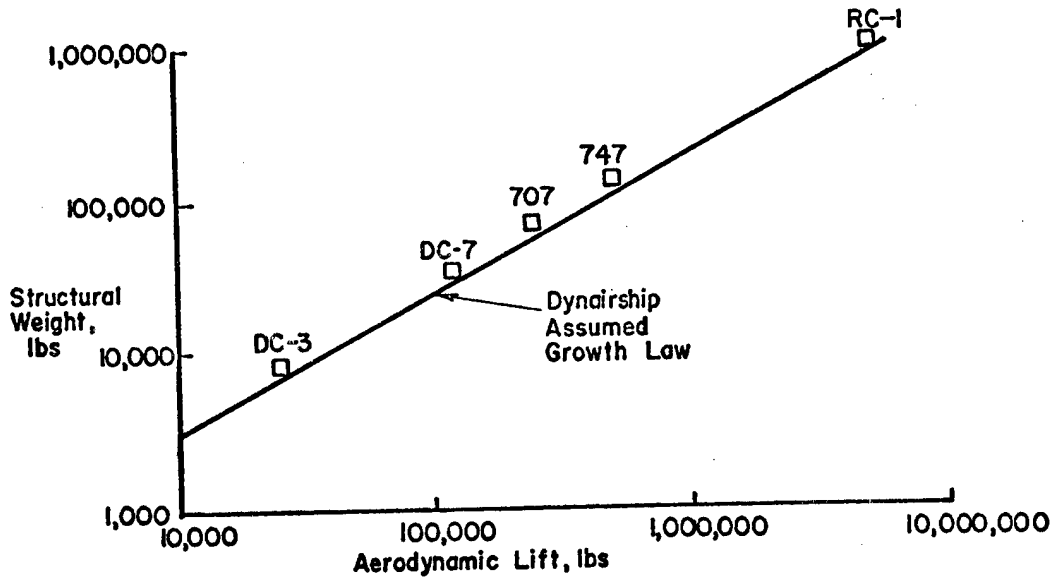
Figure 11. Structural Weight Growth Law
