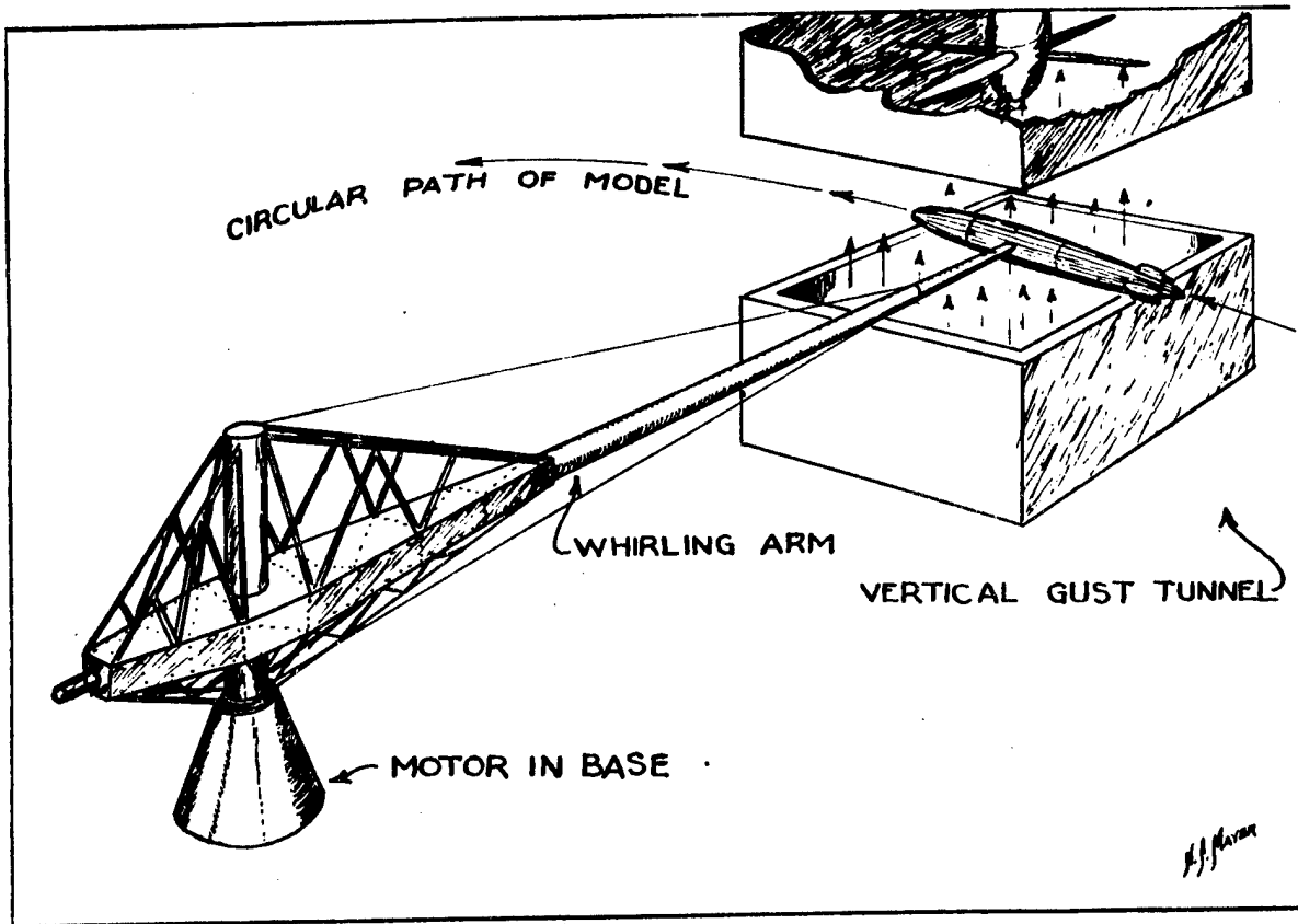
Sketch of Whirling Arm. Figure 3
