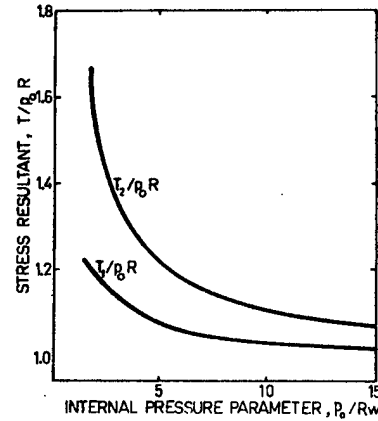
Fig 8 Stress Resultants, T/p_o R versus p_o/Rw for the case shown in Fig 4; e/R=0.2 , \gamma=15^\circ
