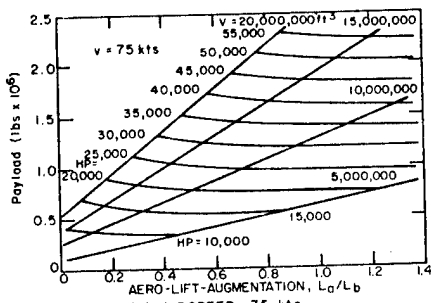
FIG. 7(a) AIRSPEED = 75 kts
