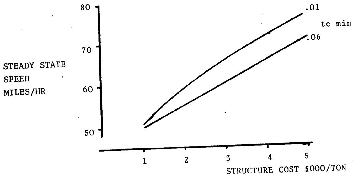
FIGURE 4 STEADY STATE SPEEDS
