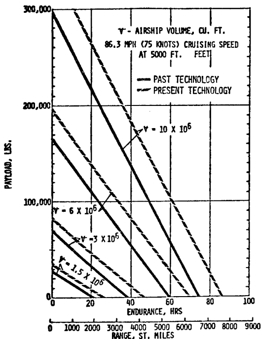
Figure 7 Payload Weight Capabilities Versus Range For Airships Cruising At 75 Knots
