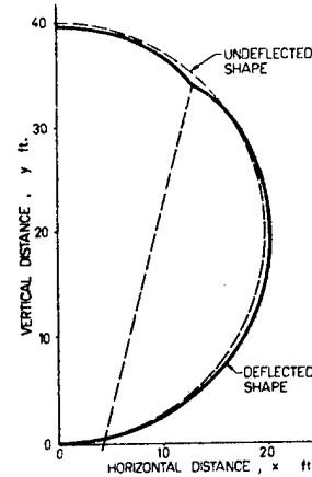
Fig 6 Cross-sectional Shape for an inflation pressure of 10 lbf/ft 2 for twin suspension
