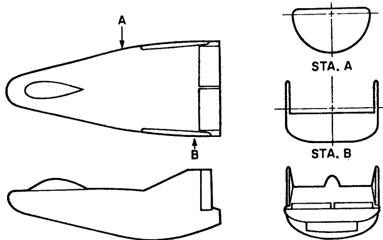
Figure 1 M2/F2 Lifting Body
