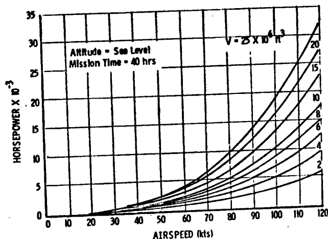
FIGURE 3. SIZING TRENDS OF CONVENTIONAL AIRSHIPS
