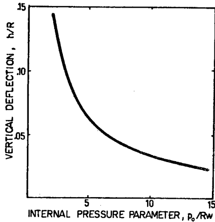
Fig 7 Suspension Deflection, h/R , versus p_o/Rw for the case shown in Fig 4; e/R=0.2 , \gamma=15^\circ
