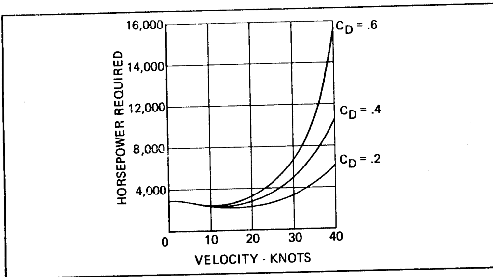
FIGURE 5. Installed Horsepower Required
