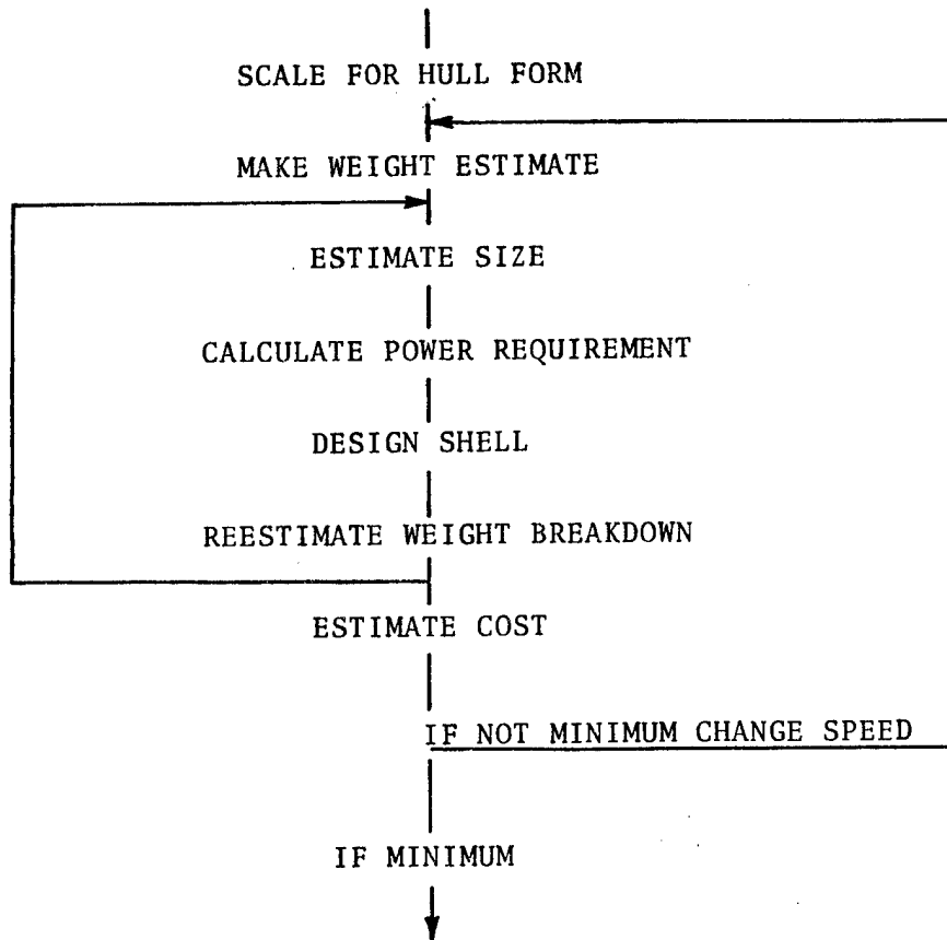
FIGURE 1 - MODEL STRUCTURE
