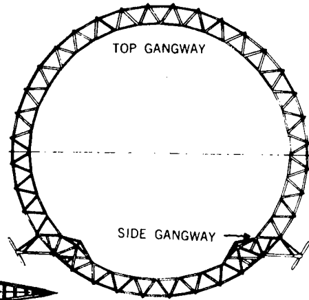
Figure 6b. Integrally Stiff
