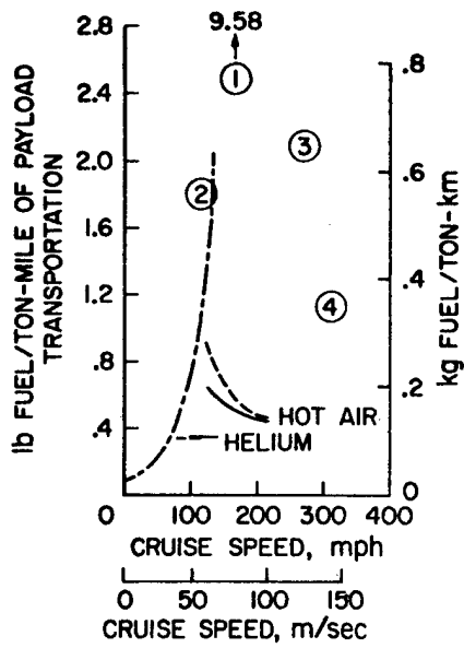
Figure 5 Fuel Consumption
