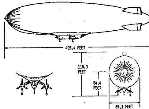
Figure 4 Goodyear ZPG-3W Airship
