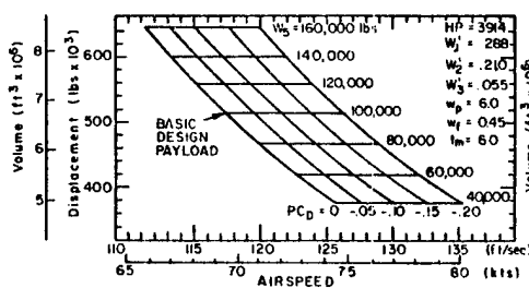
FIG. 4(c) REDUCING HULL DRAG, INCREASING POWER
