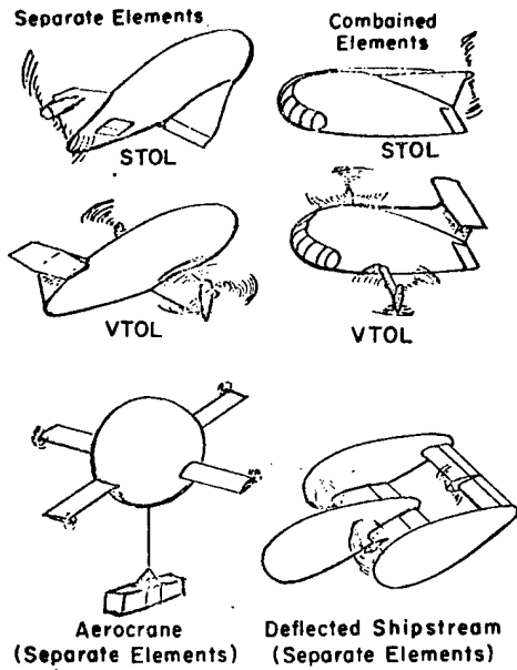
Figure 3 Hybrid Configurations
