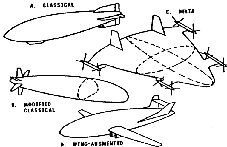
FIGURE 1. AIRSHIP DESIGN CONCEPTS: CONVENTIONAL TO HYBRID
