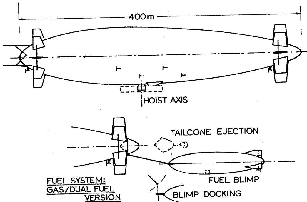
Fig.1. GENERAL ARRANGEMENT OF AIRFLOAT HL AIRSHIP
