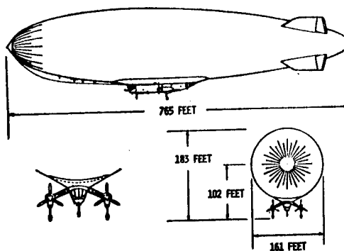
Figure 10 Typical 10 Million Cubic Feet Displacement Airship
