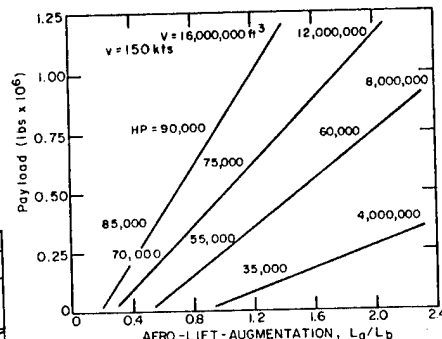
FIG. 7(c) AIRSPEED = 150 kts
