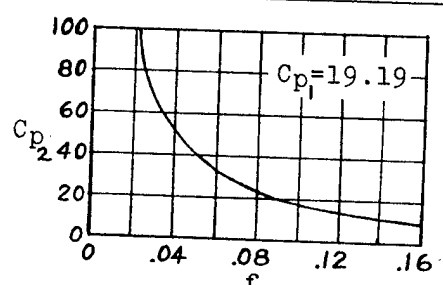
TRUNK FLATTENING VS TRUNK PRES. Figure 7
