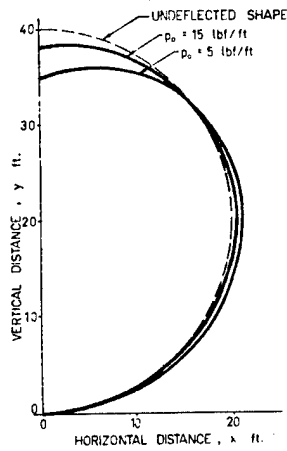
Fig 5 Cross-sectional Shapes for various inflation pressures for the central suspension case
