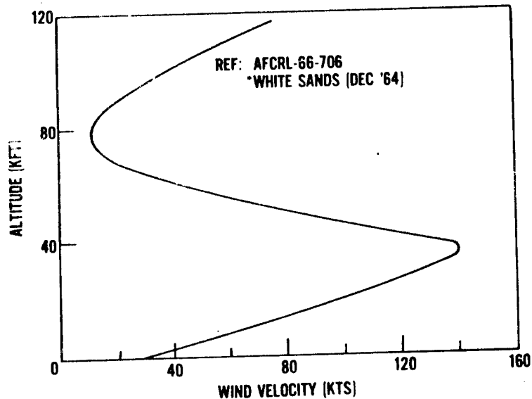
FIG. 1 TYPICAL WIND VELOCITY PROFILE
