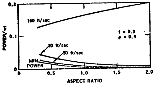
Figure 13 Effect of Aspect Ratio
