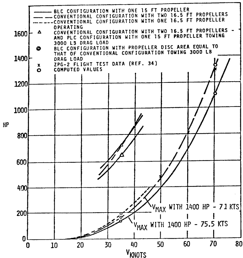
Figure 5 Horsepower Requirements vs Flight Velocity For BLC & Conventional Airships \Psi = 10^6
