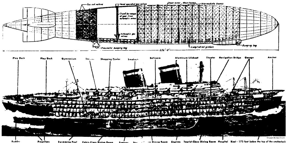
Figure 1. Ship and Airship cross-sections
