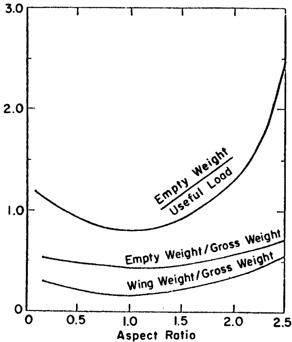
Figure 20 Typical Weight Characteristics of Hybrid Aircraft (Fixed 'Wing' - Combined Elements)
