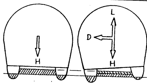
No Wind With Wind NAC ON WATER Figure 4A Figure 4B
