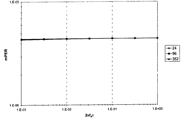
Figure 62: mPER results for different CPS-PP size (2 branch diversity).
