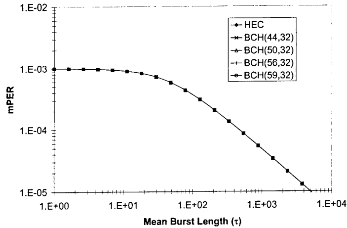
Figure 32: mPER results for BCH encoded ATM header.
