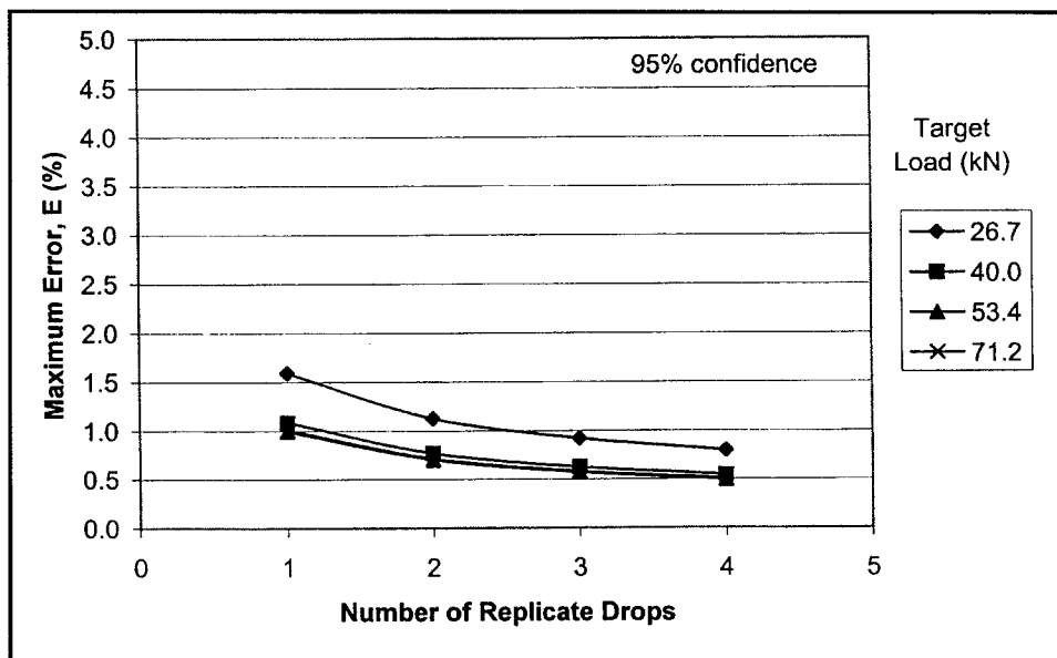
Figure B12. Maximum error for normalized deflection measurements (UT 1001; sensor offset = 203 mm)
