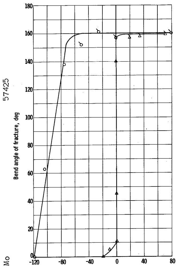
(a) 0.020-Inch-thick molybdenum sheet.
