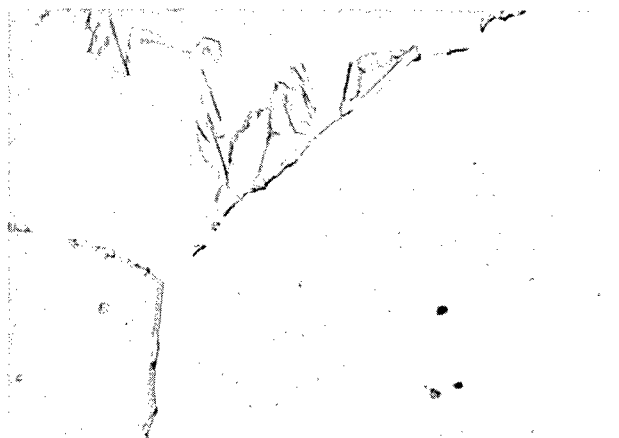
(d) 0.040-inch-thick molybdenum specimen annealed 66 minutes at 3500° F in 3 \times 10^{-5} -millimeter-mercury vacuum. X500.
