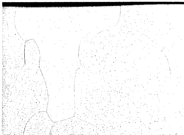
(g) Fused zone of 0.040-inch-thick molybdenum - 0.5-percent-titanium specimen welded at 7 inches per minute in helium atmosphere. X100.
