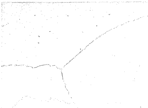
(i) 0.040-Inch-thick molybdenum - 0.5-percent-titanium specimen annealed 66 minutes at 3500° F in 3 \times 10^{-5} -millimeter-mercury vacuum. X500.
