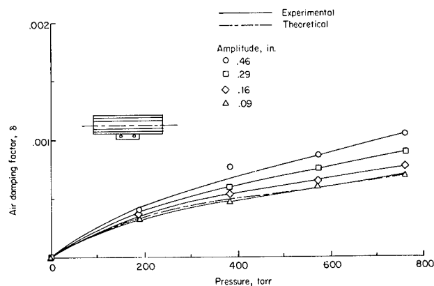
Figure 13.- Variation of air damping with pressure for the cylinder. f = 3.8 cps.
