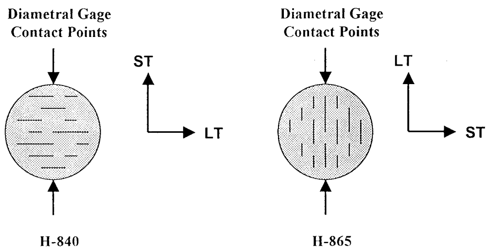
Figure 6. Grain Orientation With Respect To Strain Gage Placement for Two Hourglass Test Specimens
