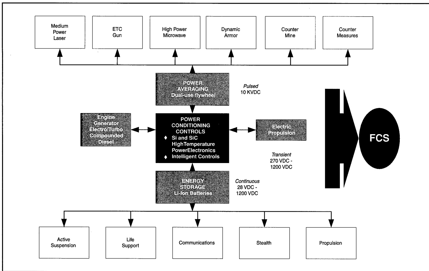
Figure 1: CHPS Concept
