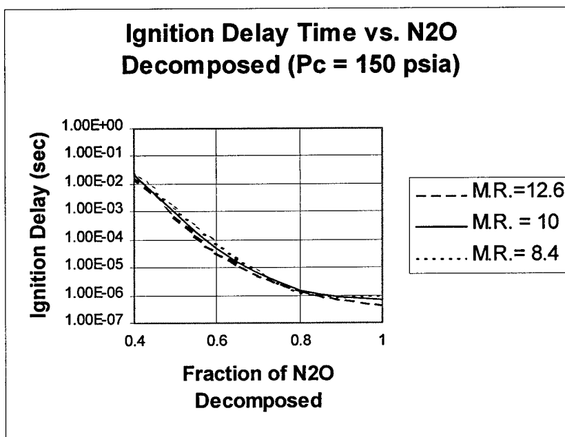
Figure 21: Ignition delay time versus fraction \text{N}_2\text{O} decomposed, for various M.R.'s.
