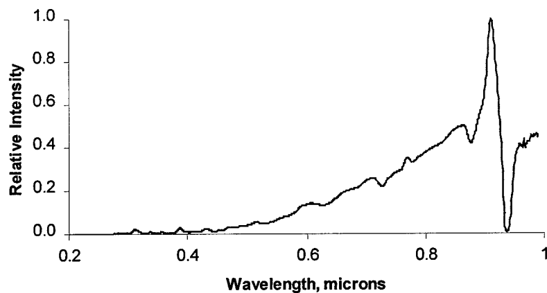
Figure 92: UV/VIS/NIR spectrum.
