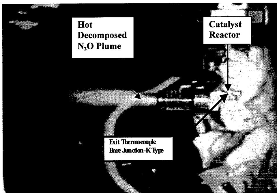
Figure 39: A hot flame of N 2 O decomposed gases is shown emanating from the exit of the atmospheric combustion catalytic igniter.
