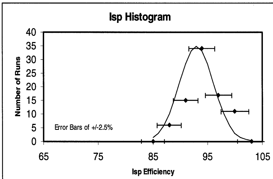
Chart 5. Illustrates a normal distribution of the Isp measurements around the average of 93% (of theoretical values).
