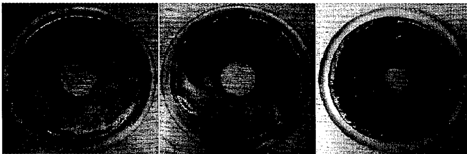
Figure 12. Progressive fuel grain patterning representing a) 8 seconds, b) 16 seconds and c) 24 seconds at an injection velocity of 7m/s and O 2 mass flow rate of 11g/s.
