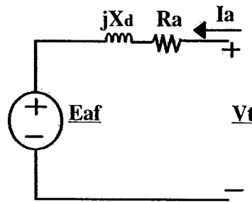
Figure 5-12: Equivalent circuit diagram for synchronous motor.
