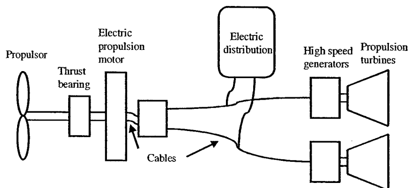
Figure 1-2: Electric drive schematic
