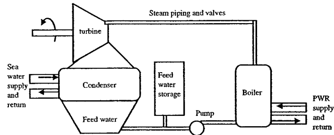
Figure 1-3: Rankine steam cycle.
