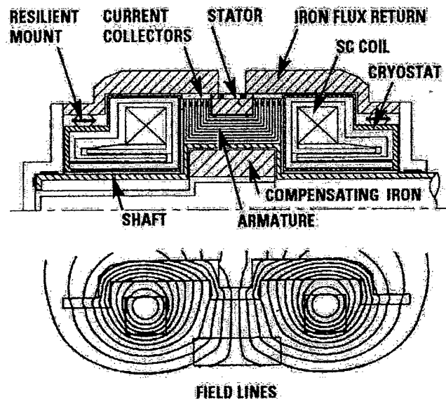
Figure 7-3: HPM cross section with flux path (courtesy of General Atomics)
