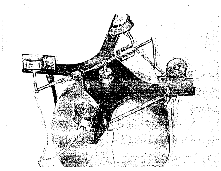
Figure 5: Cold Gas Propulsion Demonstration System
