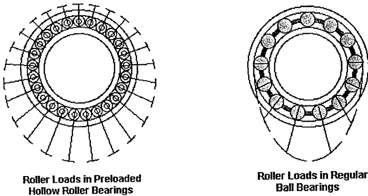
Fig 5: Comparison of Load Carrying Patterns
