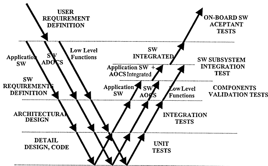
Fig. 3: “Spread-V” SW Life Cycle Model
