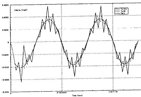
Fig 10: True anomaly time response
