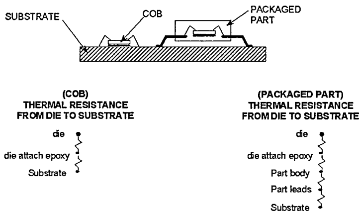
Fig. 4: Chip-on-Board Technology
