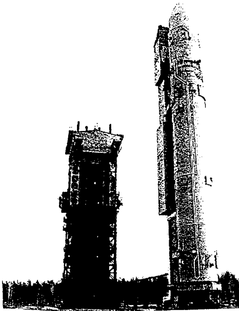
Fig. 13: Erected state
