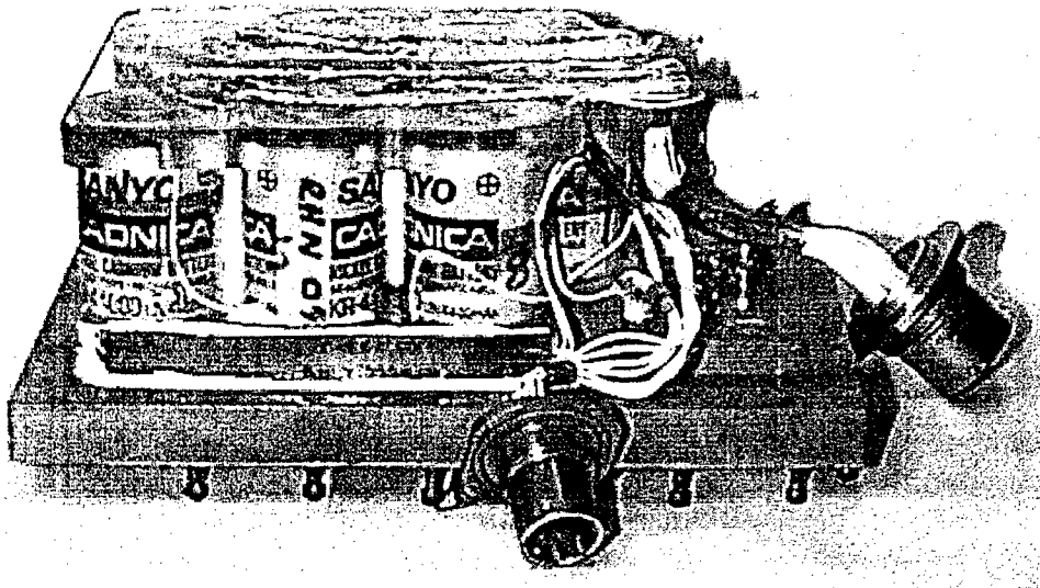
Fig 3: PANSAT Battery During Assembly
