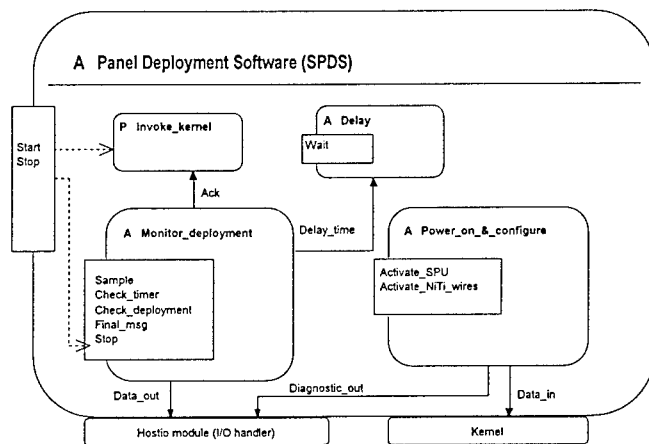
Fig. 8: HOOD Diagram of SPDS decomposition.
