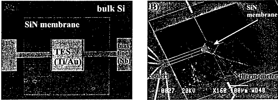
Figure 1: A) An optical microscope image of one of our x-ray detectors. The transition-edge sensor (TES) is 300 \mu\text{m} \times 300 \mu\text{m} in size and is fabricated on a silicon nitride membrane. B) An electron microscope image of a SINIS membrane cooler. The three coolers on the left draw heat from the membrane via normal-metal coldfingers and dump it into the bulk silicon. A SINIS structure in the middle of the membrane is used as a thermometer.
