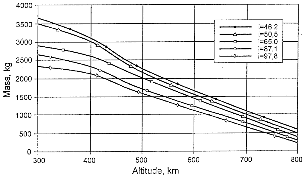
Figure 1. Dnepr-1 LV Performance Curves
