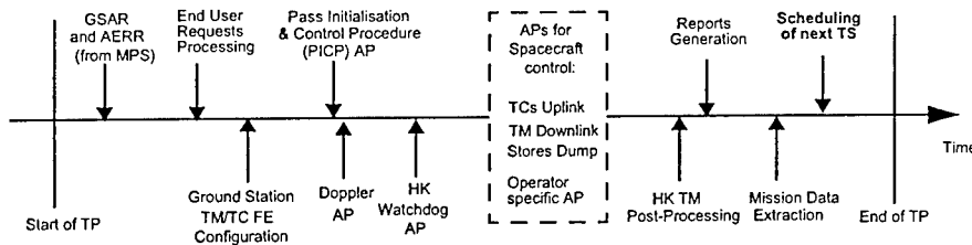
Fig 8: OAE Task Plan for the PROBA Mission
