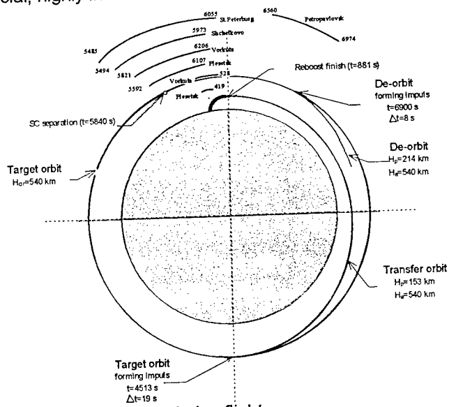
Figure 15: Radio visibility during flight
