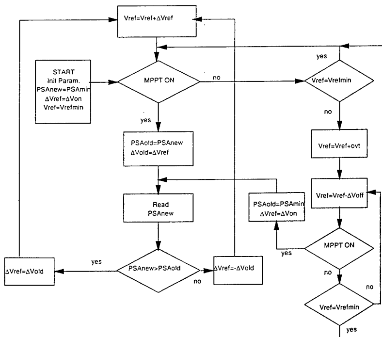
Fig.2: MPPT Algorithm
