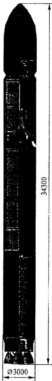
Fig 2. DNEPR LY GENERAL VIEW AND PRINCIPAL CHARACTERISTICS
