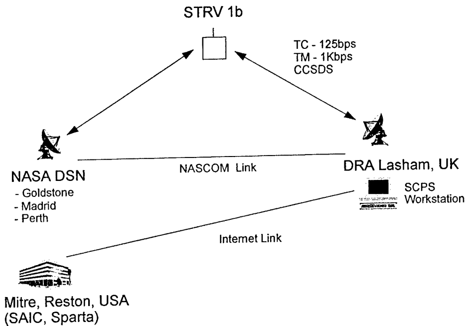
Figure 4. SCPS experiment arrangement.
