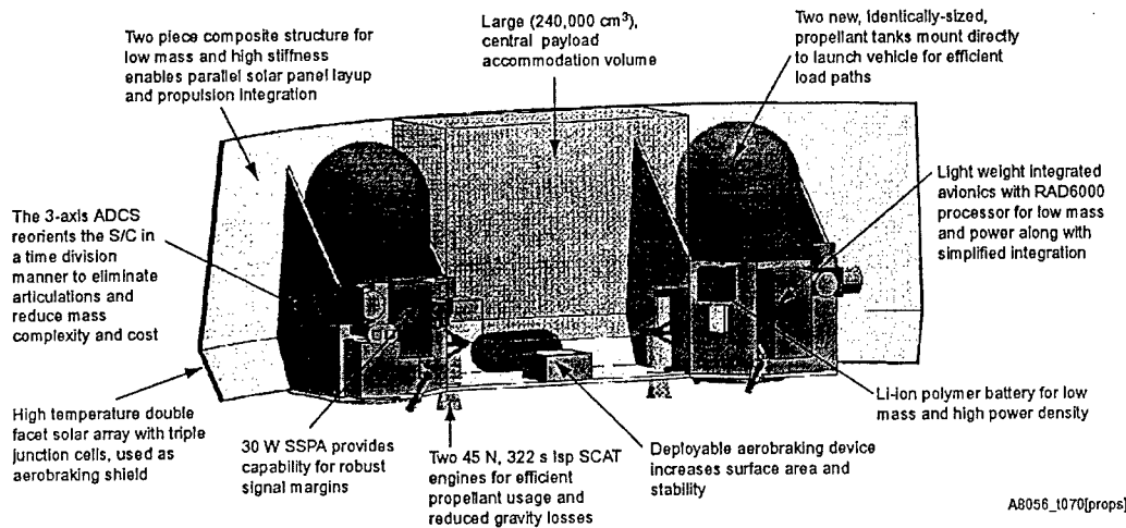
Figure 1. Key design features of the MSC bus.
