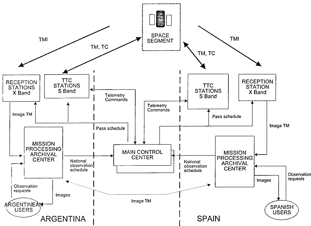
CESAR Ground Segment
