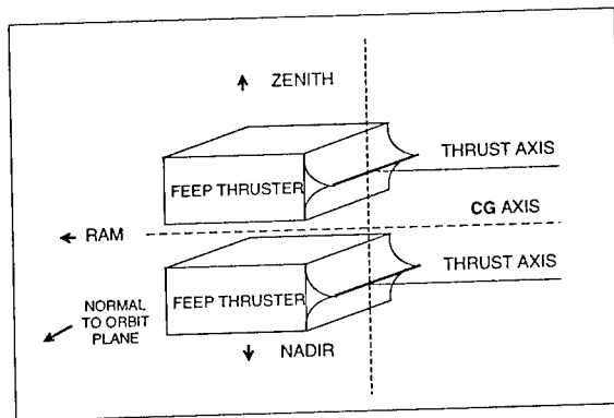
Fig. 4: FEEP thruster alignment with respect to a nadir pointing spacecraft axes.
