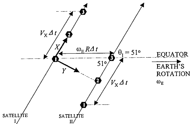
Figure 1: Picture of the same ground track formation as the satellites pass over the equator.
