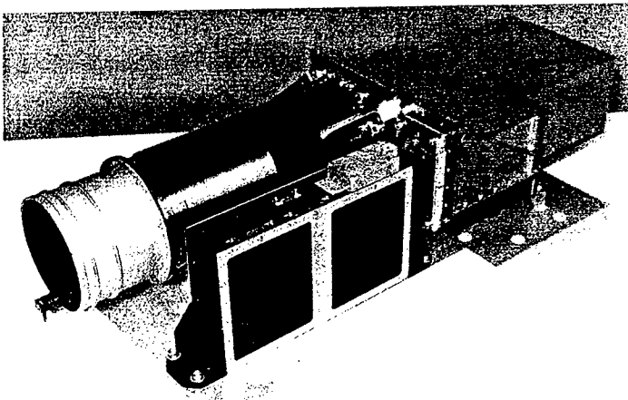
Figure 6: CHRIS instrument
