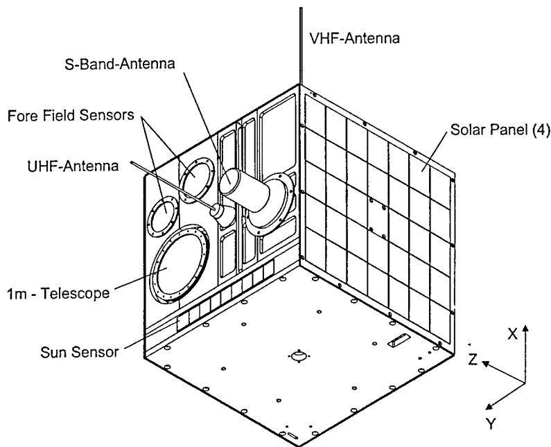
Figure 2: Microsatellite DLR-TUBSAT
