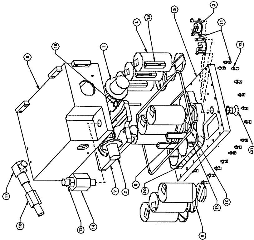
Fig 2: PANSAT Battery Housing Expanded View
