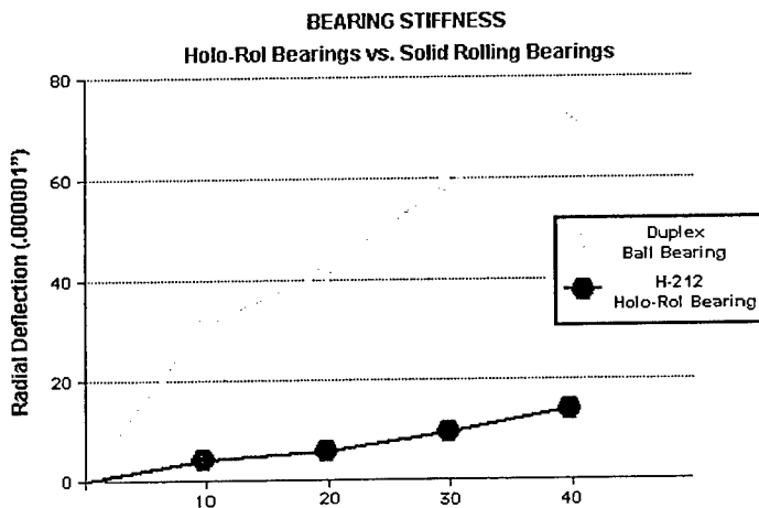
Fig. 4: Bearing Stiffness
