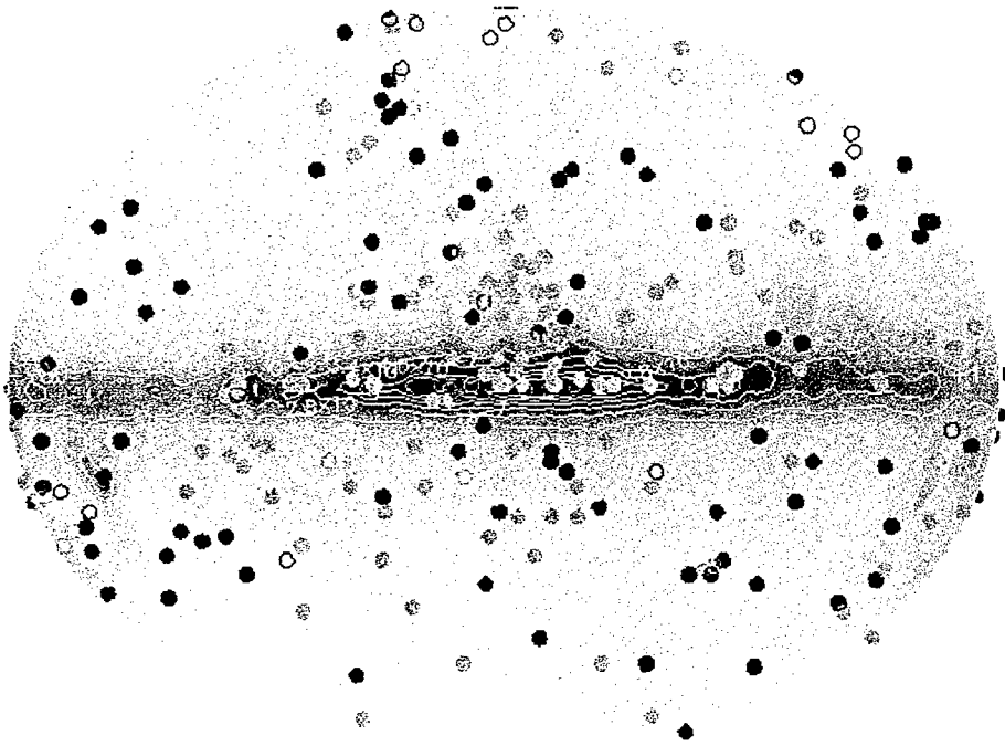
Fig. 3: A possible sky-coverage of AGILE (simulation, whole mission). The circles are EGRET sources; the filled ones will be observed by AGILE ( \text{ph}/\text{cm}^2/\text{s} @ E > 100 \text{ MeV} )
