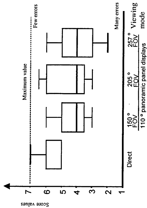
Figure I-13. Lane-Following Accuracy.
