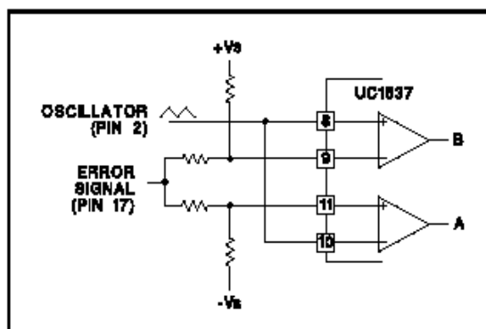
Figure 2. Comparator Biasing
