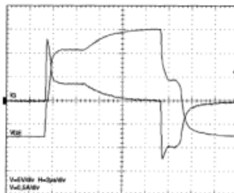
Fig.11 Output voltage ( V_{GE} ) and output current ( I_C )
