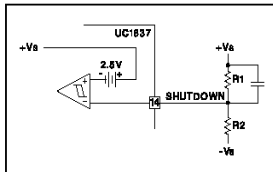
Figure 5. Delayed Start-Up
