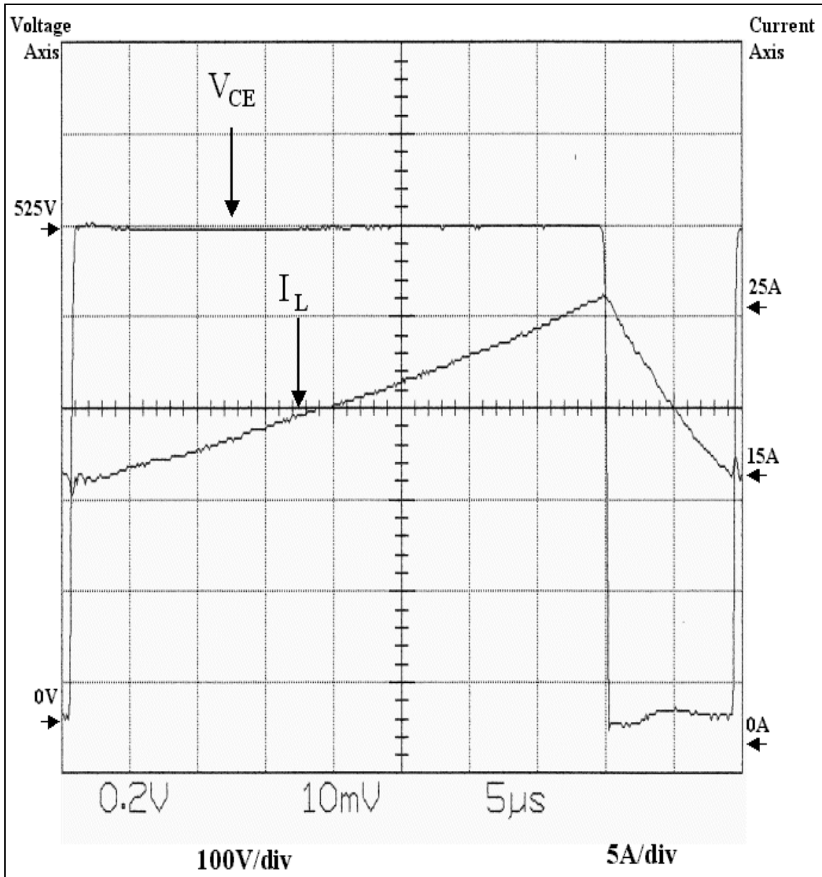
Figure 6-6, Voltage across the IGBT ( V_{CE} ) and Current through the Inductor ( I_L ) for one Switching Cycle with V_{in} = 528.2V.4 , V_{out} = 425V and R_{Load} = 19.63\Omega (measured at 20.2\Omega with zero current).
