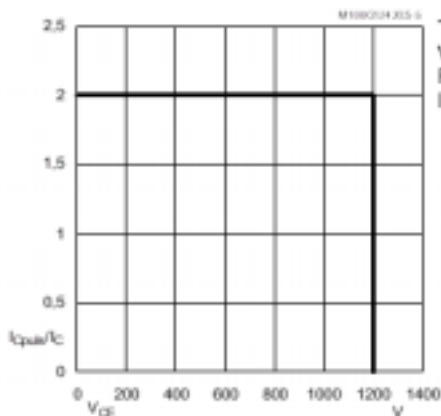
Fig. 5 Turn-off safe operating area (RBSOA)
