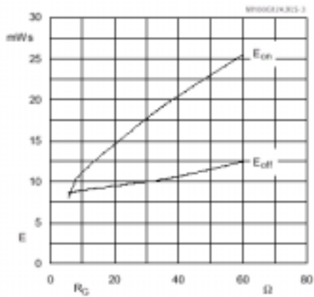
Fig. 3 Turn-on /-off energy = f(R_G)
