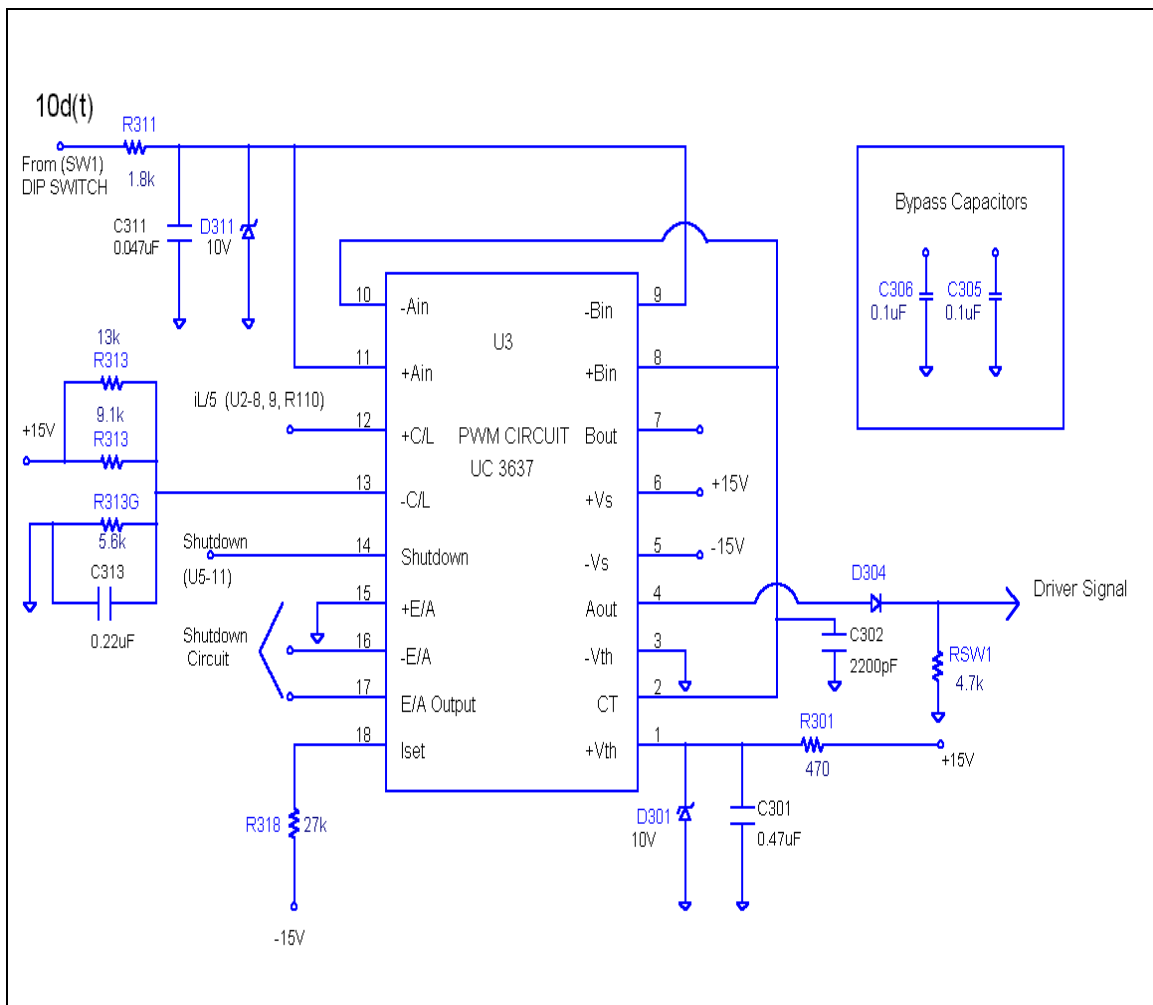
Figure 3-11, PWM Circuit Diagram.
