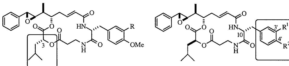
Figure 2. Structure of C3 and C10 Analogues.
