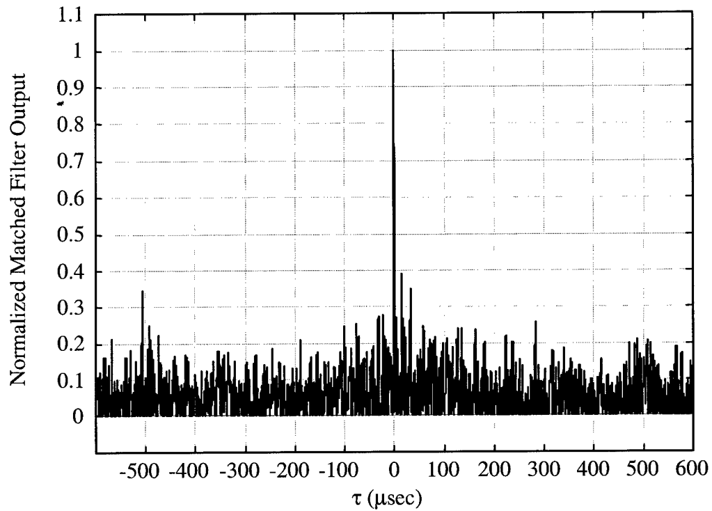
Figure 20. Post-Processed GP-3 Matched Filter Output Results for N = 2 Pulses, Gold Coded Waveform at \text{SNR} = -15.0 dB.
