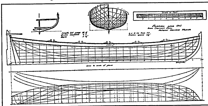
Figure 9. Hull lines of a 1700-1750 pinnace (as presented in Chappelle 1951:23).
