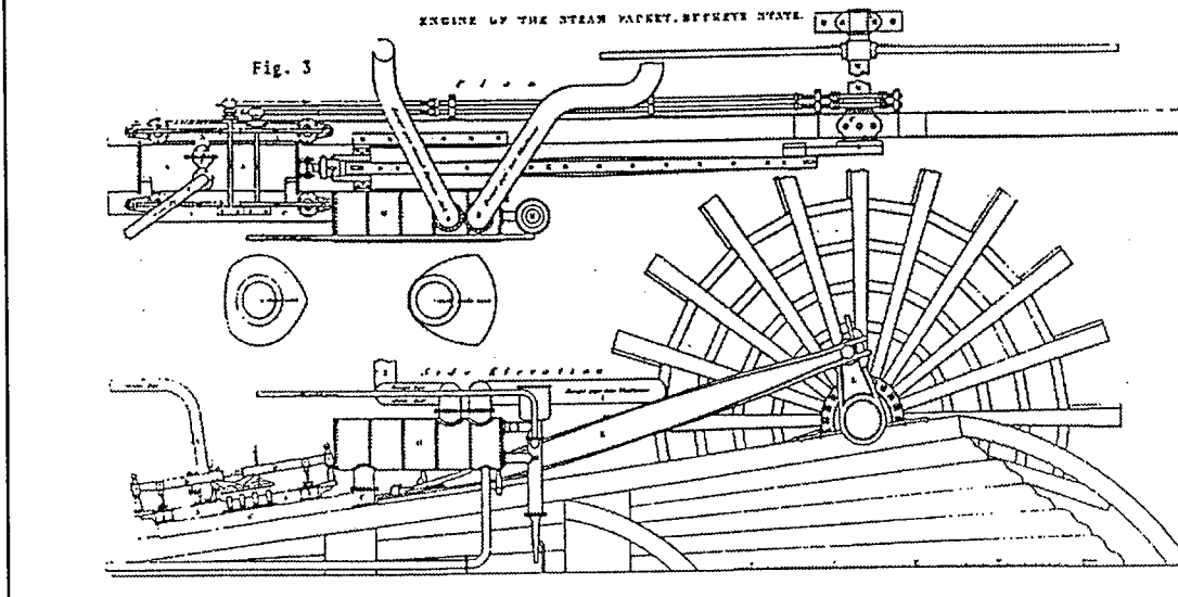
Figure 15. Illustration of an 1850s steamboat boiler and engine (as presented in Sawyer 1978:75).
