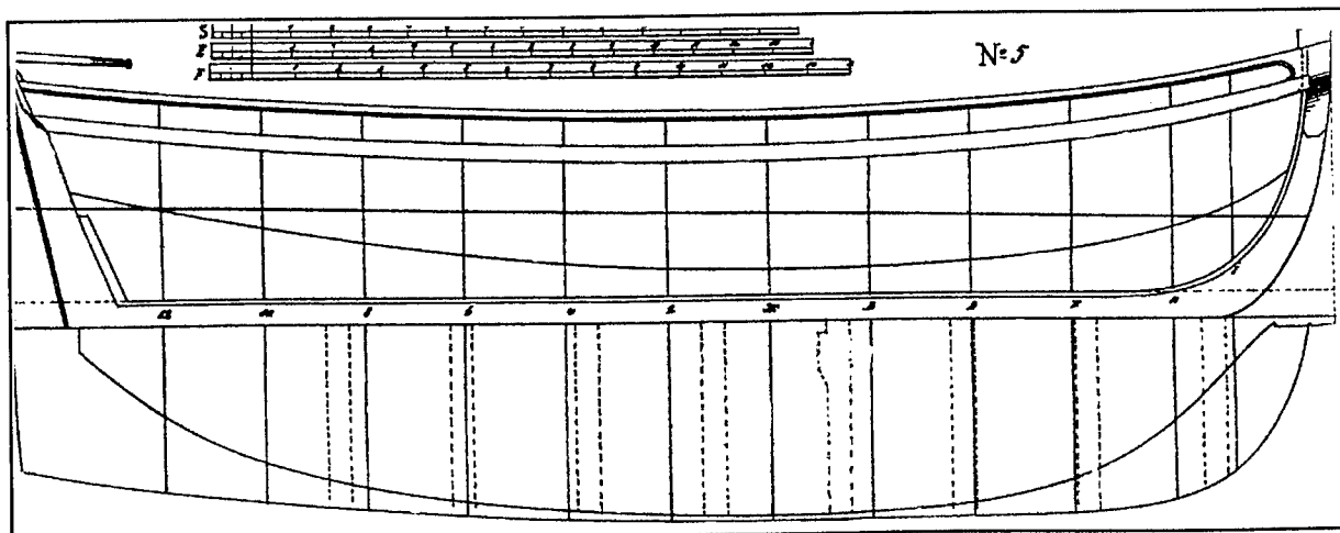
Figure 8. Hull lines of a 34-foot longboat (as presented in Chapman 1768:58).
