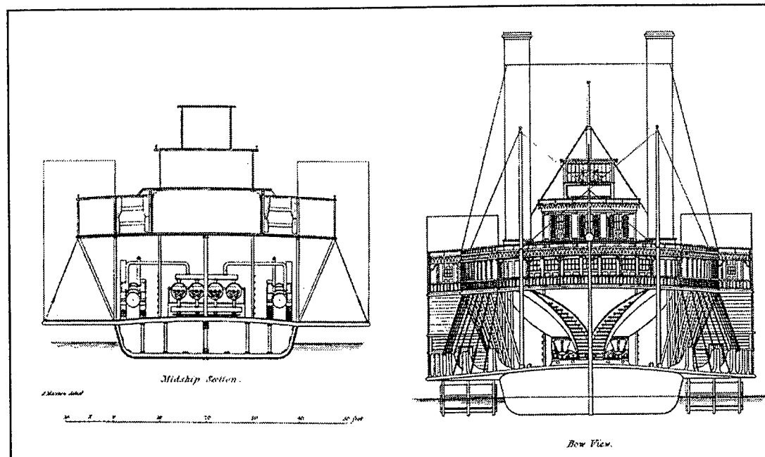
Figure 16. Midship section and bow view of a typical western rivers steamboat of the 1850s (as presented in Hunter 1949:18).
