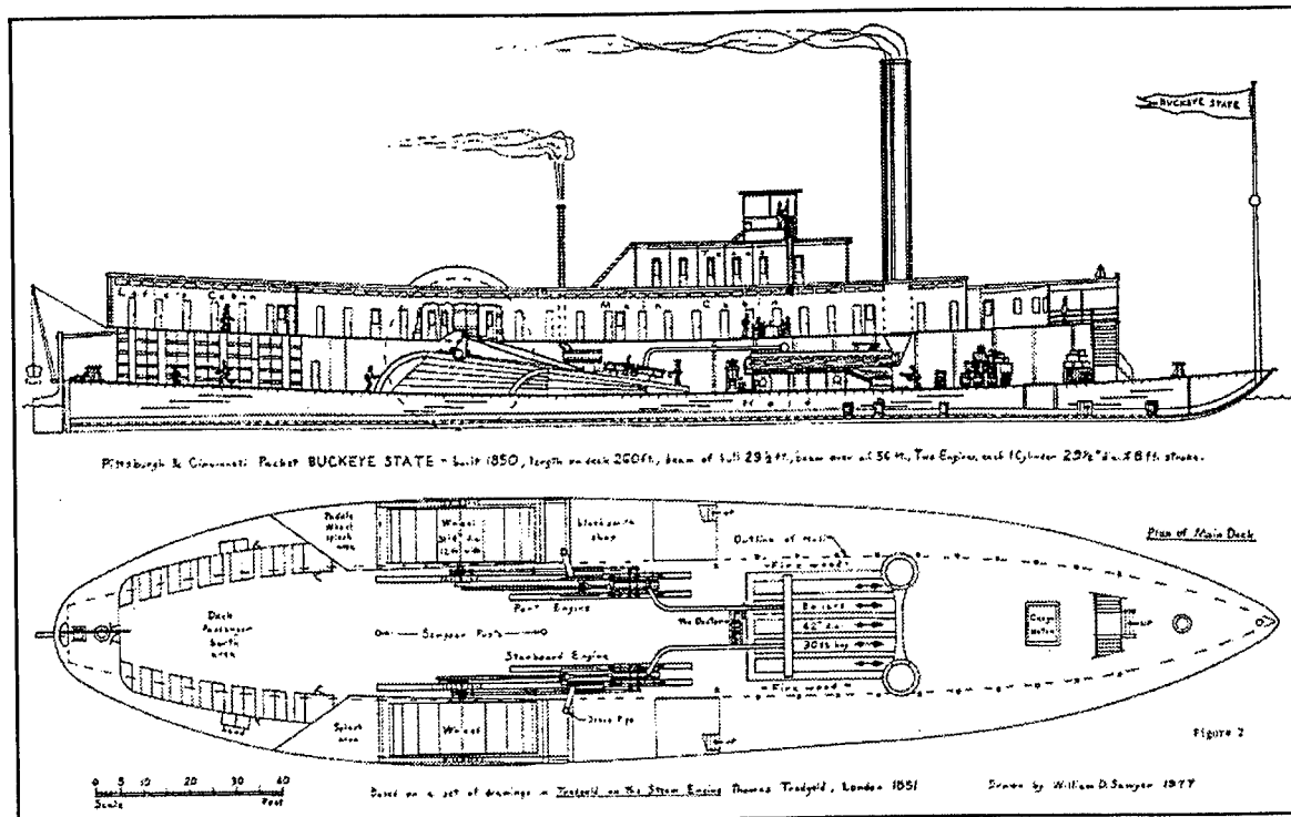
Figure 17. Plan and profile of a typical western rivers sidewheel steamboat of the 1850s (as presented in Sawyer 1978:74).
