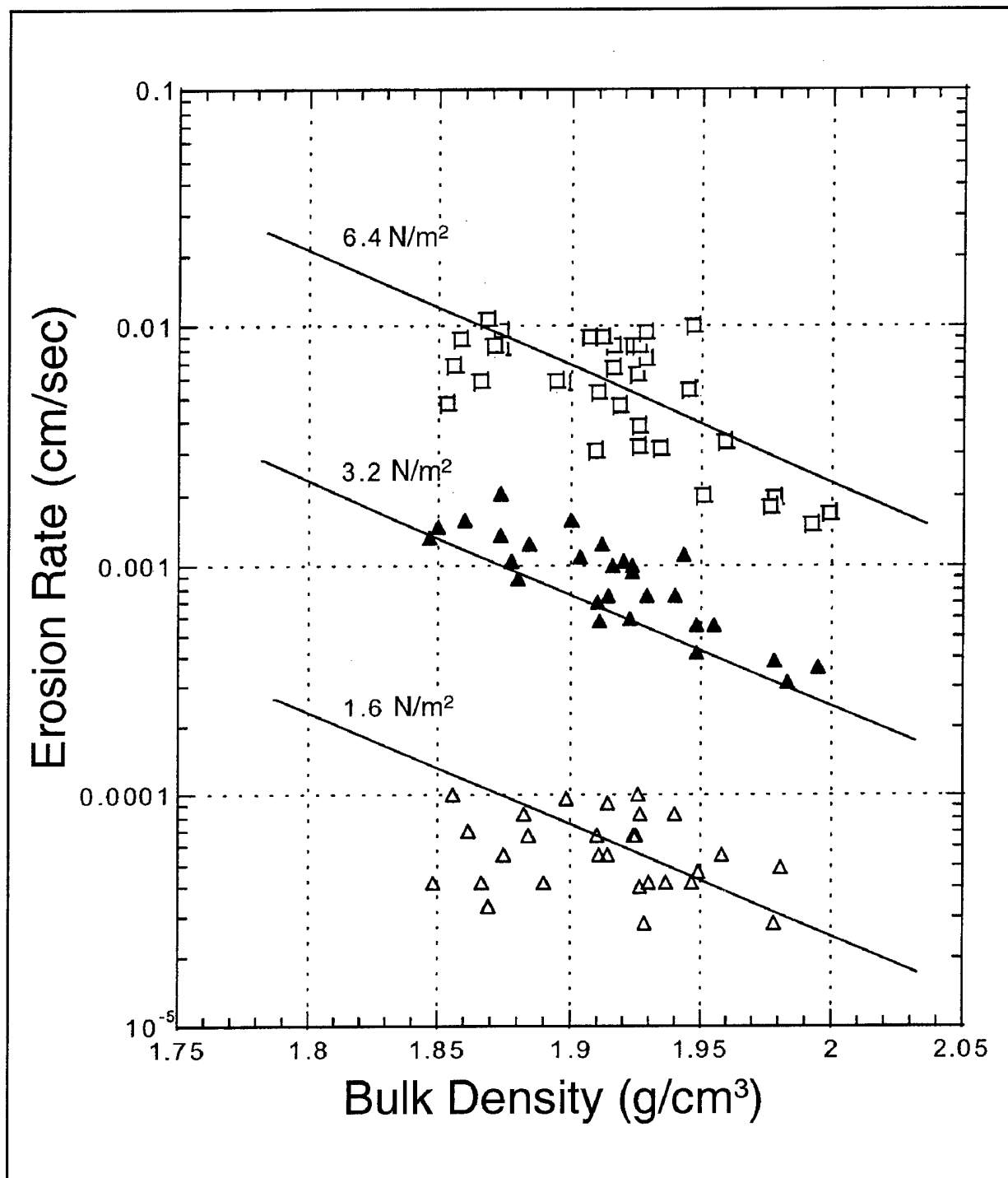
c. Erosion rates as a function of \rho^* with shear stress ( \text{N/m}^2 ) as a parameter and 1 day data eliminated
