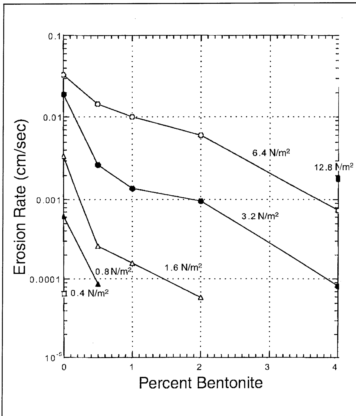
Figure 5. Erosion rates averaged for all densities as a function of percent bentonite added with shear stress ( \text{N/m}^2 ). Note the difference in the vertical scale between Figures 5a, 5b, and 5c (Sheet 1 of 3)
