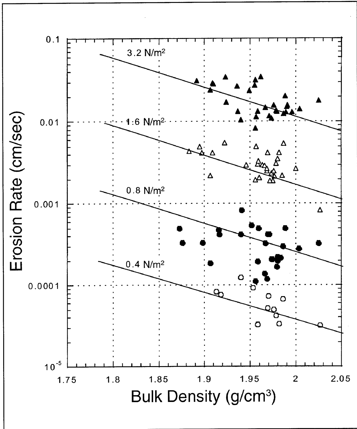
c. Erosion rates for capping material with no base sediment as a function of \rho^* with shear stress (N/m²) as a parameter
