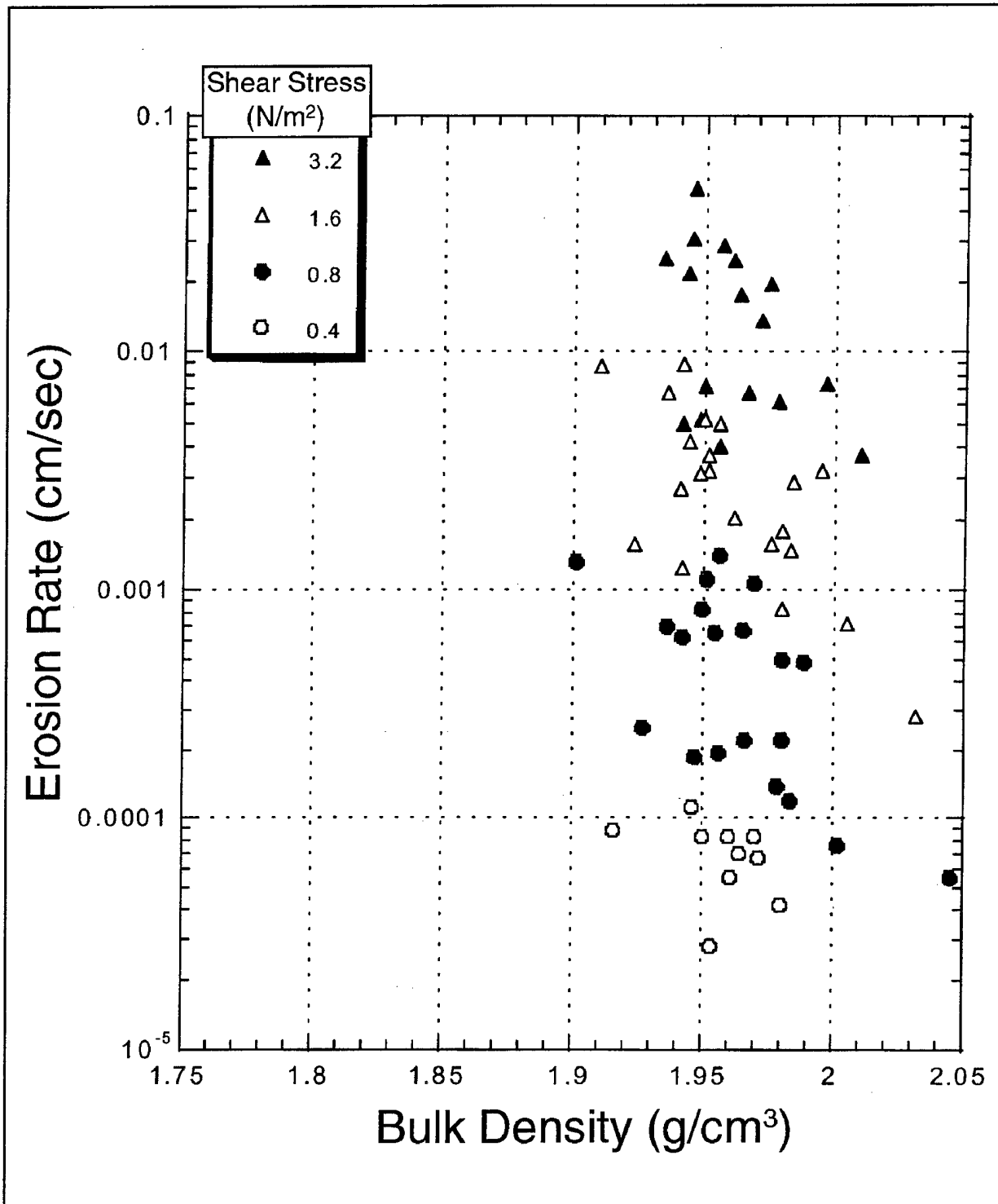
b. Erosion rates as a function of density, \rho^* , with shear stress (N/m 2 ) as a parameter. Cap over base. Inset legend indicates values for different shear stresses
