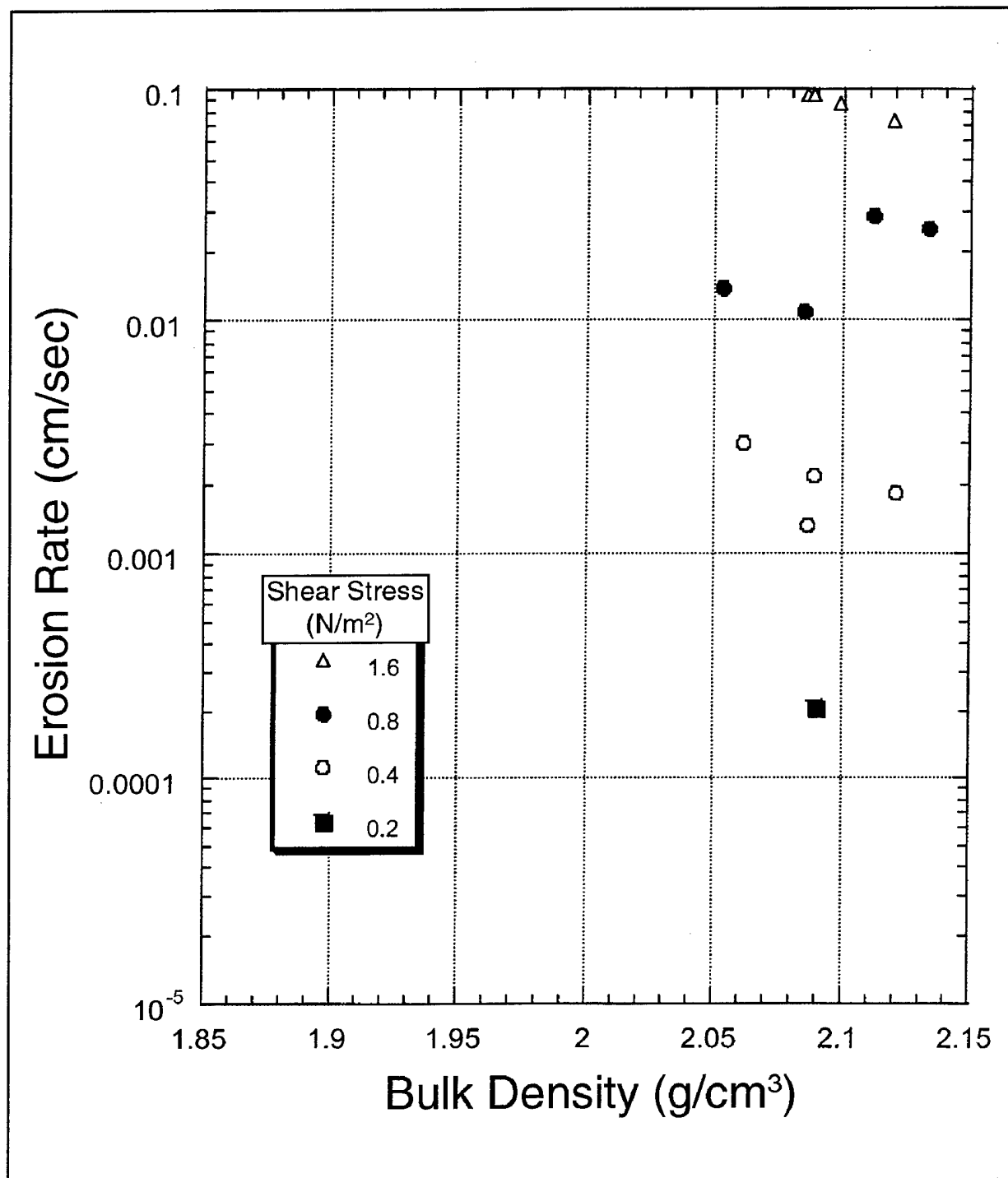
Figure 4. Sand erosion rates as a function of \rho with shear stress (N/m²) as a parameter (Sheet 1 of 4)
