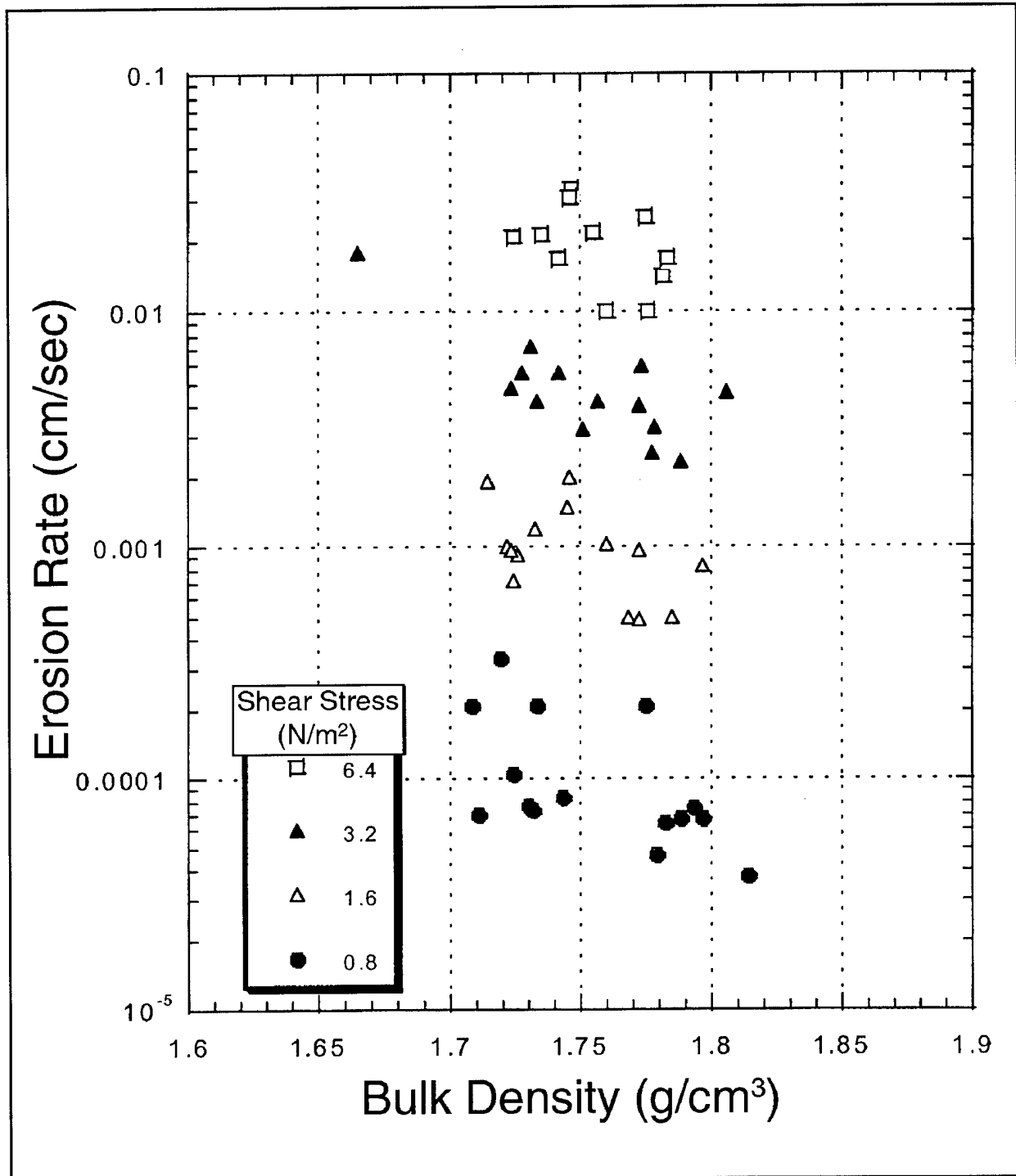
Figure 3. Erosion rates as a function of \rho^* with shear stress (N/m²) as a parameter (Continued)
