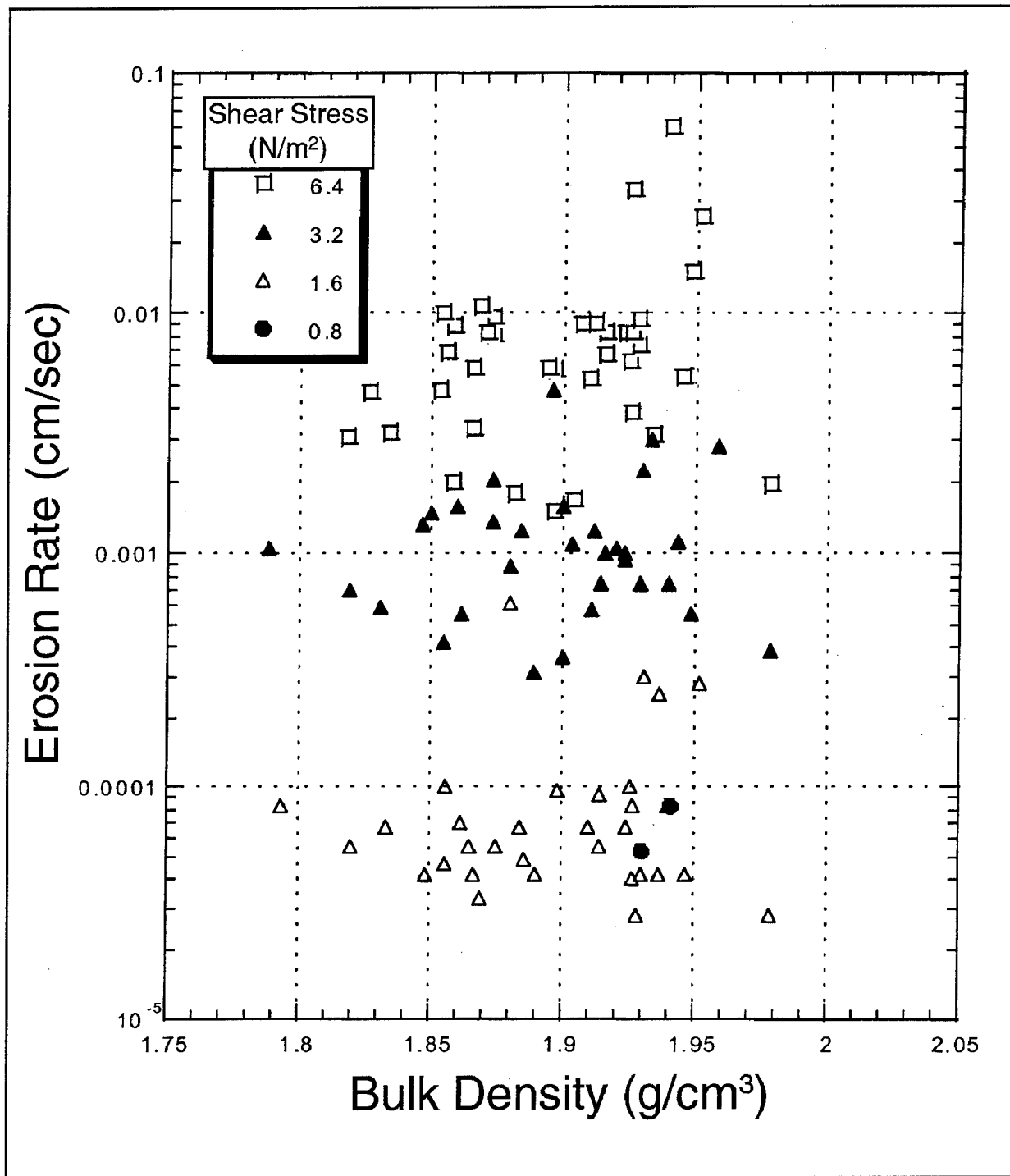
a. Erosion rates as a function of \rho with shear stress ( \text{N/m}^2 ) as a parameter. Includes all consolidation times (1-128 days)
