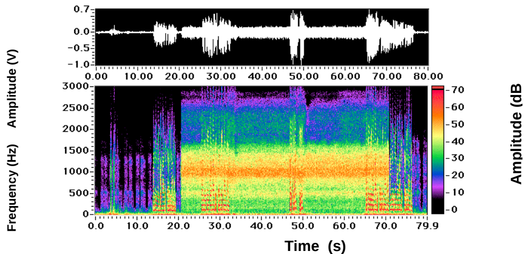
Figure 7: Gel sensor on neck detecting voice in high noise environment (105 dB C).
