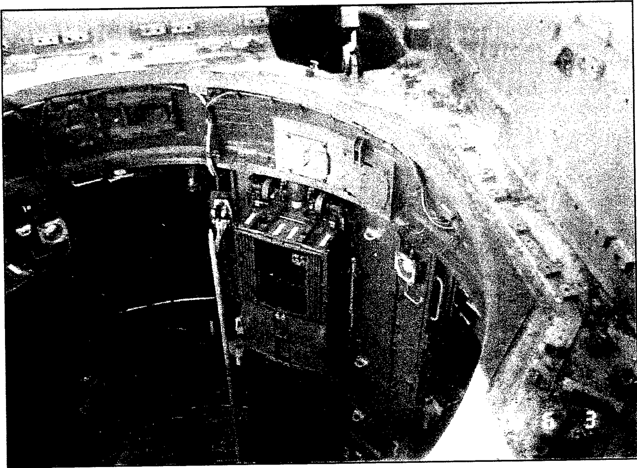
Figure 9. Detail of the silo door pocket and upper part of the silo tube, prior to demolition. The silo door is open. Note the elevator in the center. Derzhavinsk, Regiment 2, Silo 2. Courtesy of DTRA.
