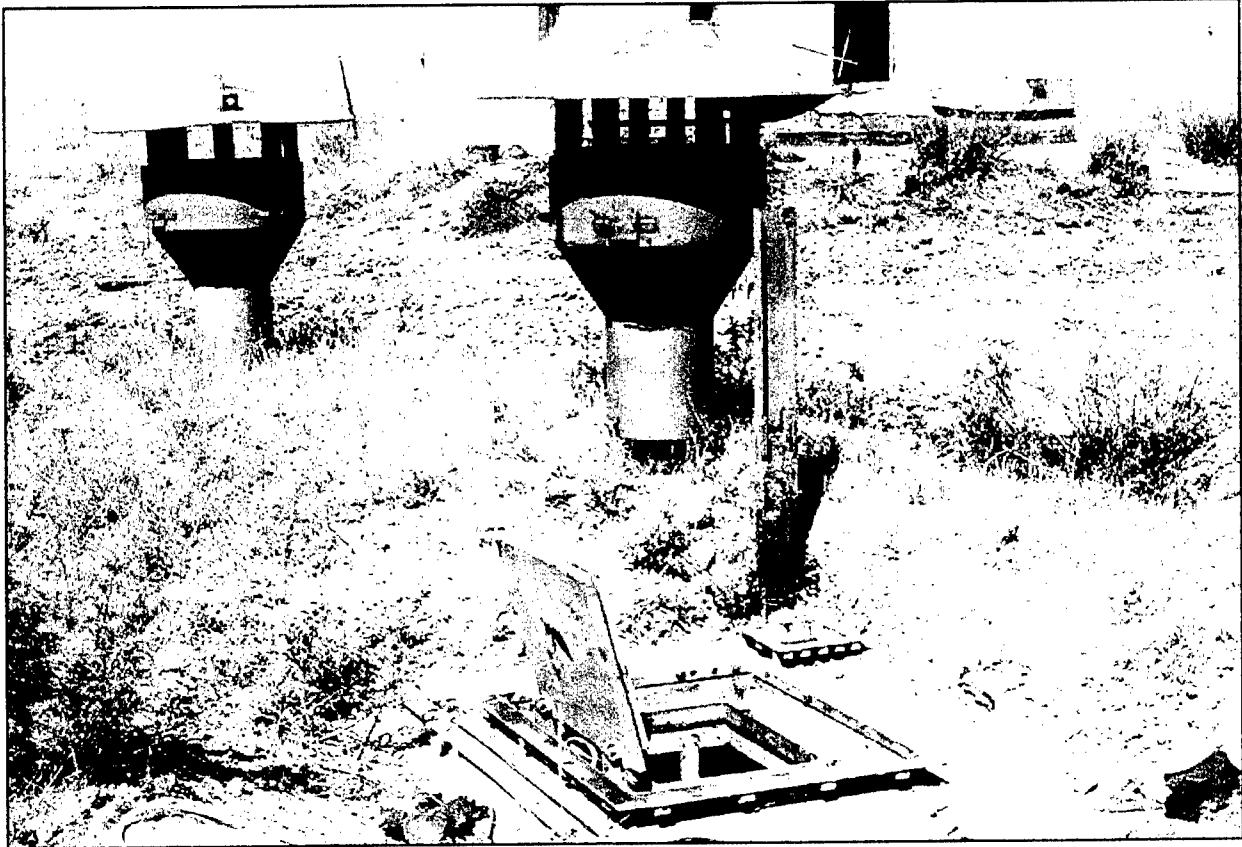
Figure 22. The ventilated underground chamber for access to the launch silo and cables. The transformer substation is in the background. Derzhavinsk, Regiment 2, Silo 4.
