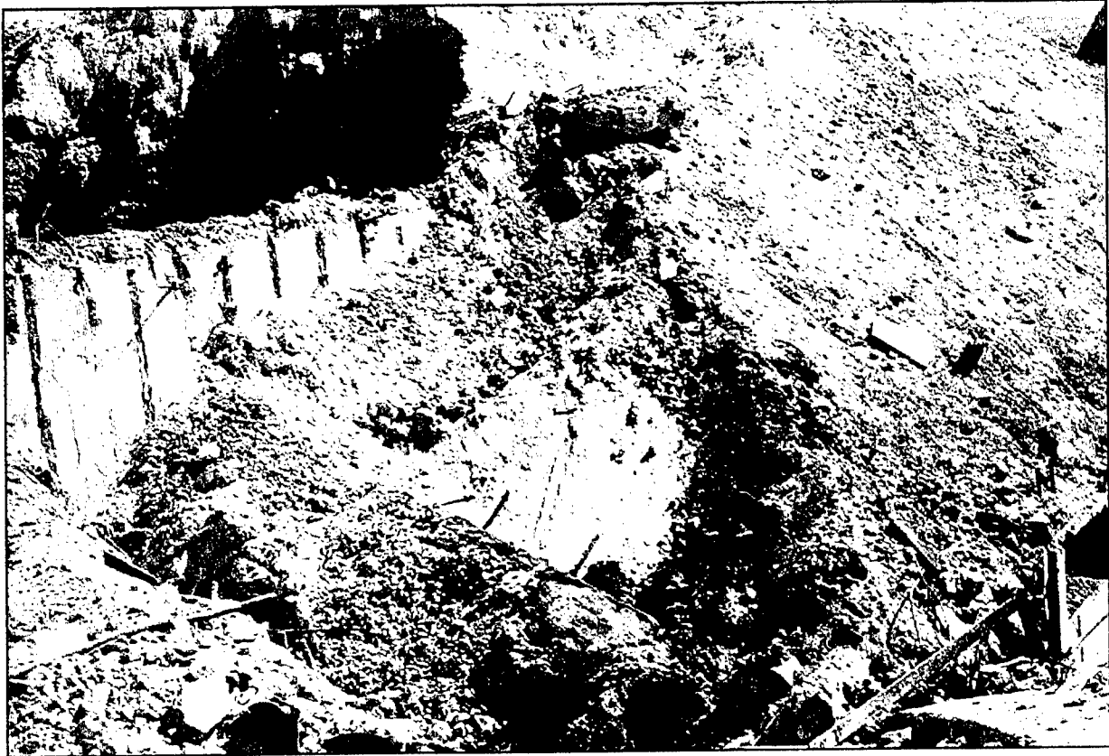
Figure 6. Poured, reinforced concrete square outer retaining wall exposed in silo crater. Derzhavinsk, Regiment 5, Silo 4.
