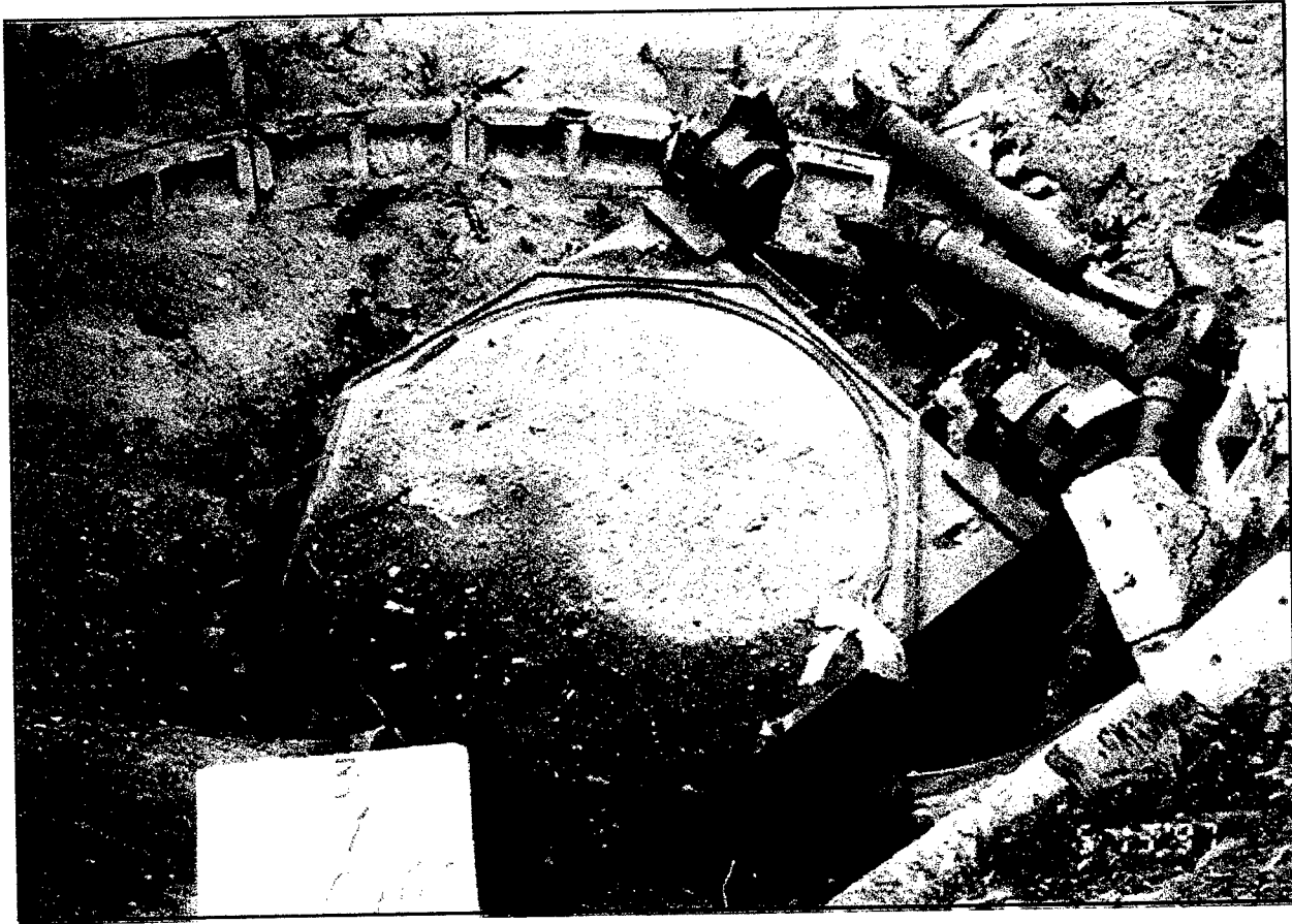
Figure 13. Hinged door for a launch silo, resting on the crater wall. Zhangiz Tobe, Regiment 3, Silo 1. Courtesy of Brown & Root/ABB SUSA.
