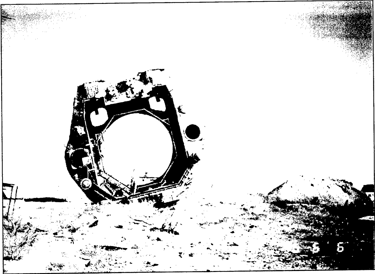
Figure10. Destroyed silo door pocket standing on end. Note the individual for scale. Probably Zhangiz Tobe. Courtesy of DTRA.
