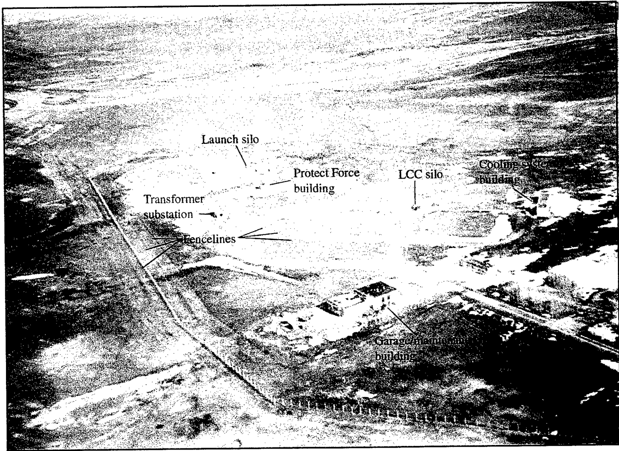
Figure 5. Helicopter overflight of a co-located LS/LCC silo site. Zhangiz Tobe. Courtesy of DTRA.
