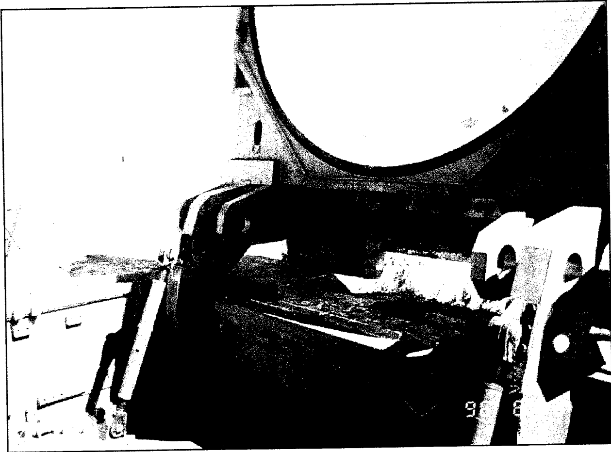
Figure 11. Detail of the top of the silo door pocket and door hinge assembly, prior to demolition. Derzhavinsk, Regiment 2, Silo 2. Courtesy of DTRA.
