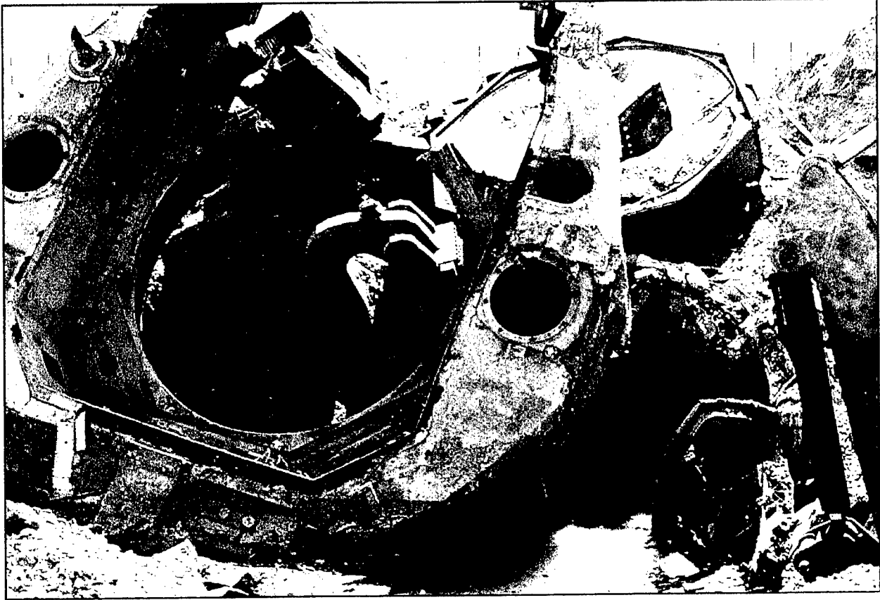
Figure 32. Up-ended silo door pocket in flooded crater. The silo door is behind the door pocket, and higher on the crater rim. Derzhavinsk, Regiment 2, Silo 4.
