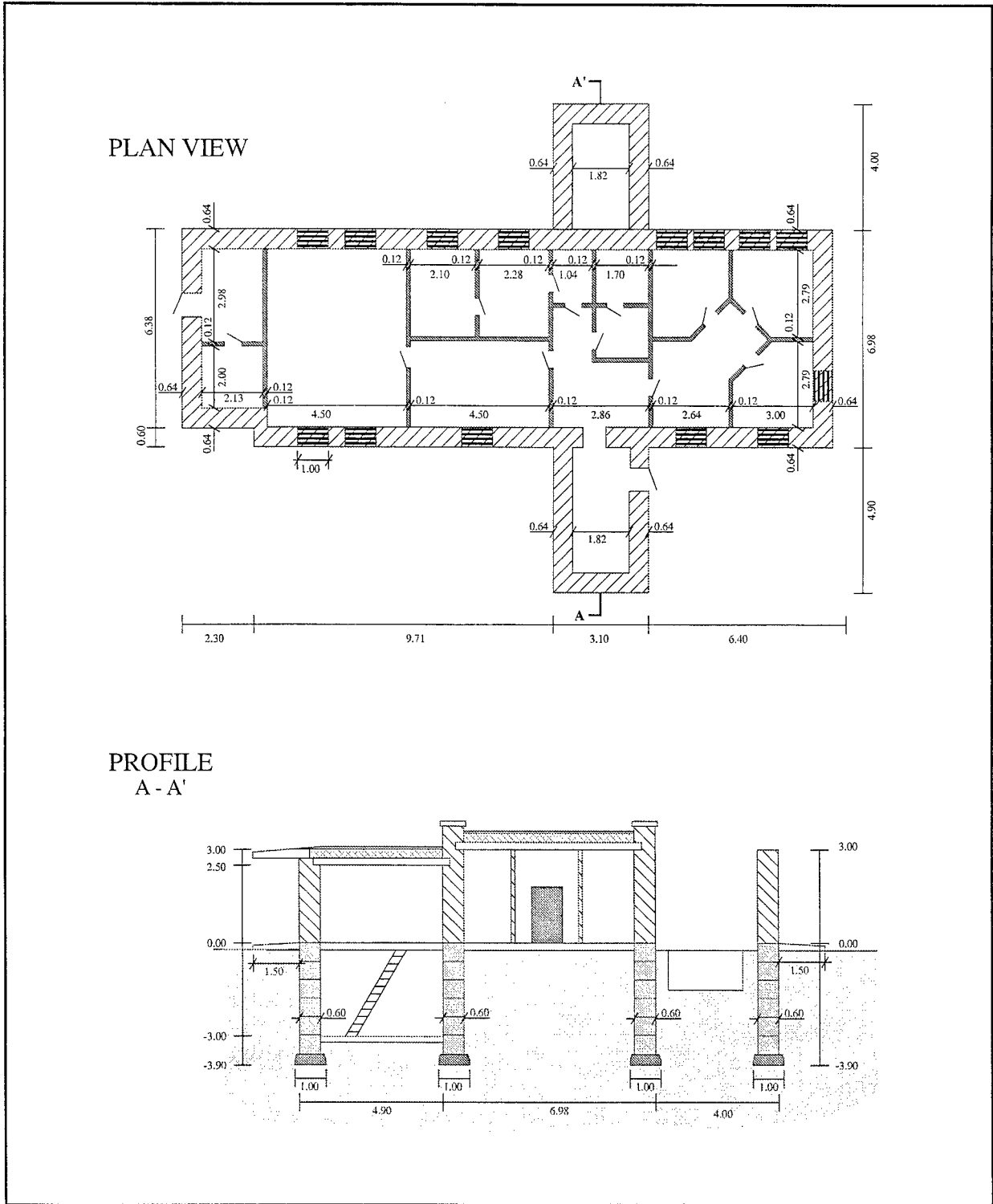
Figure 29. Plan and cross sectional drawings of the guest cottage. Derzhavinsk, Regiment 5, Silos 5/7. All measurements are in meters.
