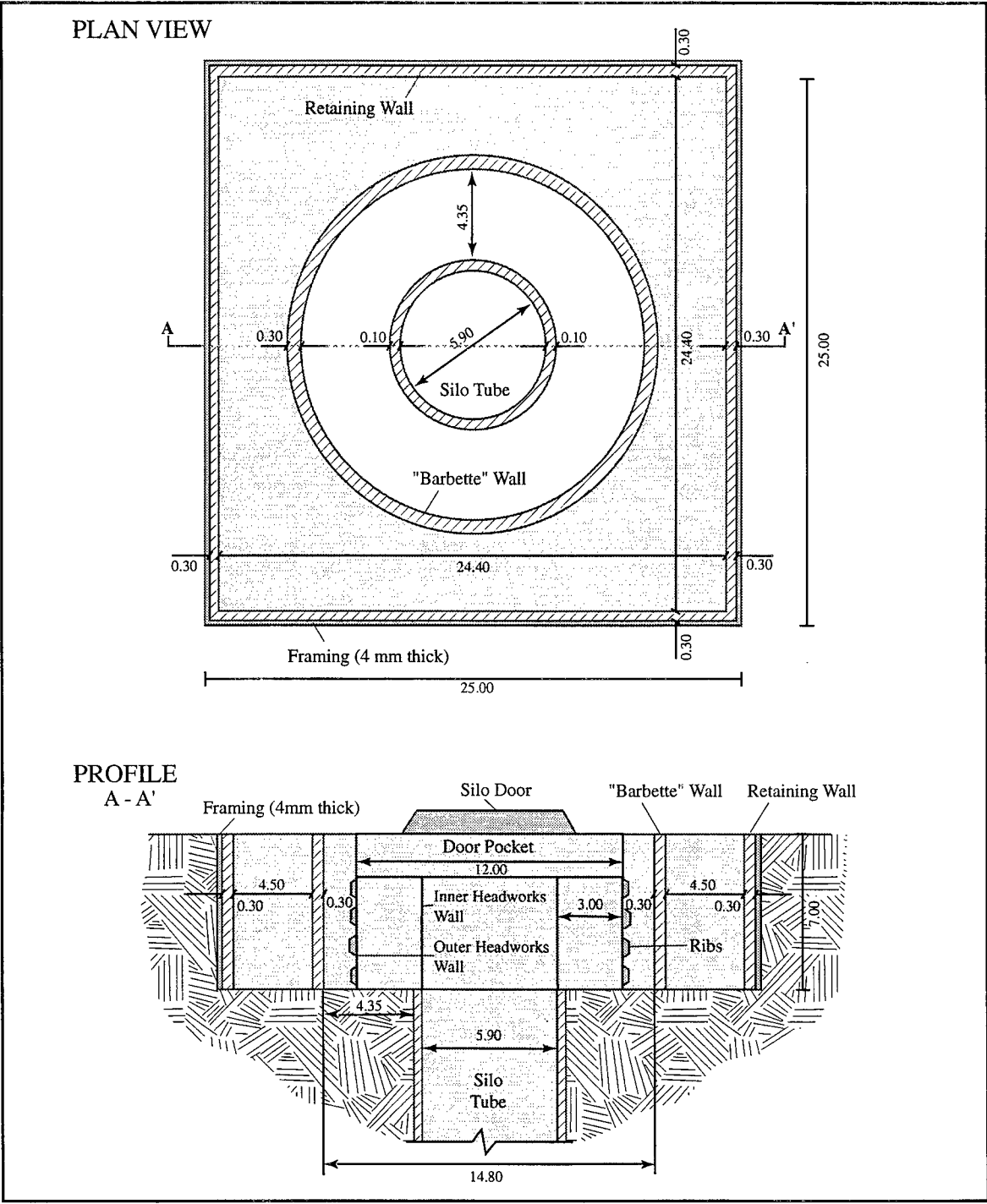
Figure 7. Plan and cross section drawings of the outer retaining wall, the inner "barbette" sectional wall, and the silo headworks area. The configuration and dimensions of the silo door, door pocket, and inner and outer headworks walls are estimated from the site photography. Derzhavinsk, Regiment 2, Silo 3. All measurements are in meters.
