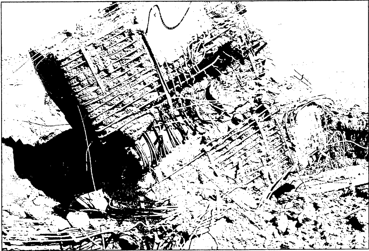
Figure 44. The bottom of the heavily reinforced concrete foundation for the dish antenna located near the launch silo. The base is 6.8 to 8.8 meters across, and 4 meters thick. A cable conduit is seen in the center. Derzhavinsk, Regiment 5, Silo 4.
