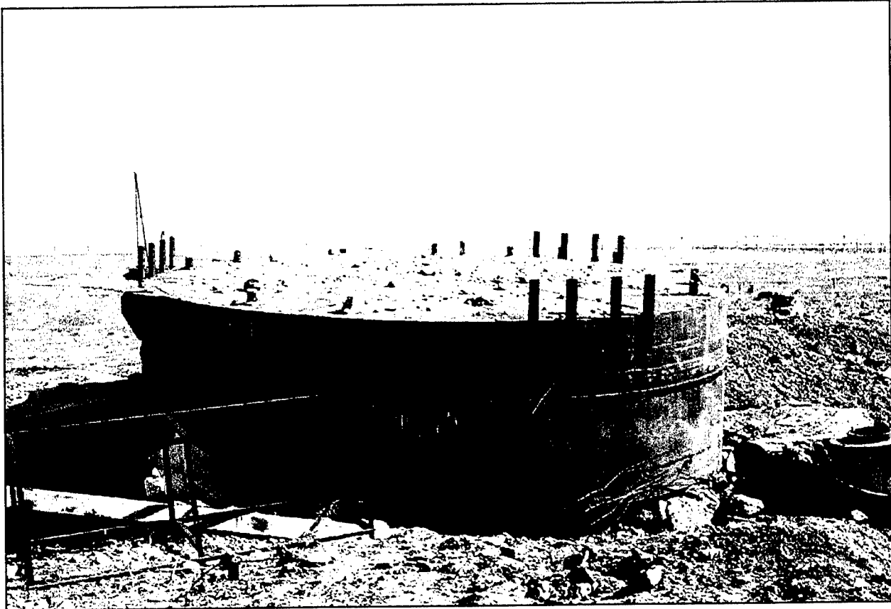
Figure 14. Round silo door for the Launch Control Center (LCC) silo. Note the difference between this door and the door for a launch silo (compare to Figure 12). Derzhavinsk, Regiment 2, Silo 7.
