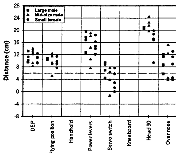
Figure 14. Measurements of clearance/contact between right-side forward airbag and subjects' NVGs. Distances greater than 0 cm indicate clearance. Distances less than or equal to 0 cm indicate contact.
