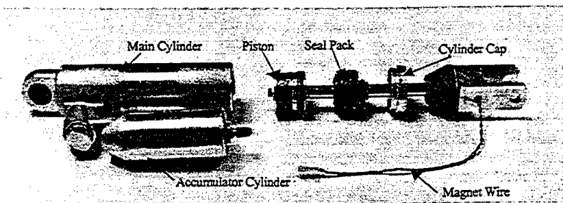
Figure 2. Components of the UNR MRF retrofit damper.
