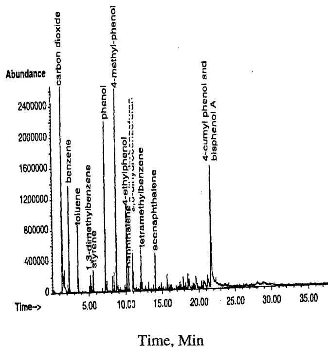
FIGURE C-6. PY-GC MS ANALYSIS OF BPA-BASED POLYCARBONATE
