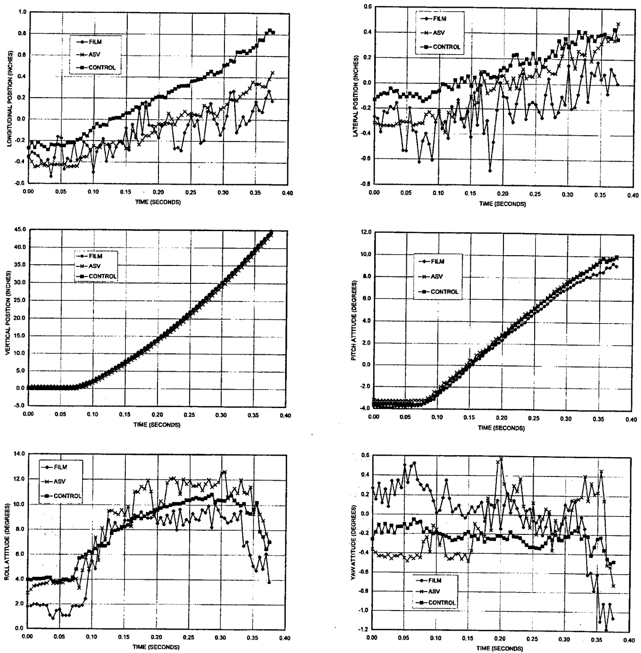
Figure 10. Sample ASV, Film and Control 6-DOF Comparison (Ground Test)
