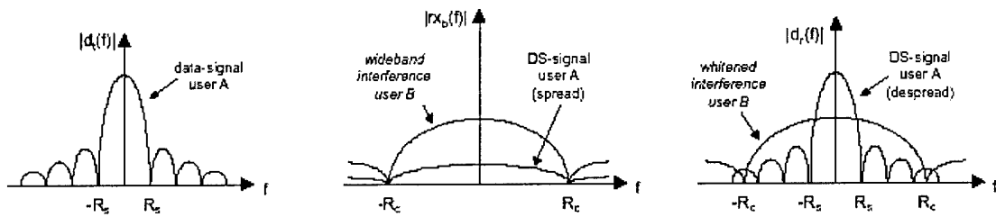
Figure 11. Effect of wideband interference on a DSSS signal [9].
