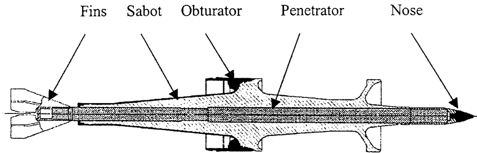
Figure 1. Schematic of the M829A1 Projectile.
