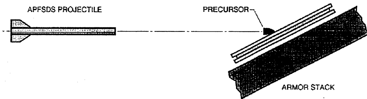
Figure 7. Tandem-Rod Concept From Menna and King (1993).
