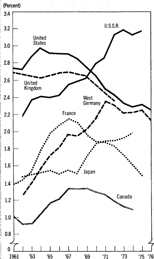
National Expenditures for performance of R&D 1 as a percent of Gross National Product (GNP) by country, 1961-76
