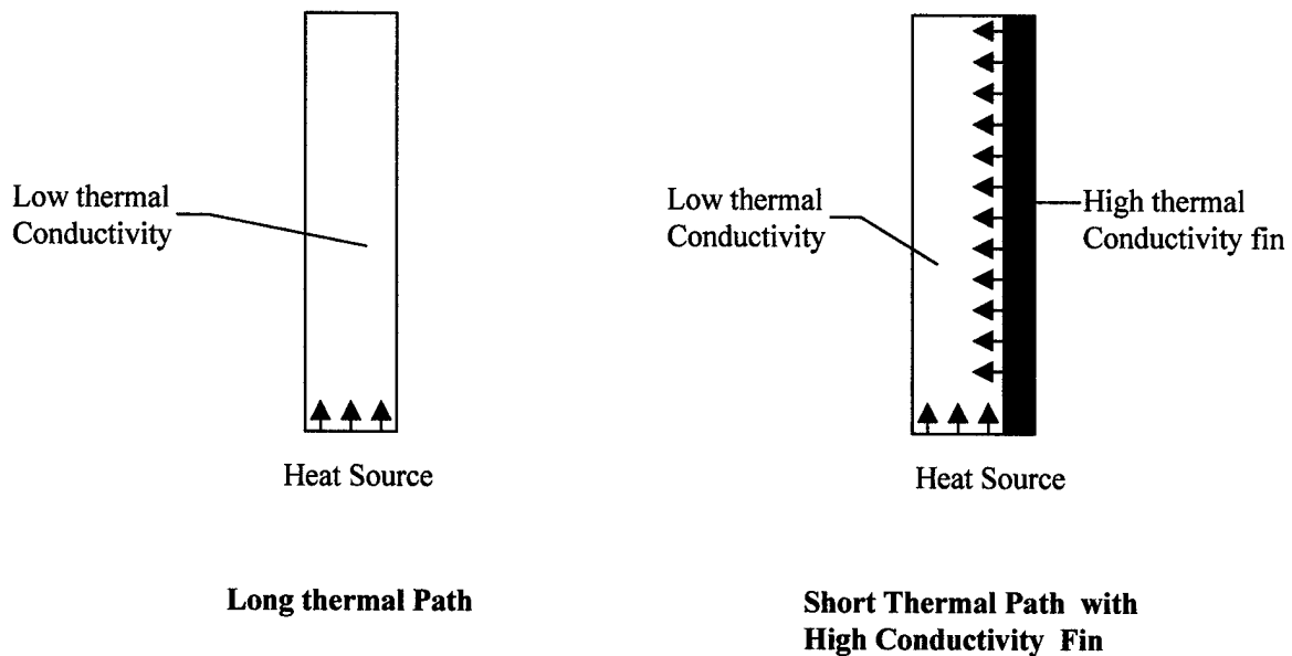
Figure 2.16 The Use of High Conductivity Fins to Provide a Shorter Thermal Path Through the Lower Conductivity PCM
