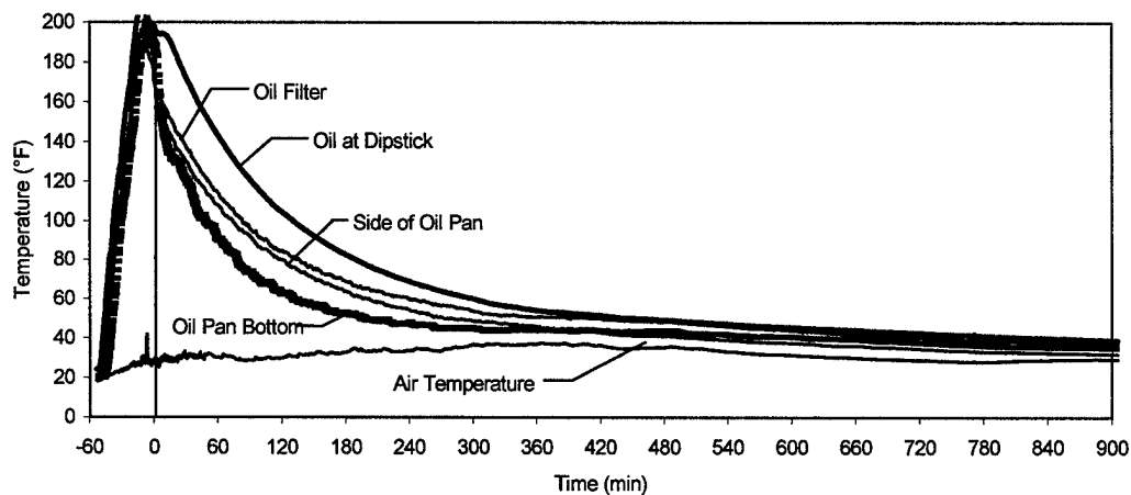
Figure 4.17 Oil System Temperatures Measured During Cool-Down Test on February 14,1999
