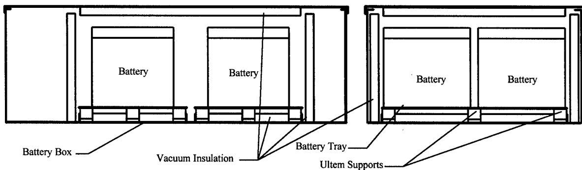
Figure 2.36 Simplified Assembly Drawing of the Insulated Battery Box
