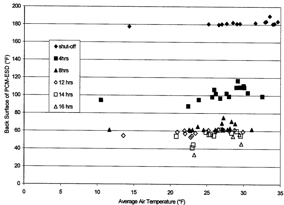
Figure 4.37 Temperature Measured on the Backside of ESD#1 vs. the Average Air Temperature after Engine Shut-off
