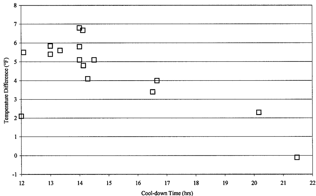
Figure 4.44 Difference Between the Oil Temperature at the Bottom and Top of the Oil Pan for PCM-ESD Cases
